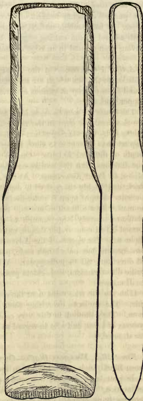
COPPER CHISEL. Full size.—Length 7\frac{1}{4} in.; breadth 1\frac{1}{2} in.; thickness \frac{3}{8} in. Minnesota Mine. View edge-wise.
