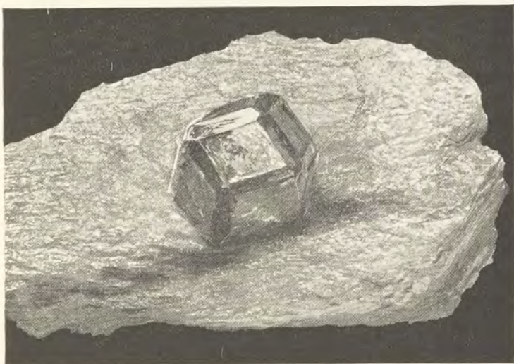
CRYSTAL OF GARNET IN MATRIX (ACTUAL SIZE).
