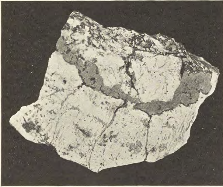
TURQUOISE IN THE FORM OF A VEIN.
