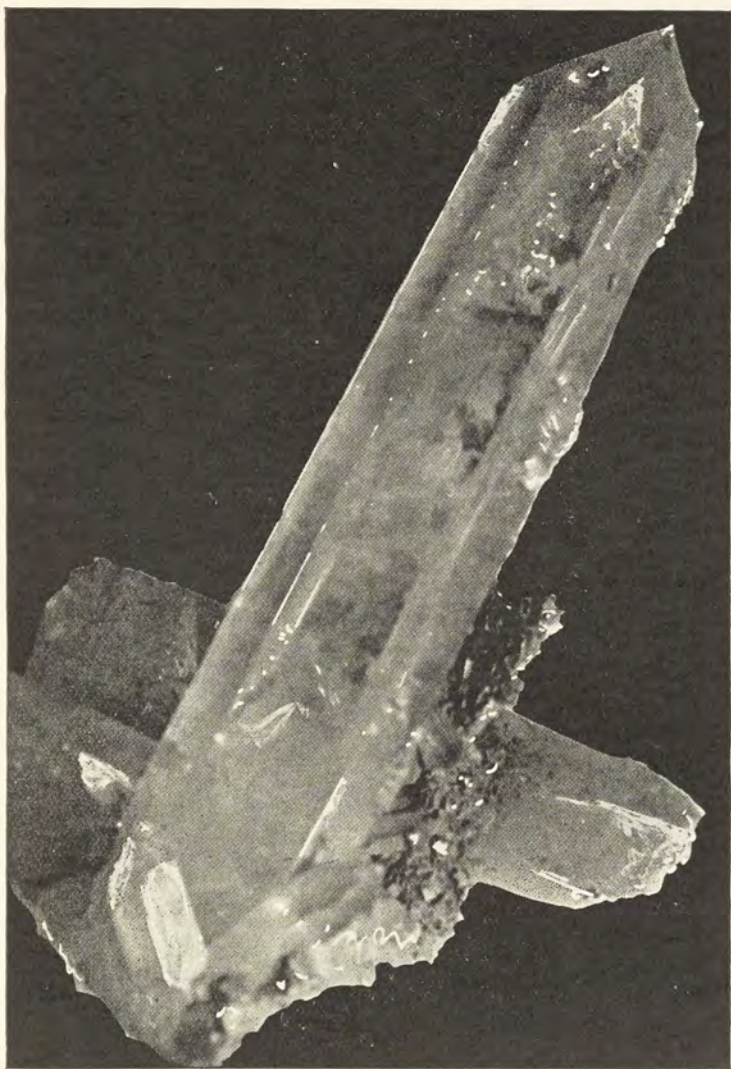
CRYSTALS OF ROCK CRYSTAL (ACTUAL SIZE).
