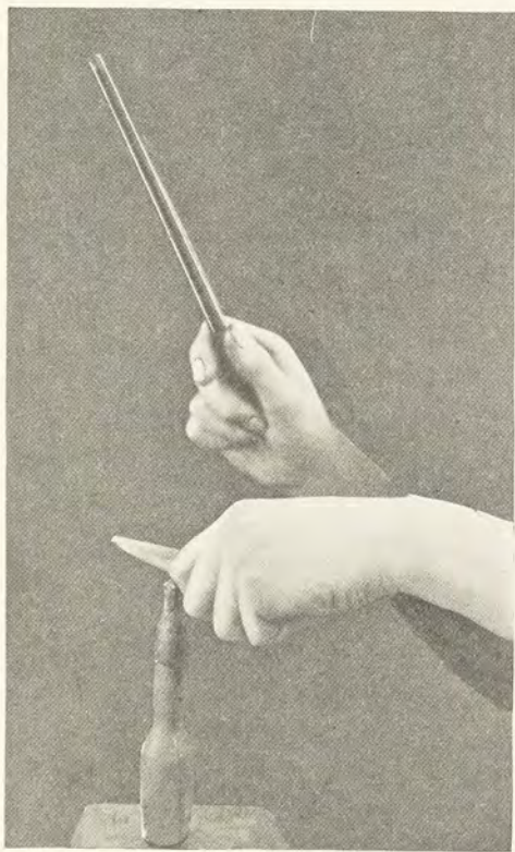
DIAMOND CLEAVING.
