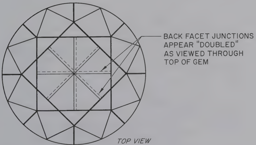
FIG. 7 A faceted zircon gem showing how the back facets appear doubled due to double-refraction.
