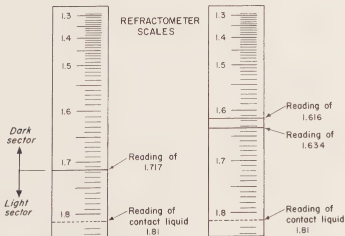
THE REFRACTOMETER
