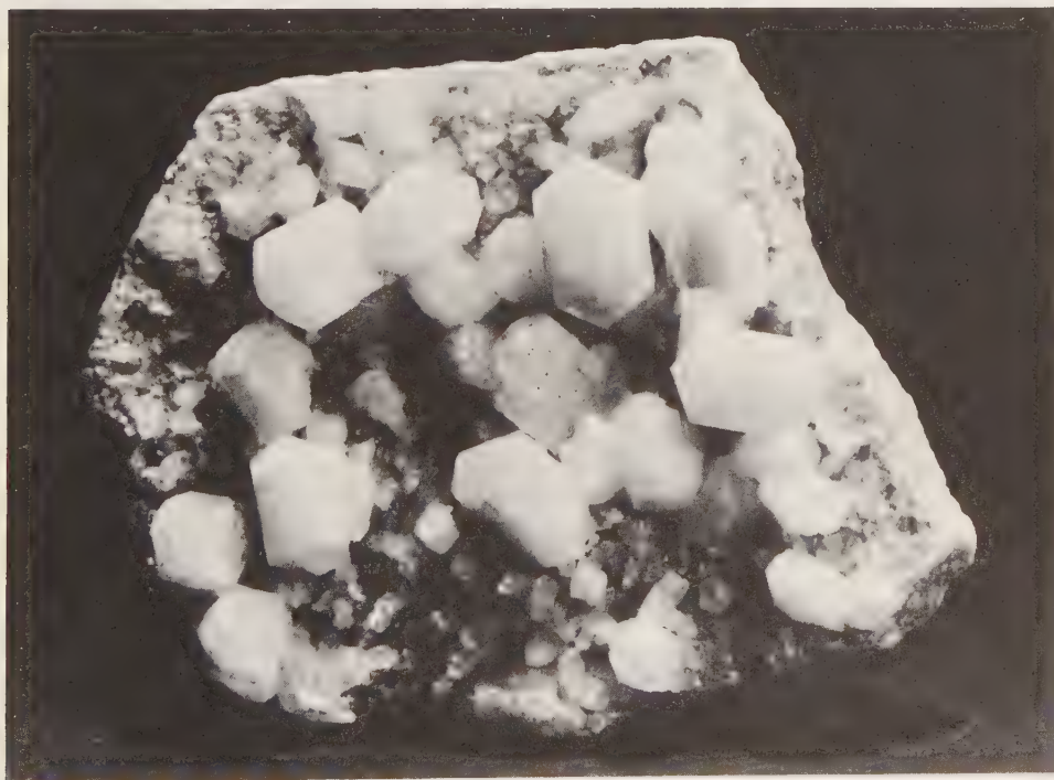
FIG. 258. Twinned harmotome crystals on matrix from Bellesgrove Mine, Strontian, Argyllshire, Scotland. Size 2\frac{1}{2} " by 1\frac{3}{4} ". The boat-shaped faces are b[010] , the blunt wedges are formed by pairs of m[110] faces.
