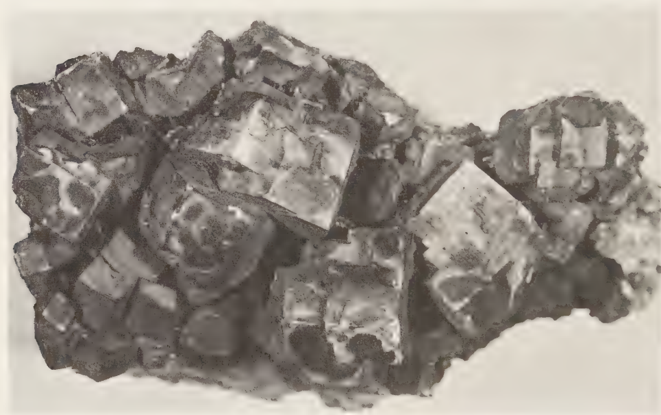
FIG. 226. Pyromorphite crystals from Beresovsk, Ural Mountains, U.S.S.R. These unusually large crystals are about \frac{3}{4} " in diameter. Photo courtesy Schortmann's Minerals, Easthampton, Massachusetts.
