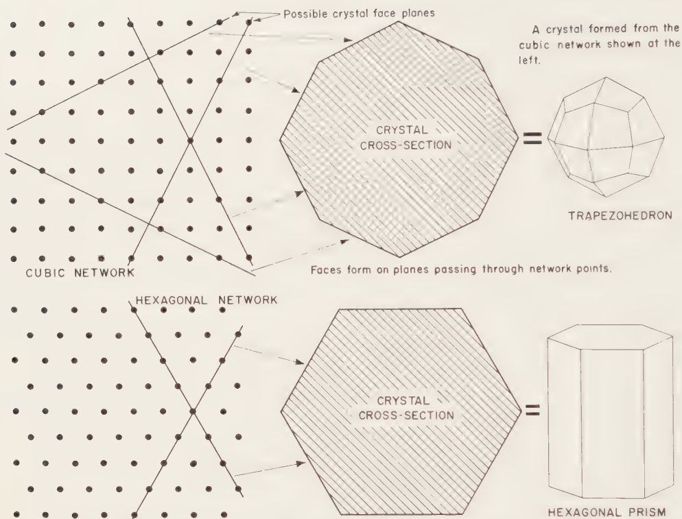
NETWORKS OF POINTS IN CRYSTALS RELATED TO CRYSTAL FACES
