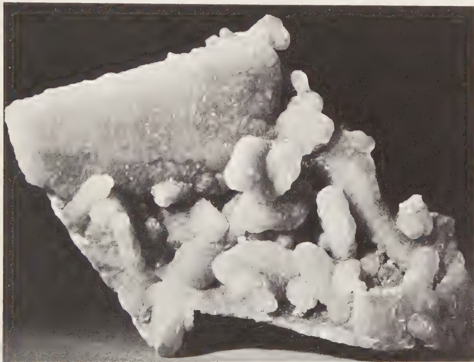
FIG. 324. Prehnite crusts originally coating anhydrite crystals. The latter dissolved after formation of prehnite, leaving behind cavities corresponding to their shapes. The large flat area at the upper left of the specimen was once a spray of slightly divergent anhydrite crystals. Size 7" by 4½". Prospect Park, Paterson, Passaic County, New Jersey.
