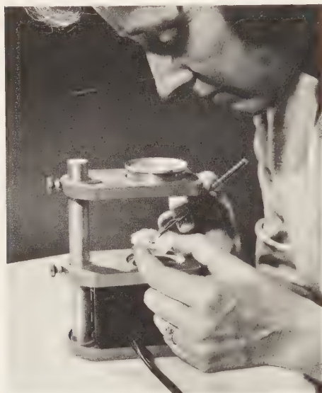
FIG. 101. Testing a thin cleavage flake of mica for a biaxial figure between the crossed polaroids of the Gemological Institute of America's polariscope. Light is provided from underneath by a small microscope substage lamp. The glass stirring rod ball-tip acts as a powerful but easily maneuvered magnifying glass to enlarge axial figures to the point where they can be clearly seen.
