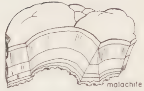
BOTRYOIDAL, MAMMILLARY
