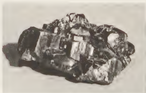
FIG. 141. Bournonite crystals in "cogwheel" twins from Wheal Boys, Endellion, Cornwall, England. Size 1\frac{1}{2} " by 1\frac{1}{4} ".
