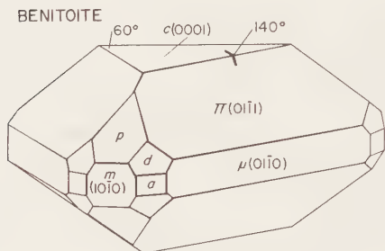
PINACOID c , FIRST ORDER PRISM m , SECOND ORDER PRISM a/11\bar{2}0 , FIRST ORDER DIPYRAMID \rho/10\bar{1}1 , SECOND ORDER DIPYRAMID d/22\bar{4}1 , THIRD ORDER PRISM \mu , THIRD ORDER DIPYRAMID \pi .
