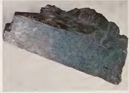
Hornblende
