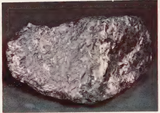
Graphite
