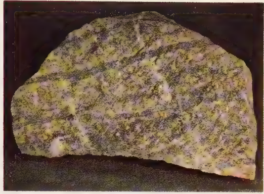
Serpentine
