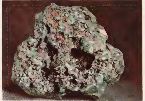
Malachite
