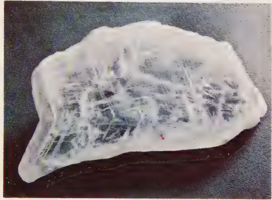
Selenite (Gypsum)
