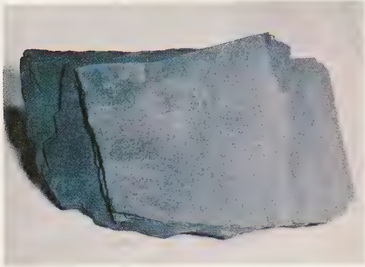
Gray Slate
