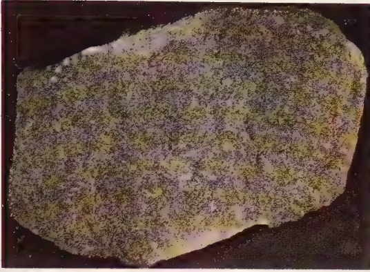
Olivine
