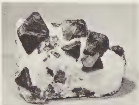
FIG. 167. Franklinite octahedrons in calcite matrix from Franklin, Sussex County, New Jersey. Size 3" by 2".
