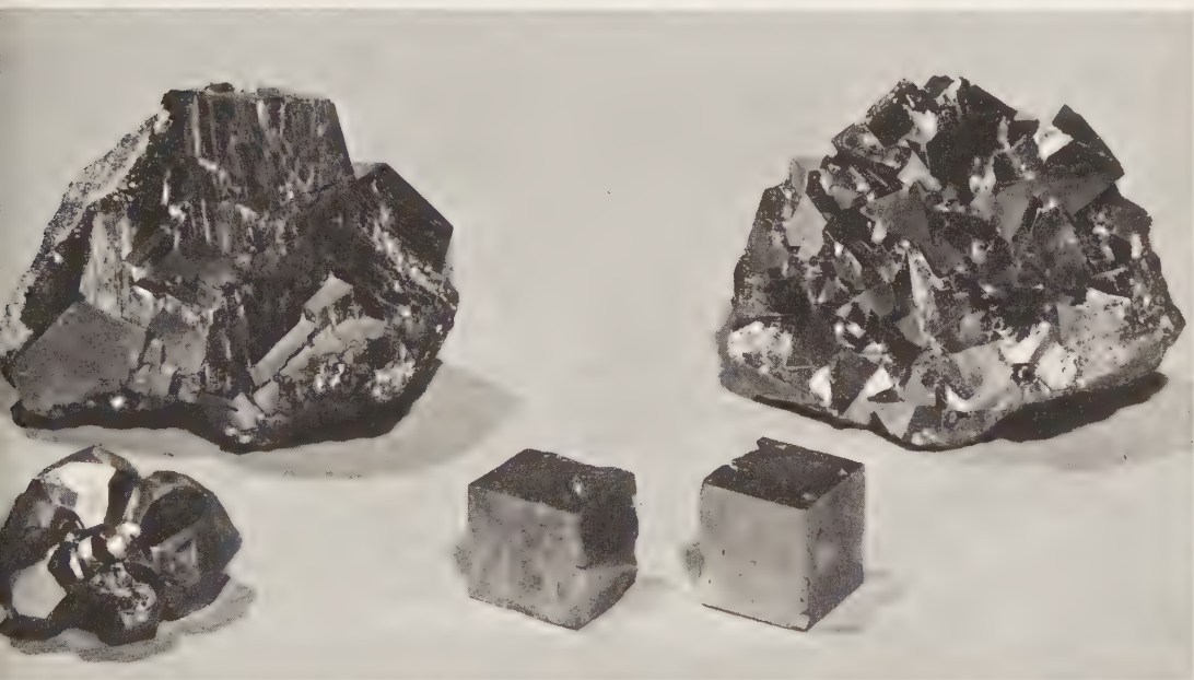
FIG. 129. Pyrite. Top left: modified pyritohedrons on matrix of specular hematite. Size 3½" by 3". Rio Marina, Elba, Italy. Top right: sharp octahedral crystals on massive pyrite from Morococha, Peru. Size 3½" by 2½". Bottom left: highly modified crystals in a cluster from Elba. Forms include cube, pyritohedron, octahedron and diploid. Size 1¾". Bottom center: simple cubes from Elba.
