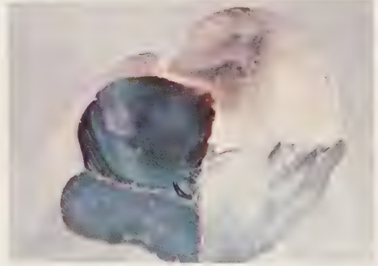
Flint Concretion in Chalk
