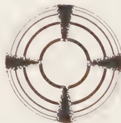
Normal uniaxial figure showing colored rings and black cross.
