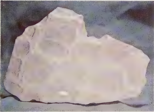
Mudcracks in Sandstone
