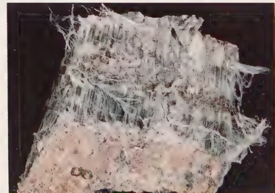
Chrysotile Asbestos
