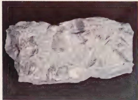
Shell Limestone
