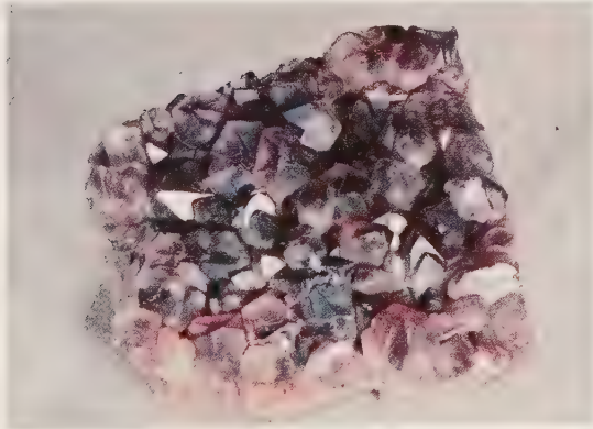
Amethyst
