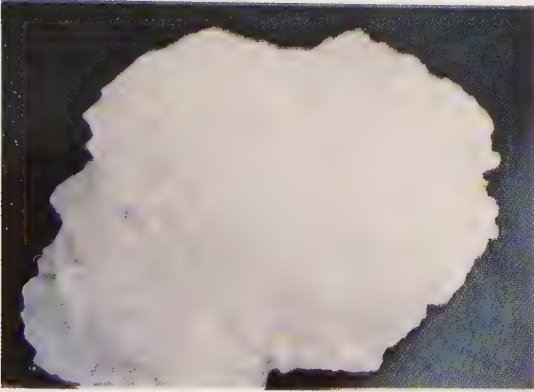
Rock Salt
