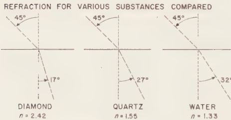
REFRACTIVE INDEX
