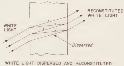
DISPERSION
