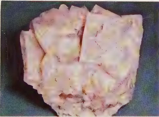
Fluorite
