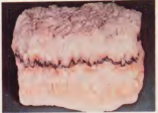
Banded Travertine
