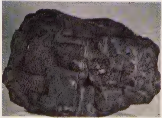
Bituminous Coal
