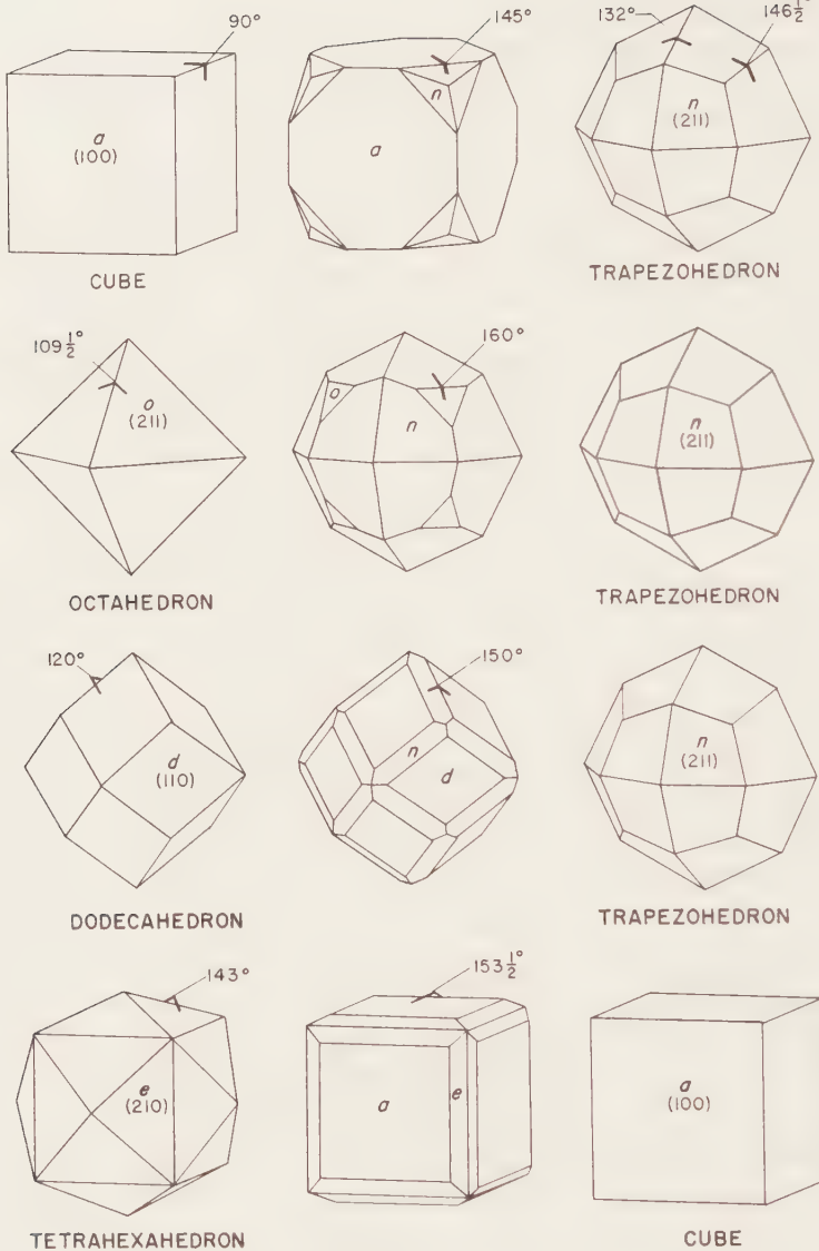
ISOMETRIC FORMS AND COMBINATIONS
