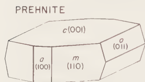
PRISMS m, a , PINACOIDS a, c .
