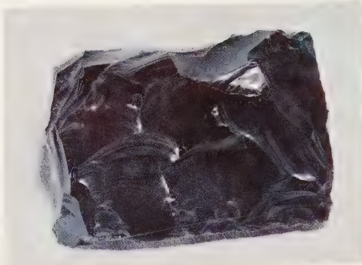
Obsidian
