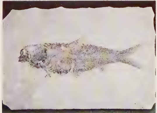
Fossil Fish in Shale
