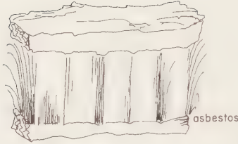
FIBROUS MASSIVE
