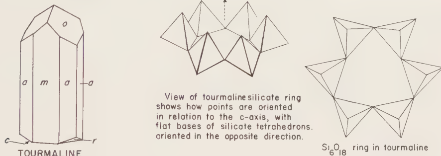
TOURMALINE
