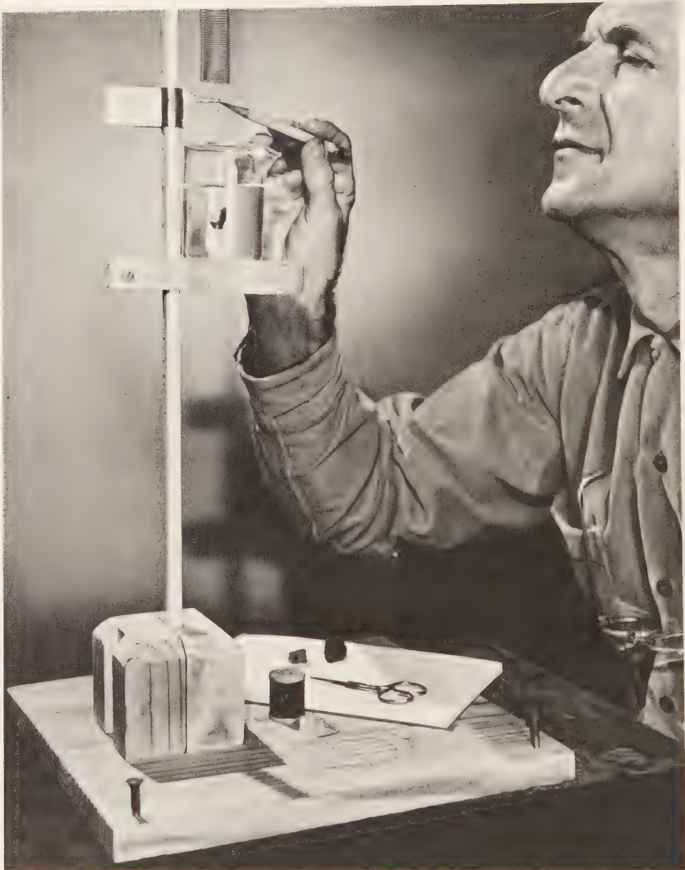
FIG. 86. Jolly balance in use. A specimen is suspended from thread at the lower end of the tension spring and is immersed in water for the weight-in-water reading. The author is checking the metal slider mark against the mark on the spring to see if marks match. The reading is taken from the strip of marked graph paper seen on the back side of the metal curtain rod.
