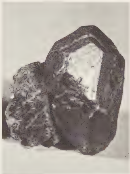
FIG. 150. Ilmenite. Stubby crystal showing a brightly reflective n(2243) face. From Froland, near Arendal, Norway. Size 2" by 2".
