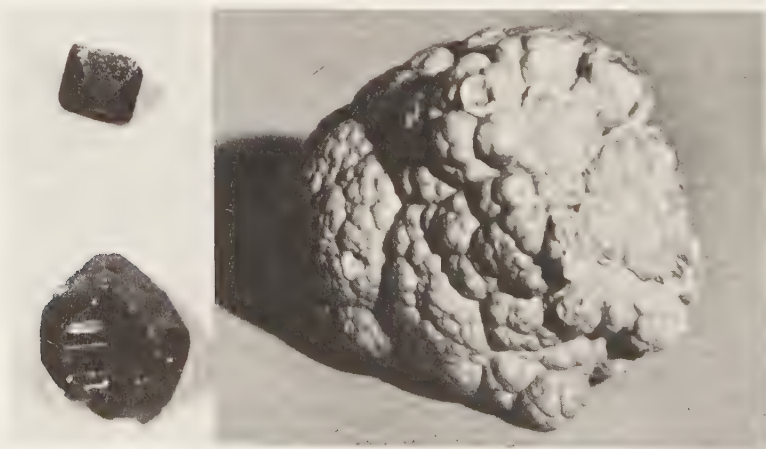
FIG. 155. Cassiterite specimens. Small crystals showing typical dipyramidal form at top left and twin at bottom left. Right: colloidal cassiterite or "wood tin," from the Arroyo Carrizal, Guanajuato, Mexico. Size \frac{1}{2} " diameter.
