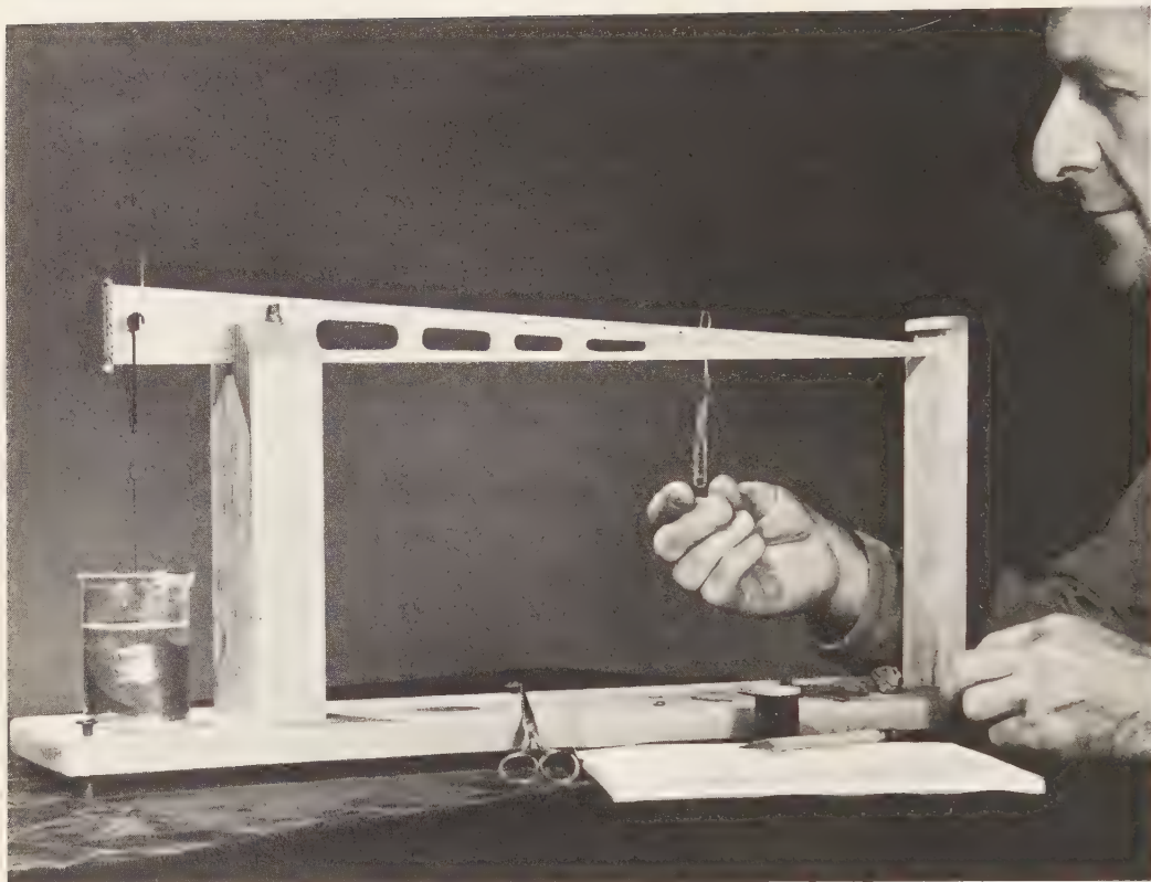
FIG. 84. Homemade specific gravity beam balance in use. A specimen suspended with thread is immersed in a beaker of water at the left. The author is adjusting the position of the paper-clip rider to achieve balance. The point of the paper clip is near the forward edge of the balsa wood beam, upon which is pasted a strip of ten-division graph paper, suitably calibrated, and from which the reading of weight-in-water is to be obtained.
