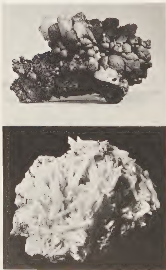
FIG. 188. Cerussite specimens. Top: small gray sixling twins on botryoidal psilomelane from the Campbell Shaft, Bisbee, Cochise County, Arizona. Size 2\frac{3}{4} " by 1\frac{3}{4} ". Bottom: "jackstraw" aggregate of acicular white cerussite on limonite gossan matrix. Flux Mine, Santa Cruz County, Arizona. Size 3\frac{1}{2} " by 3".
