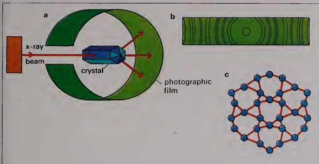
Above: X-ray diffraction. (a) x-rays are passed through a crystal; (b) rays that are diffracted (scattered) are registered on film; (c) the atomic pattern is then worked out
