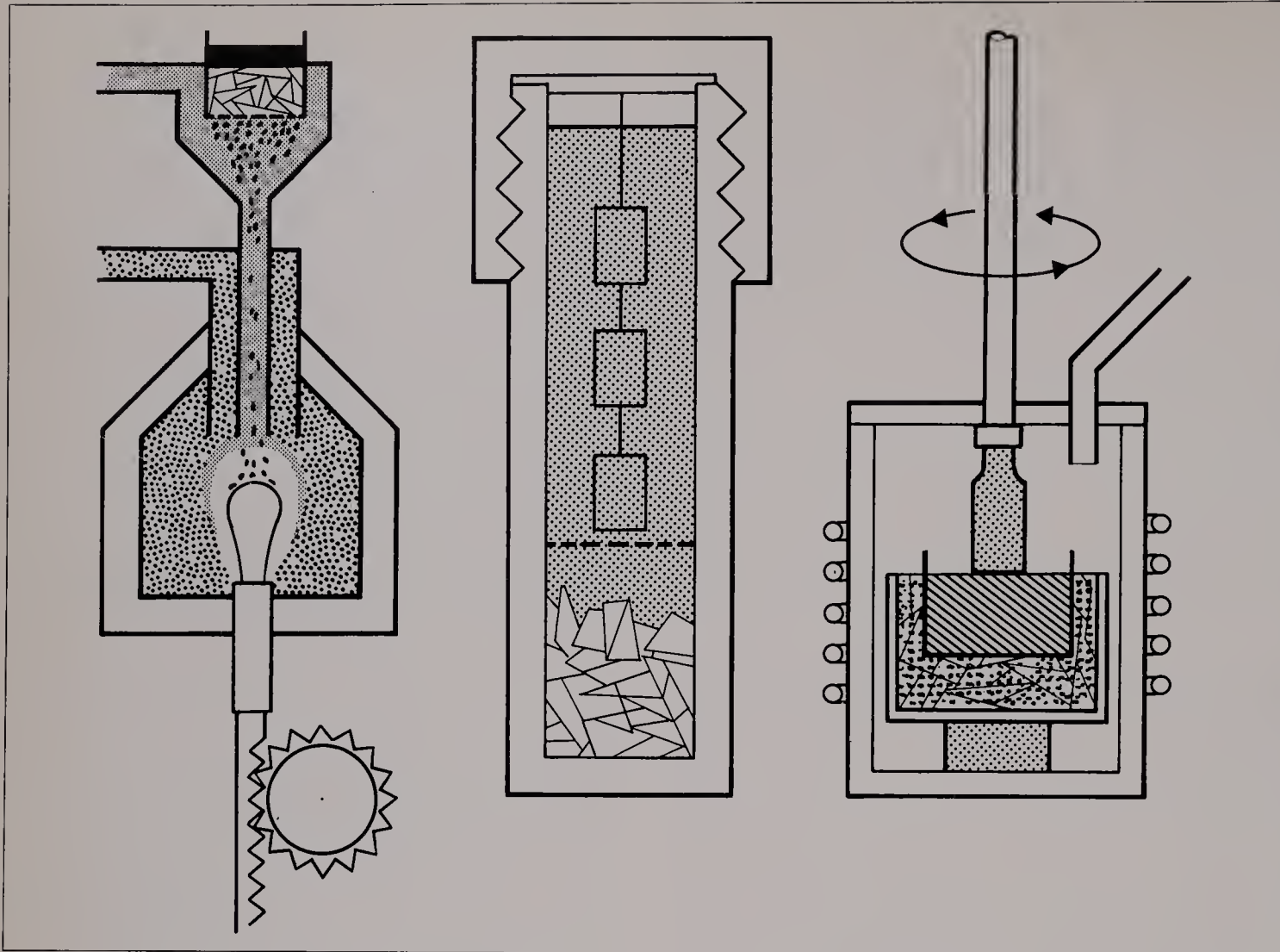
Left: The three most common methods of making synthetic gems. In the Verneuil furnace (far left) a stream of powdered alumina and a colouring agent falls through an oxyhydrogen flame, is melted and drops onto a 'boule' of already crystallized material, to which it adds. In the autoclave (centre) feed material is dissolved in an aqueous solution at a high temperature and pressure. It is deposited on 'seed plates' in the cooler upper parts of the vessel. In the Czochralski process (near left) a seed is slowly withdrawn from a melt while being rotated. New growth occurs at the zone of contact between seed and melt
