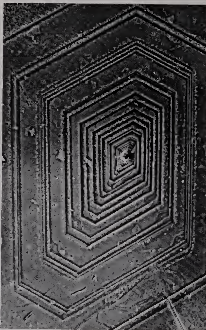
Left: Dislocation of the screw type. Again growth takes place at the 'step'. But though the step changes position, it never vanishes
