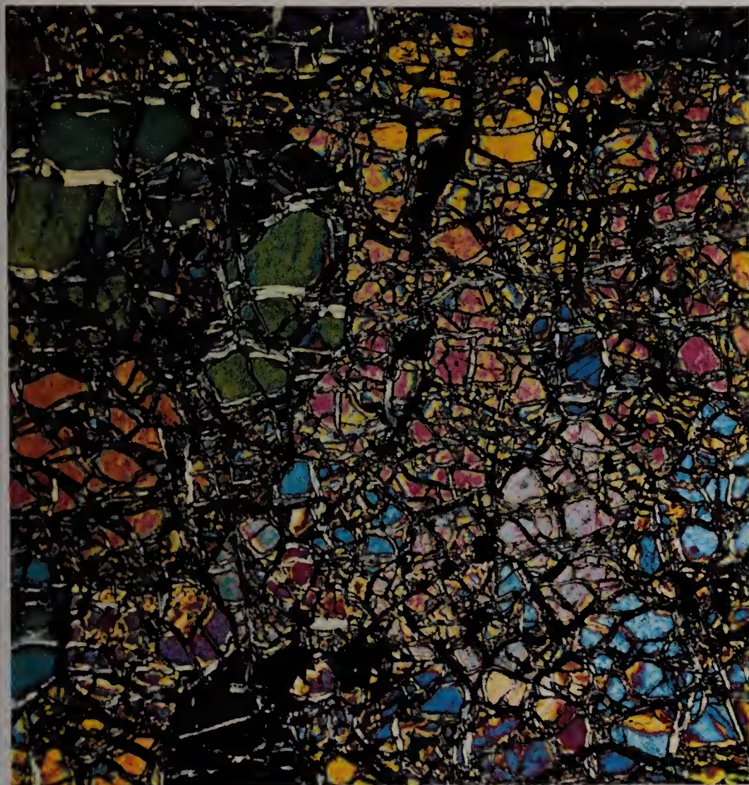
Above: Thin section of dunite seen through crossed polarizers. Individual grains are revealed in different colours. Dunite is a rock consisting entirely of members of the olivine series
