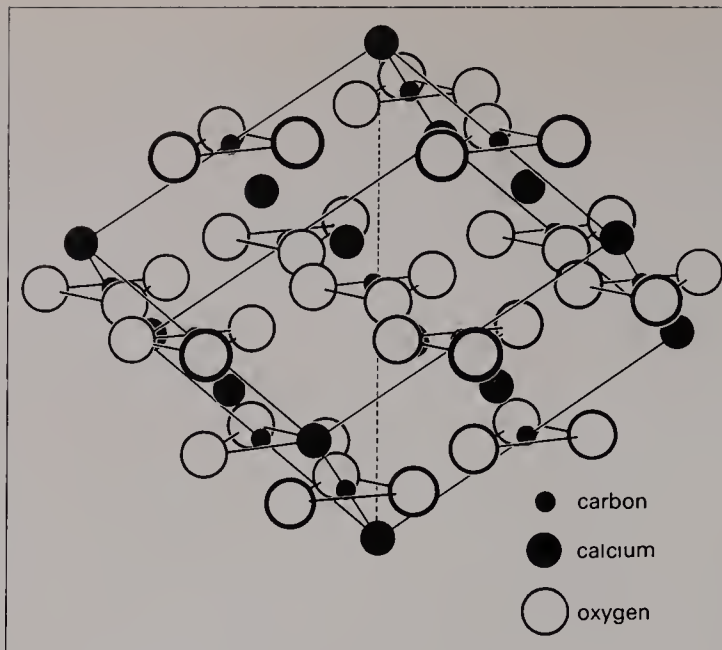
Left: Unit cell of calcite. This is the crystal's building block and is itself made up of atoms of carbon, calcium and oxygen
