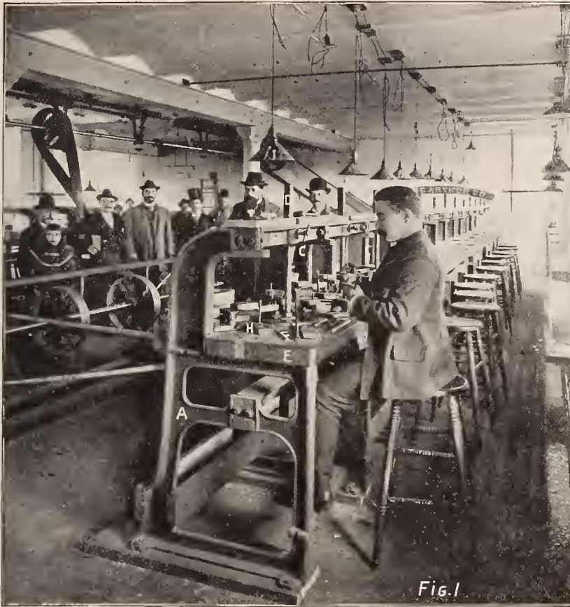
POLISHING MILL SHOWING DETAILS OF CONSTRUCTION.
