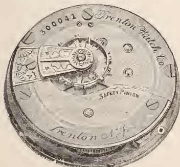
18 SIZE, 7 JEWELS.
