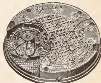
16 SIZE, 16 JEWELS.
