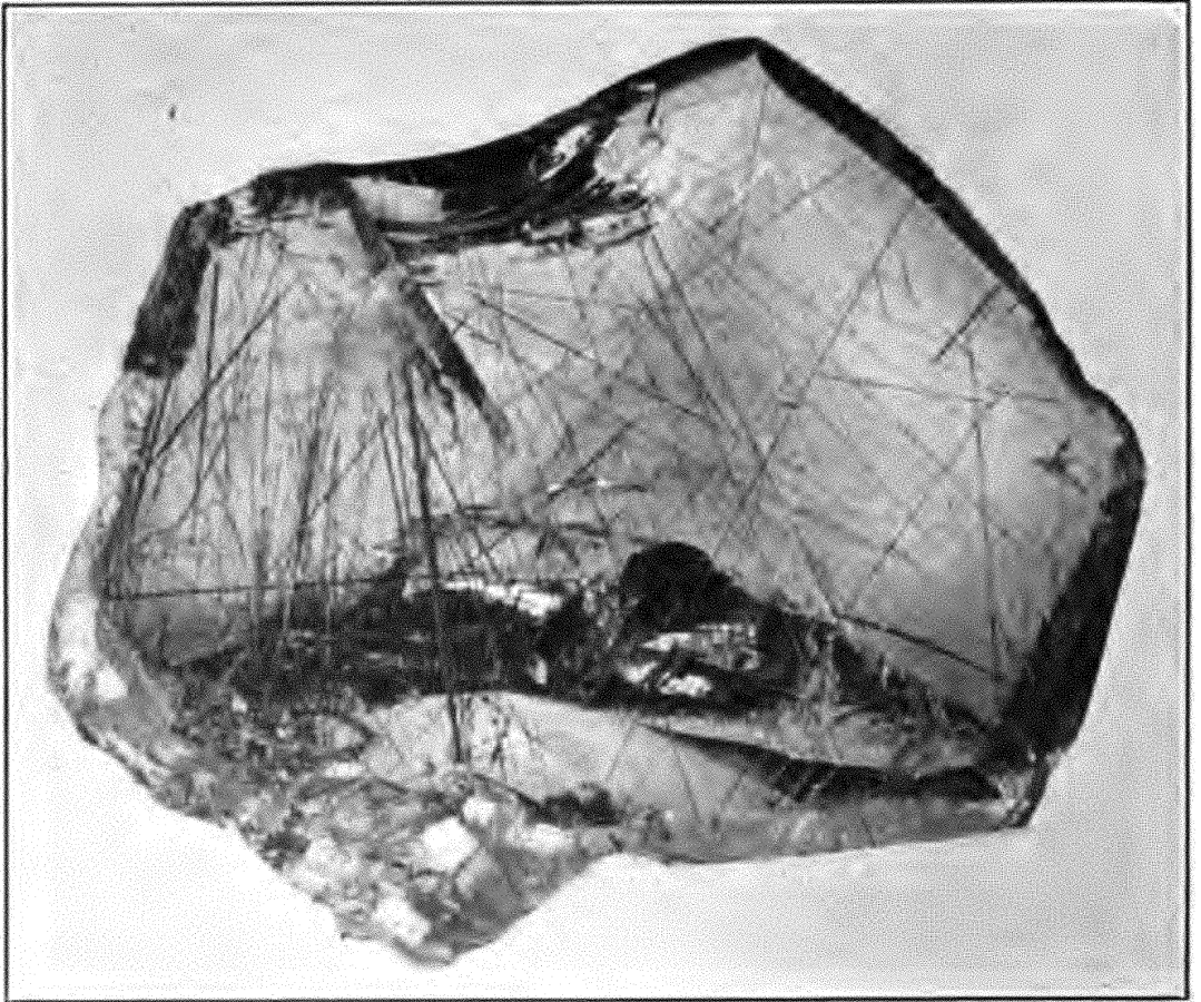
FIG. 10.—QUARTZ CONTAINING RUTILE NEEDLES.
