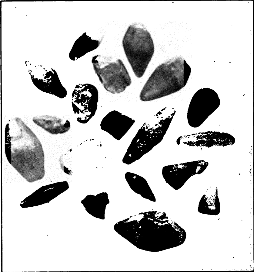
FIG. 4.—CORUNDUM CRYSTALS.
