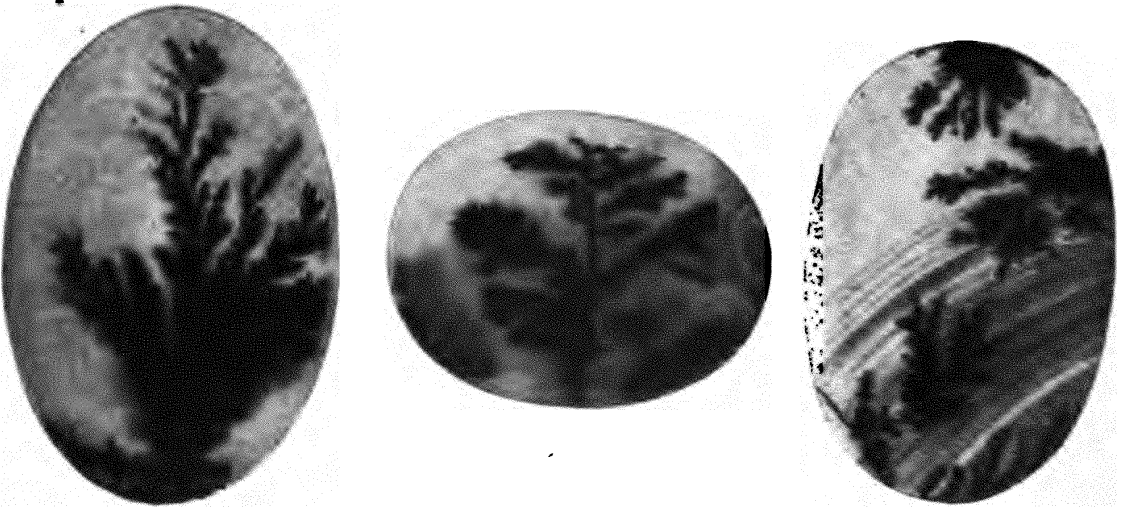
FIG. 3.—MOSS AGATES.
