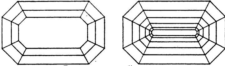
FIG. 23.—UPPER AND UNDER SIDES OF TRAP CUT.
