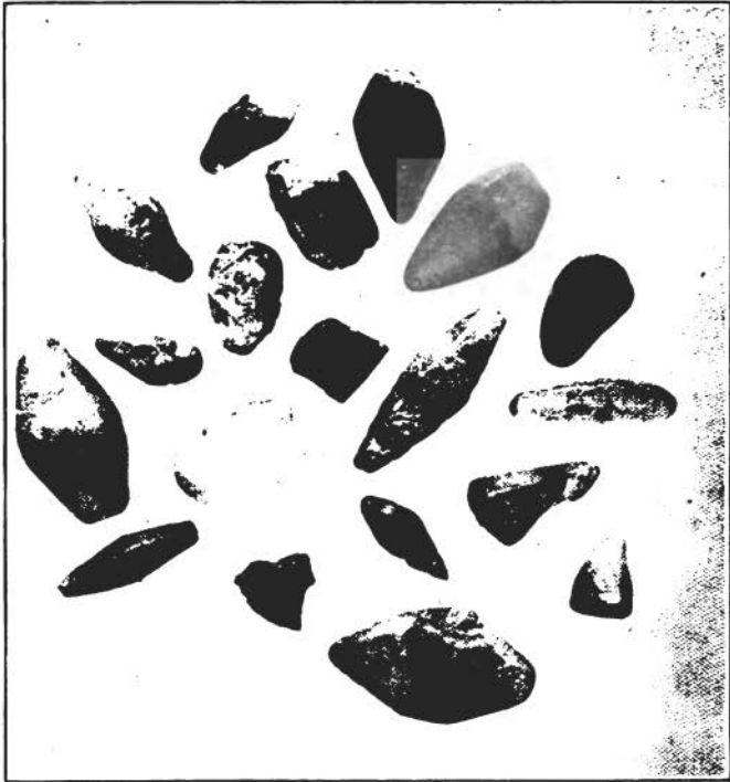
FIG. 4.—CORUNDUM CRYSTALS.
