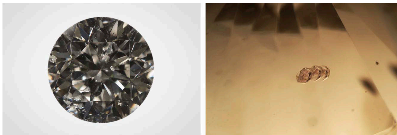
Figure 9. Left: Face-up image of the 0.13 ct round brilliant diamond. Right: Photomicrograph of the largest corundum inclusion exhibiting a slight pinkish color when viewed through a microscope with a diffuser plate. The triple image of the inclusion is due to the diamond's faceting. Field of view 1.76 mm.
