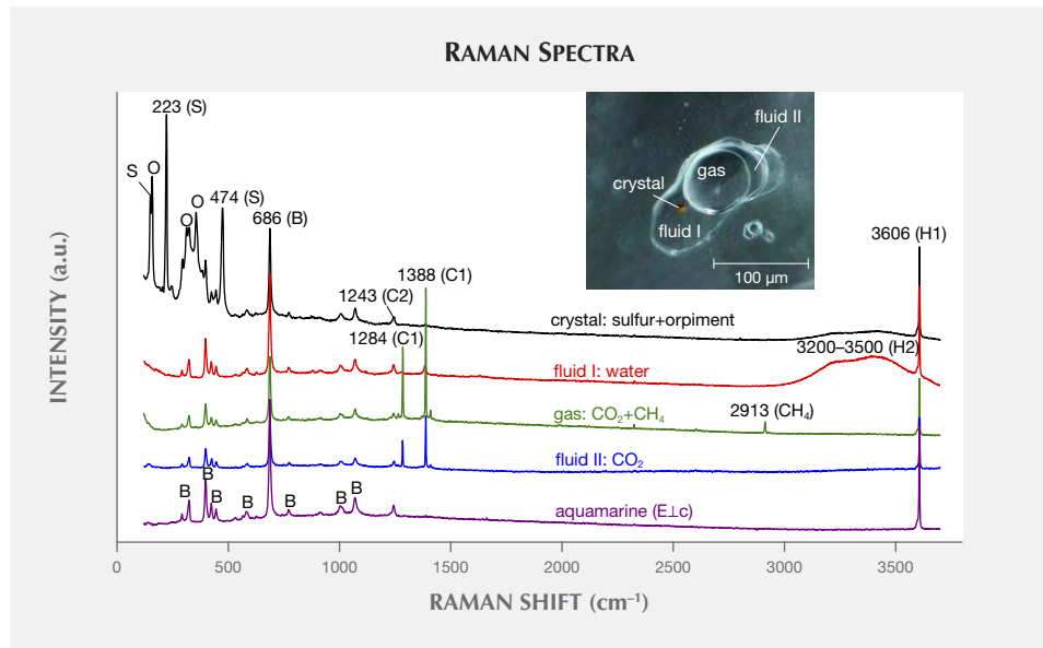
Figure 3. This multi-phase inclusion had two fluid phases, one gaseous phase, and one crystal phase. Abbreviations: B—beryl, S—sulfur, O—orpiment, C1—CO 2 in the inclusion, C2—CO 2 in the beryl structure channel, H1—water in the beryl structure channel, and H2—water in the inclusion. Spectra are offset vertically for clarity. Photomicrograph by Yang Hu.
