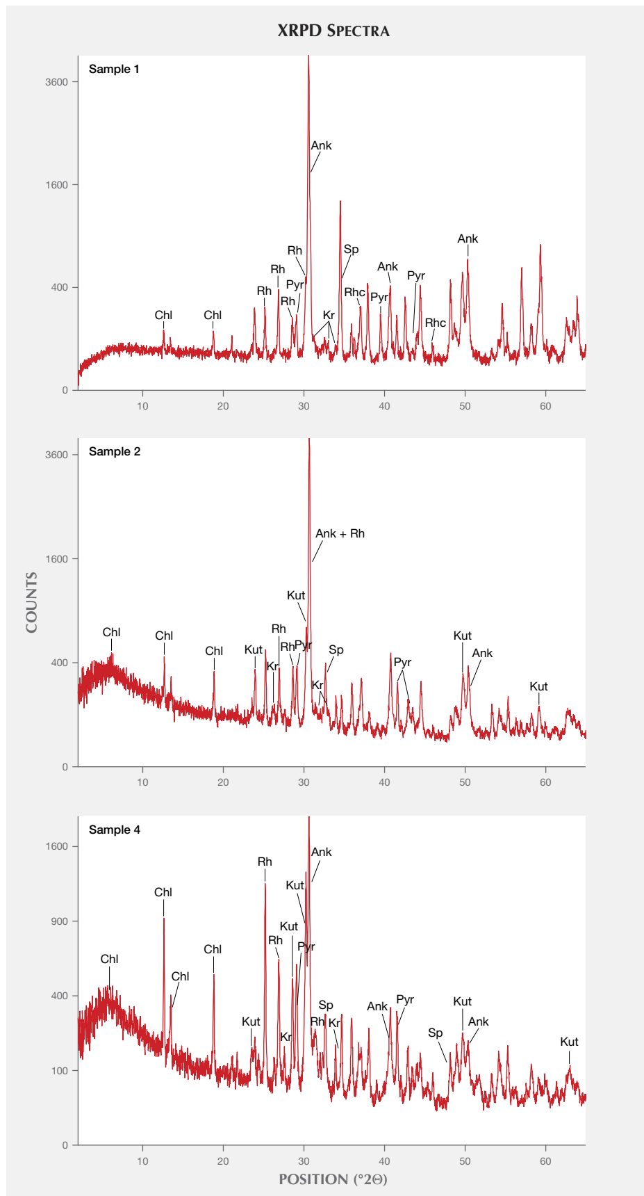
Figure 7. XRPD patterns of the rhodonite samples 1, 2, and 4 from figure 4. The most important minerals are reported, close to their diagnostic peaks. Ank = ankerite; Pyr = pyroxmangite; Rh = rhodonite; Kut = kutnohorite; Sp= spessartine; Rhc = rhodochrosite; Chl = chlorite.
