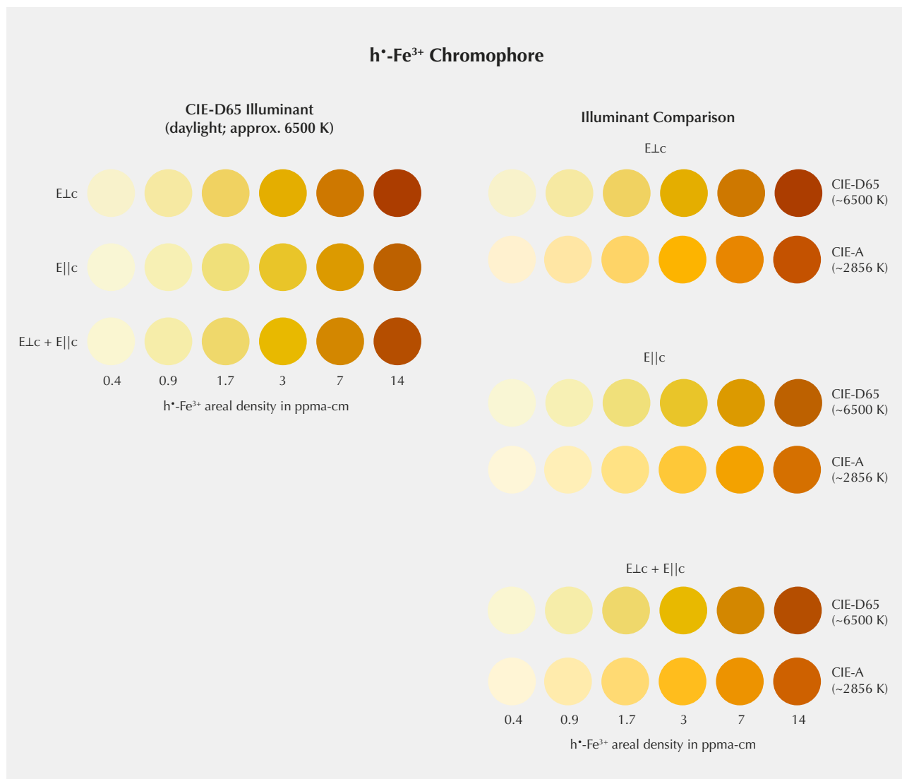
Figure 13. Left: Areal density color circles for the h • -Fe 3+ chromophore. Right: Illuminant comparison of the h • -Fe 3+ chromophore. Little color change is observed with the change in illuminant for all orientations.
