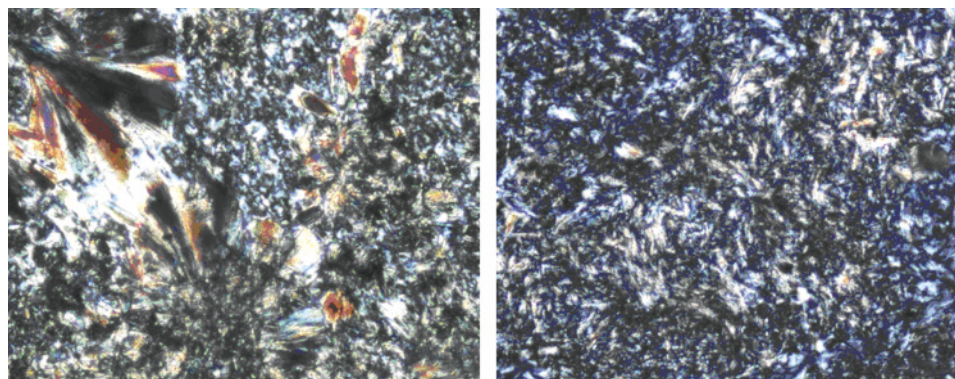
Figure 6. The nephrite slab displays band (left) and unpatterned areas (right). The band's tremolites are fibrous, columnar, of varying particle size, and poorly oriented. The interwoven tremolites of the unpatterned area are fine, with homogeneous particle size. Photomicrographs by Zuowei Yin; image widths 0.57 mm.
