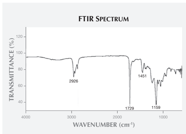
Figure 14. The FTIR spectrum of the coating scraped from the surface of the fire opal exhibits characteristic peaks at 2926 , 1729 , 1451 , and 1159\ \text{cm}^{-1} consistent with acrylic polymer.
