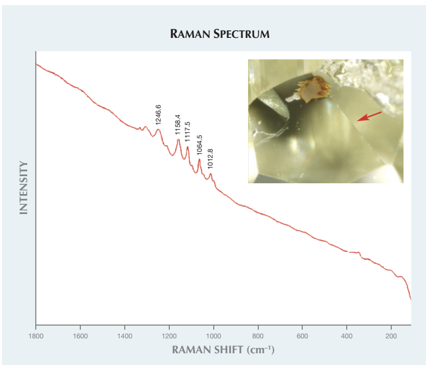
Figure 7. The xenotime inclusion broke through the pavilion surface (inset; magnified 80 \times ). Radiation stains were also observed at the contact with the host diamond (see arrow). The Raman spectrum, using a 514 nm laser, shows xenotime peaks at 1012.8, 1064.5, 1117.5, 1158.4, and 1246.6 \text{cm}^{-1} .
