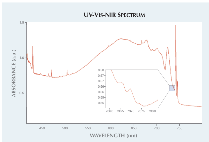
Figure 13. The visible-NIR spectrum of the 0.46 ct irradiated synthetic diamond showed a clear Si-doublet at 737 nm.
