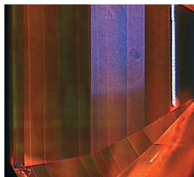
Figure 17. DiamondView imaging showed banded red fluorescence with a striated pattern, typical of CVD synthetic diamonds.
