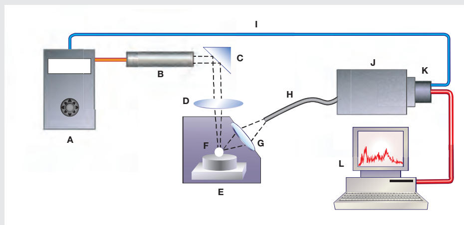
Figure A-1. This diagram shows the main components of a modern LIBS system: (a) laser source and cooler; (b) pulsed laser head; (c) mirror; (d) focusing lens; (e) excitation chamber; (f) sample; (g) collecting optics; (h) optical fiber; (i) detector trigger signal; (j) wavelength selector; (k) detector array; and (l) microcomputer. From Pasquini et al. (2007).
