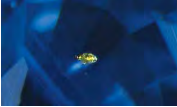
This unheated sapphire from the Ban Huai Sai area, Laos, contains a conspicuous inclusion of yellow monazite. Photomicrograph by S. Singhamroong, ©Dubai Gemstone Laboratory; magnified 25×, oblique illumination.
