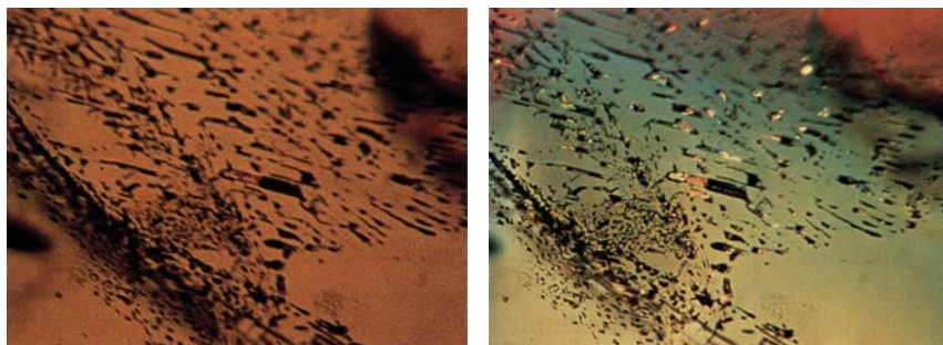
Figure 7. Healed fractures in taaffeite have been noted in the literature, but without identifying the the solid phase in the negative crystals as magnesite. Left: the healed fractures with standard illumination. Right: tiny birefringent crystals are visible in the negative crystals with crossed-polarized light. Immersion, magnified 80 \times .
