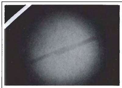
Figure 22. This X-radiograph shows the predrilled nucleus of one of the pearls in figure 21.
