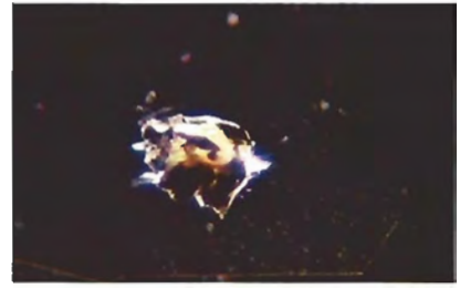
Figure 19. A phlogopite mica inclusion in the sapphire shown in figure 18. Magnified 63×.
