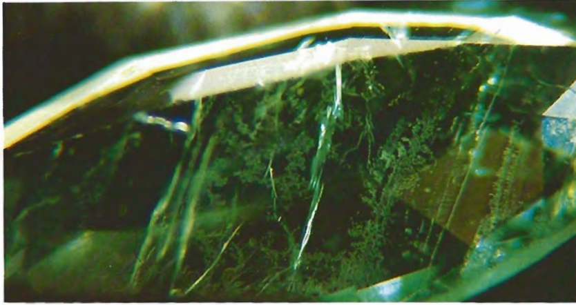
Figure 7. These fractures containing dendritic deposits became visible after the oiled emerald was heated during manufacturing. Magnified 33×.
