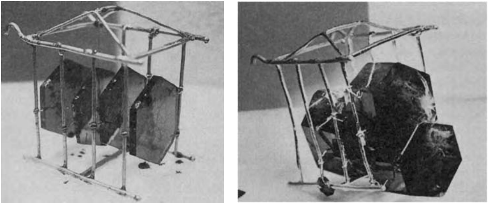
Figure 15.7 (left) Platinum cage containing Gilson synthetic seed plates after 2 months overgrowth. (right) Gilson synthetic emerald crystals after 10 months growth. (Gilson)
