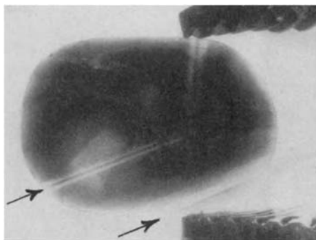
Figure 16.19 (left) Straight colour zoning in natural sapphire; (right) Curved colour zoning in synthetic Verneuil sapphire
