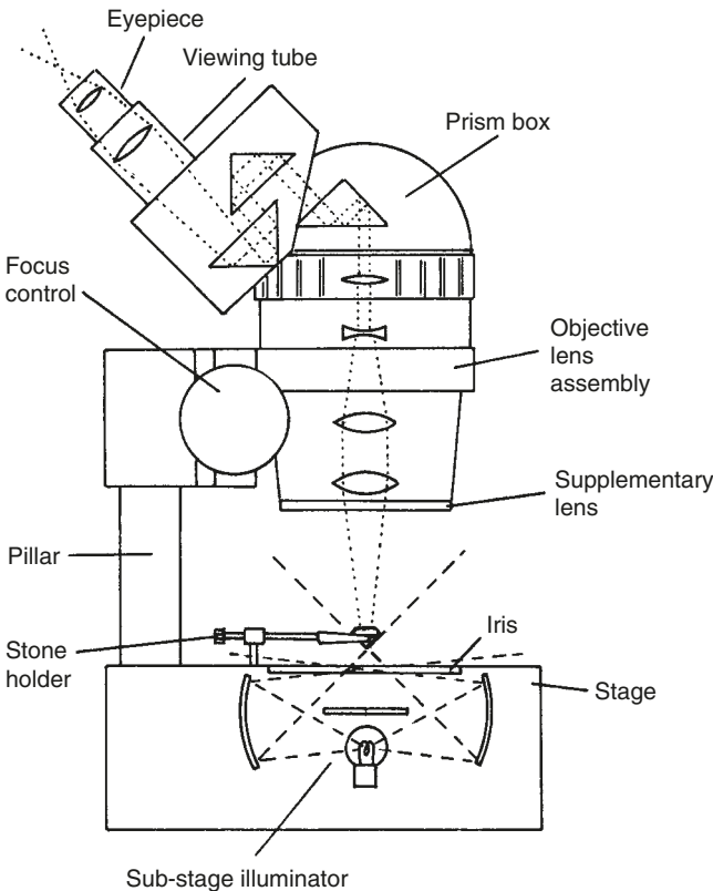
Figure 13.8 Sketch showing the components and one of the two ray paths in a typical stereo microscope. The illuminator in the sub-stage section is set for dark-field work
