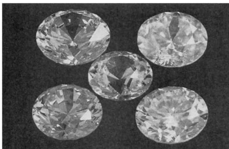
Figure 17.4 Five diamond simulants photographed at an angle to illustrate the 'light spill' test. The centre stone is a YAG (RI = 1.83); the top left is a GGG (RI = 1.97); top right is a lithium niobate (RI = 2.25); bottom left is a CZ (RI = 2.16); bottom right is a strontium titanate (RI = 2.42) which, like diamond, shows no light leakage through the pavilion facets
