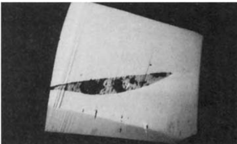
Figure 14.10 The glass-filled pits and cracks of rubies have a lower lustre compared with the surrounding corundum. Gas bubbles in the glass appear as black circular areas. (R.W. Hughes)
