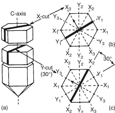
Figure 12.9 The piezoelectric effect in a quartz crystal (a) produces mechanical stress along the Y axes when an electrical charge is applied across the X axes (b) Plates are cut from the crystal as shown for use in electrical oscillators. The 30^\circ Y -cut plate (c) oscillates more readily, particularly at lower frequencies, than the X -cut plate
