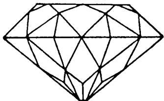
Figure 19.12 The zircon cut has additional facets placed around the culet to prevent the loss of light through the base of the pavilion
