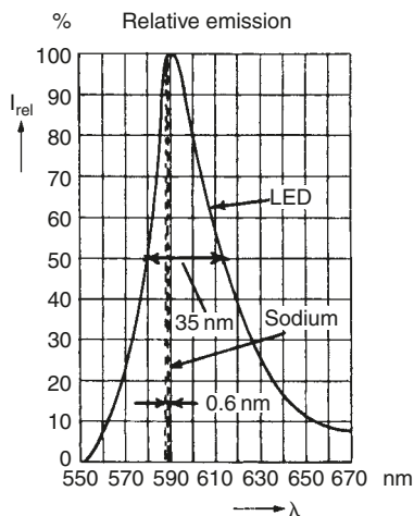
Figure 9.9 (left) Graph comparing the emission bandwidth of a typical LED light source with that of a sodium lamp. (right) A battery-operated Gem-A refractometer light source using a high-brightness LED with a peak emission at 590 nm. An adjusting screw under the front edge allows the light to be aligned with the light aperture of any refractometer
