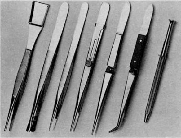
Figure 13.17 A selection of stone tweezers. The middle one has a locking slide to maintain the tweezers grip without the need for finger pressure. The two on the right of it have press-to-open reverse action
