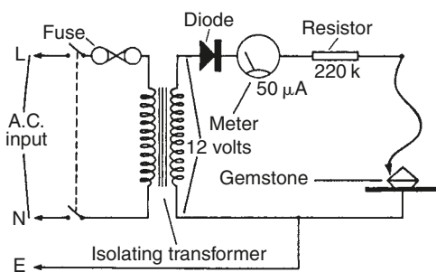
Figure 12.8 (left) A test circuit for checking the electrical conductivity of gemstones. (right) The battery-operated Synthetic Moissanite Megger Tester Mk II detects the semiconductor property of this diamond simulant (see text). The tester also verifies the semiconductor property of natural blue diamonds and synthetic boron-doped blue diamonds (diamonds whose blue colour has been artificially induced by atomic irradiation are non-conductors of electricity). (Gemmological Instruments)
