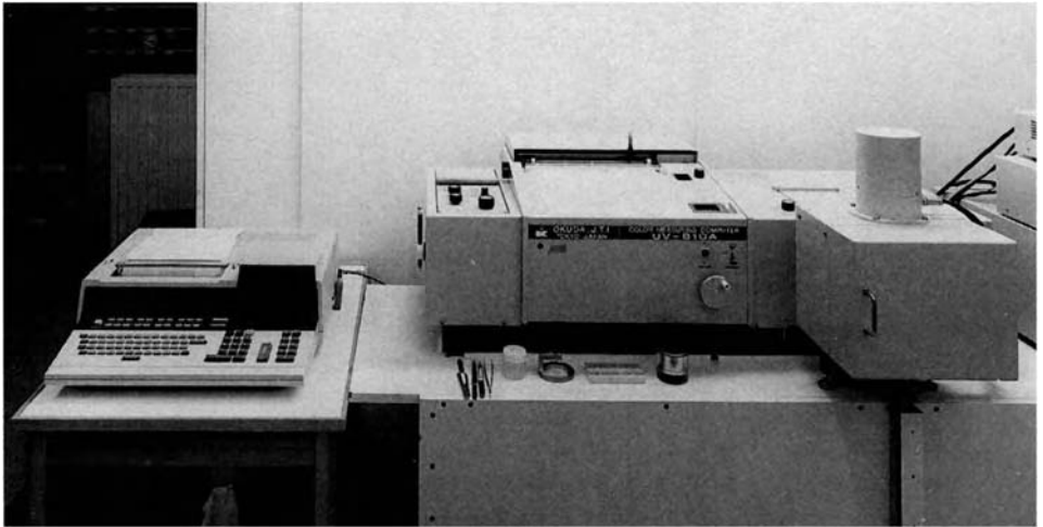
Figure 16.23 A spectrophotometer designed to measure the colour grade of cut stones. On the left is the control unit, in the centre the sample chamber and detector, and on the right the light source and monochromator
