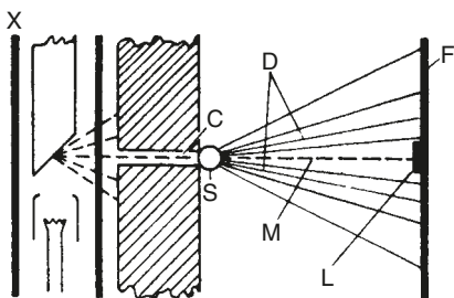
Figure 18.10 Diagram illustrating the production of a pearl lauegram: X = X-ray tube; C = collimator; S = pearl; D = diffracted X-rays; M = main X-ray beam; L = lead disk to absorb main beam (usually omitted when testing pearls); F = photographic film
