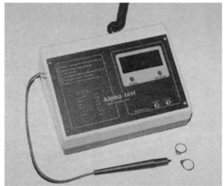
Figure 12.13 The Alpha-test instrument is a thermal tester designed to check the thermal conductivities of a range of gemstones (including diamond and its simulants). (H.S. Walsh & Sons Ltd)
