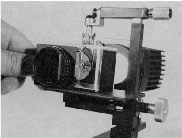
Figure 13.13 A twin polarizer attachment that can be fitted over a microscope's immersion cell to act as a polariscope. (Eickhorst)
