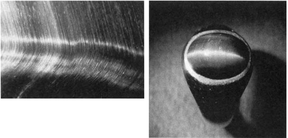
Figure 8.7 (left) An enlarged view of the parallel quartz channels just beneath the surface of a polished section of tiger's-eye. The bright chatoyant lines are running roughly at right angles to these channels. (right) A cabochon of tiger's-eye cut to show the chatoyant sheen effect
