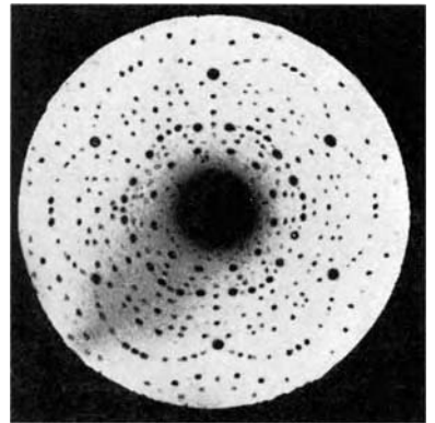
Figure 16.26 (below right) Laue diffraction pattern (taken parallel to the 'c' axis of a beryl crystal) showing six-fold symmetry: (below left) Lauegram taken parallel to the trigonal axis of symmetry of a crystal
