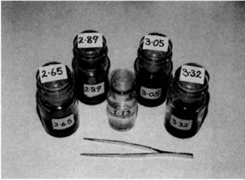
Figure 7.9 A set of heavy liquids used in estimating the SG of a gemstone. The smaller bottle in the centre contains a salt solution for testing amber (see under the heading ‘Amber’ in Chapter 18)
