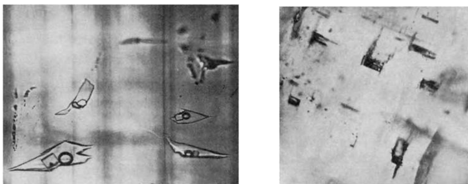
Figure 16.4 A Colombian Chivor mine emerald (left) showing three-phase inclusions. An Indian emerald (right) with comma-like two-phase inclusions
