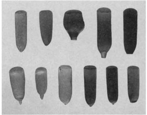
Figure 15.3 A typical selection of corundum and spinel boules grown in a Verneuil furnace. (D. Swarovsky)
