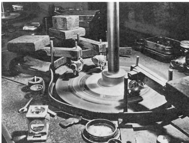
Figure 19.25 Mechanical clamp-type dops holding diamonds on a scaife. The dops are mounted on the end of tangs, which are weighted to achieve the necessary polishing pressure. (De Beers)
