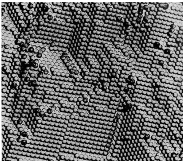
Figure 8.9 The orderly arrangement of silica gel (cristobalite) spheres in opal, as revealed by the electron microscope at the magnification of 25 000 \times
