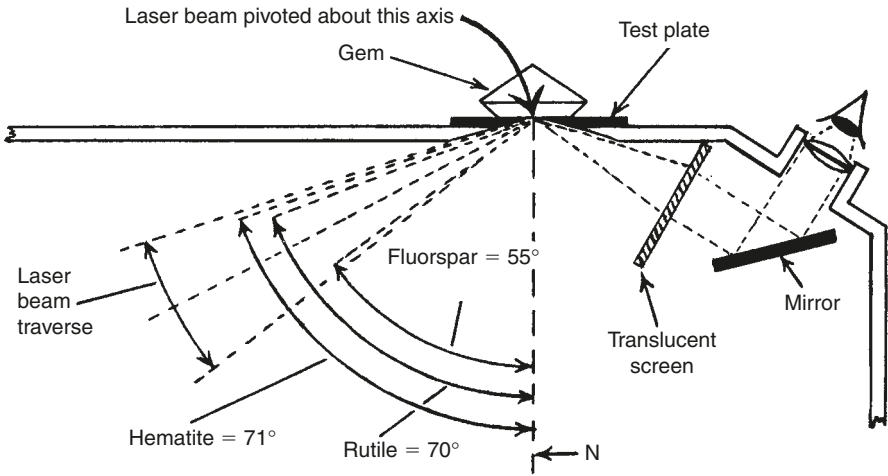
Figure 9.28 Diagram showing the use of the Brewster-angle of polarization to measure a gemstone's RI. The laser beam is vertically polarized, and at the Brewster angle the reflected light imaged on the translucent screen drops to a minimum
