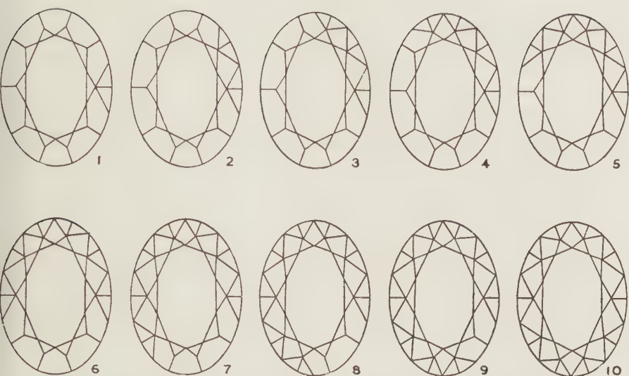
Figure 61. Cutting the Crown Break Facets of an Elliptical Brilliant. The first break facets are placed on the side to touch the first star facet. This is continued all around the crown in clockwise direction.
