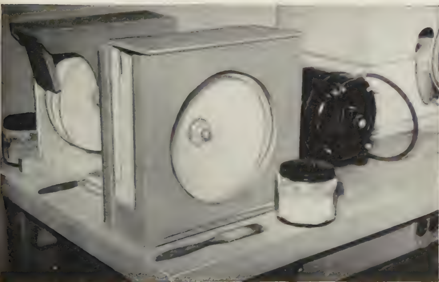
PLATE IV. Polishing bench, showing motor serving a double arbor with internal wooden polishing wheel and hard felt wheel.
