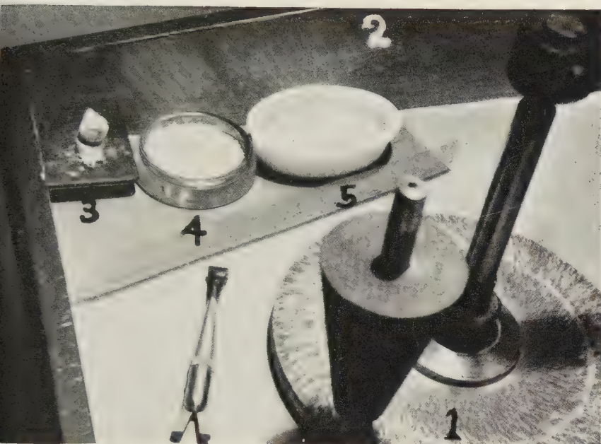
Figure 80. Polishing-Agent and Wetting-Plug Assembly. 1, polishing lap; 2, guard rail; 3, block with wetting plug; 4, polishing agent; 5, water. (Notice that this lap is scored with pits instead of lines).
