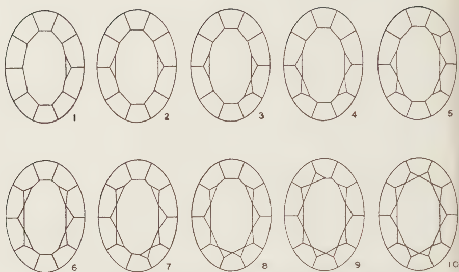
Figure 60. Cutting the Star Facets of an Elliptical Brilliant. Beginning with the first star facet, the rest are cut as opposites.
