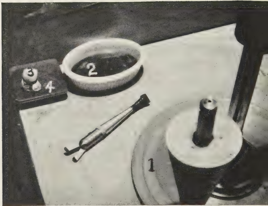
Figure 70. Assembly for Watering the Diamond Lap (view from above). 1, cutting lap; 2, water receptacle; 3, cloth wetting plug; 4, base for plug when not in actual use.
