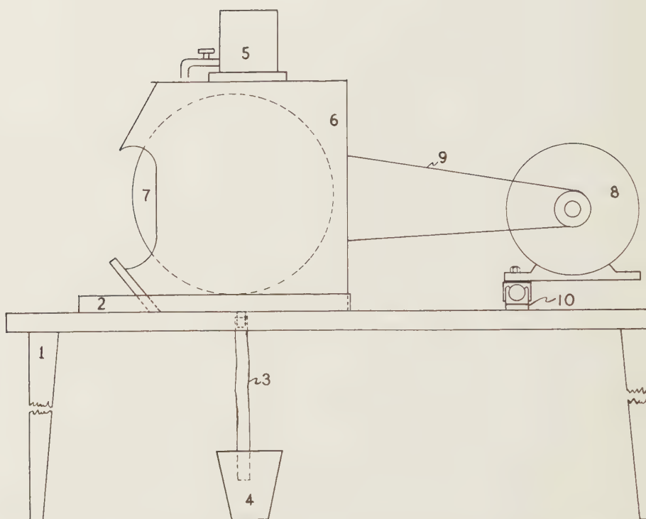
Figure 24. Side View of Complete Grinding Set-Up. 1, table; 2, splash pan; 3, drainage tube; 4, drainage bucket; 5, water reservoir; 6, plyboard splash guard; 7, grinding wheel; 8, motor; 9, drive belt; 10, floating-rail motor mount.
