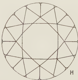
Figure 56. Cutting the Crown Break Facets of a Brilliant. A to H, two break facets are placed on the first main facet, converting it into the shape of a kite. This is continued all around the crown.
