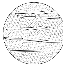
rod-shaped inclusion
