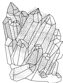
smoky quartz
