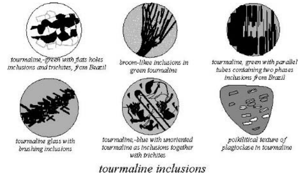
tourmaline inclusions
