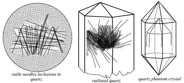
quartz inclusions
