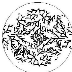
dendritic inclusion
