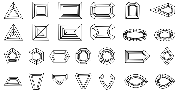
step cuts and mixed cuts
