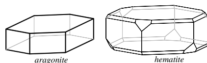
platy crystals
