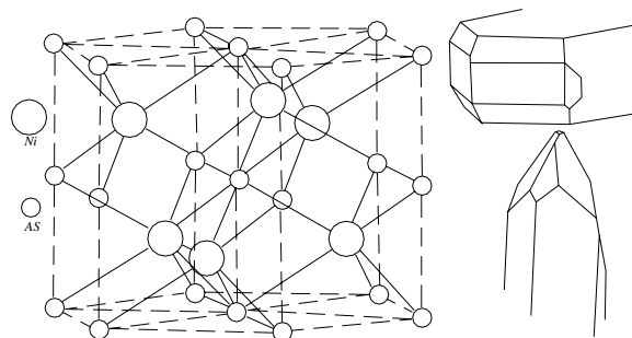
niccolite structure and crystals
