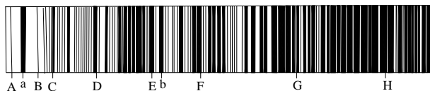
continuous sun absorption spectrum
