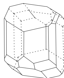
anorthite crystal
