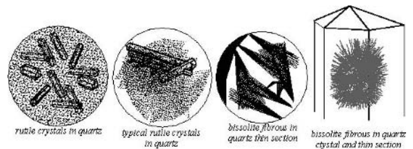
quartz inclusions
