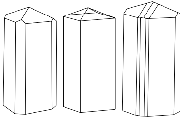
natrolite crystals
