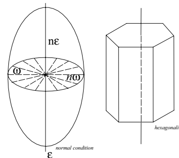
a circular section of an uniaxial crystal with two different refractive indices, n \omega and n\epsilon
