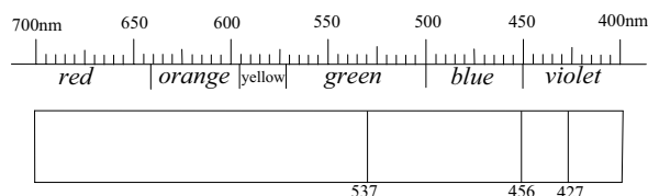
aquamarine absorption spectrum
