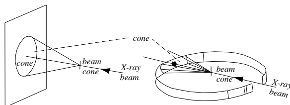
X-ray diffraction of powder
