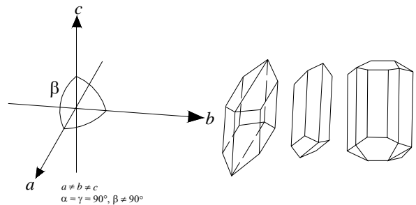
monoclinic system
