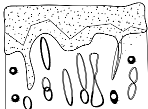
bubbles in different forms in imitation amber from synthetic resin
