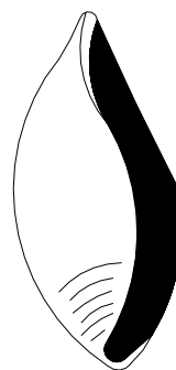
convolute
