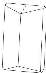
celsian crystal
