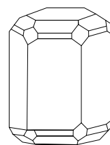
pyromorphite crystal
