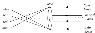
chromatic aberration
