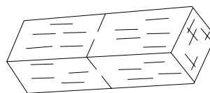
mesolite crystal
