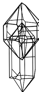
capped-quartz phantom
