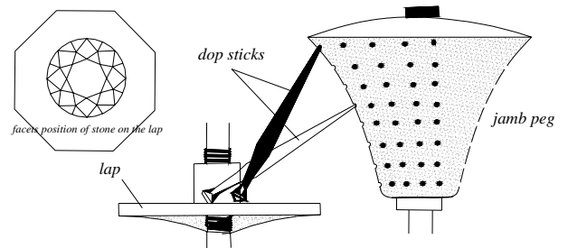
diamond polishing device or jamb peg
