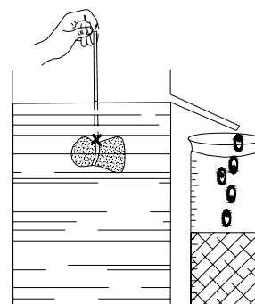
measuring the SG of a mineral by means of its volumetric displacement of water in a diffusion column
