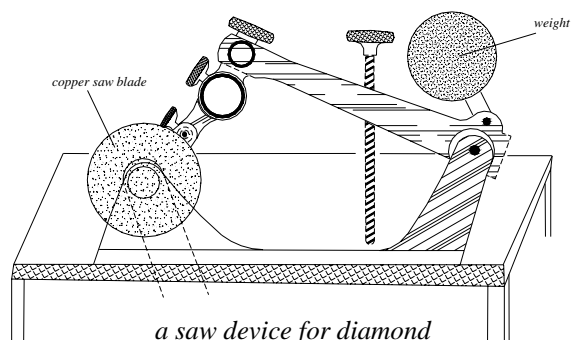
a saw device for diamond
