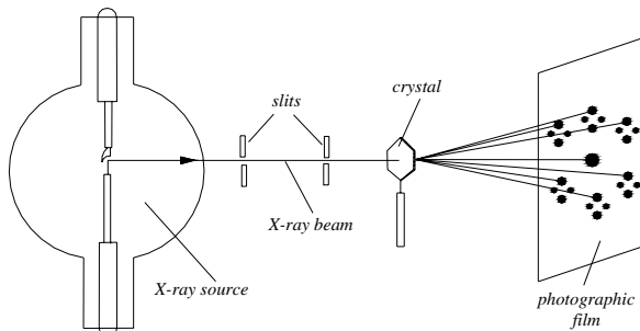
X-ray Laue-method
