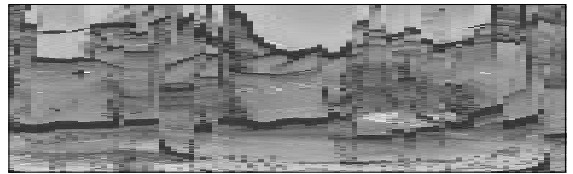
paesinite, Italy
