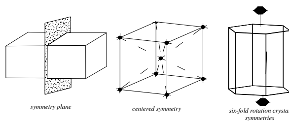
symmetry elements
