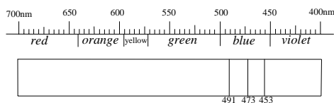
peridot absorption spectrum
