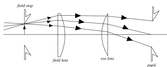
Ramsden eyepiece
