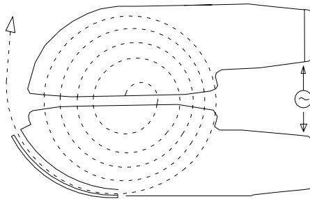
cyclotron
