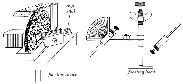
two different faceting devices
