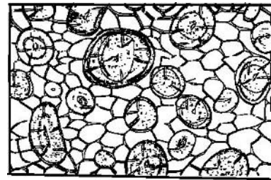
oolitic structure
