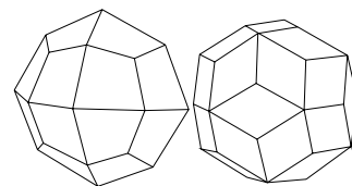
icositetrahedron crystals
