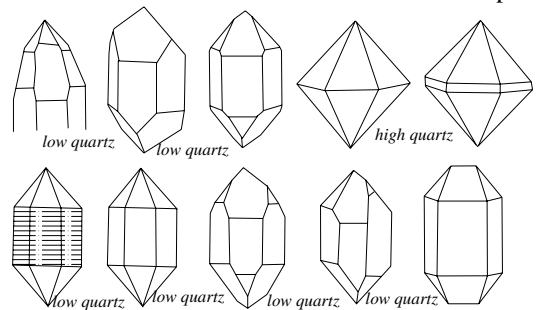
quartz crystals
