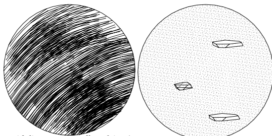
quartz inclusions
