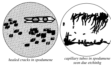
spodumene inclusions
