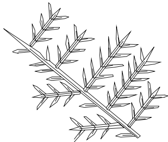
arborescent aggregate.
