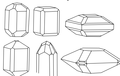
idocrase crystals
