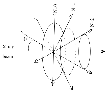
diffraction cones of X-rays
