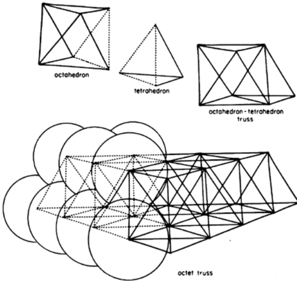
Fig. 420.01 Octet Truss.
