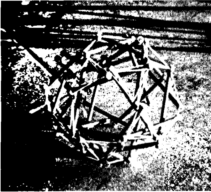
icosadodecahedron
