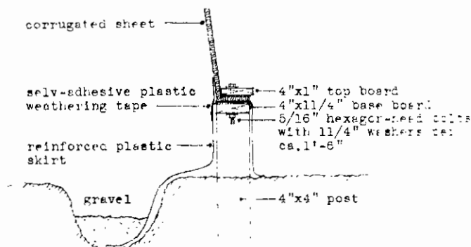
fig. 5. section in base construction
