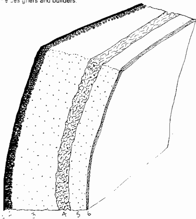
Possible laminar structure for foam dome (section through wall) 1. Elastomeric coating 2. High density foam 3. 2 lb. density foam 4. Open-celled flexible foam 5. 2 lb. foam 6. Plaster or flame retardant paint.
