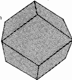
Rhombic dodecahedron
