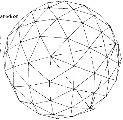
4v triacon icoso face shown dotted
