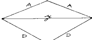
Diamond 2
