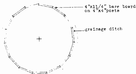
fig. 3. finished base construction
