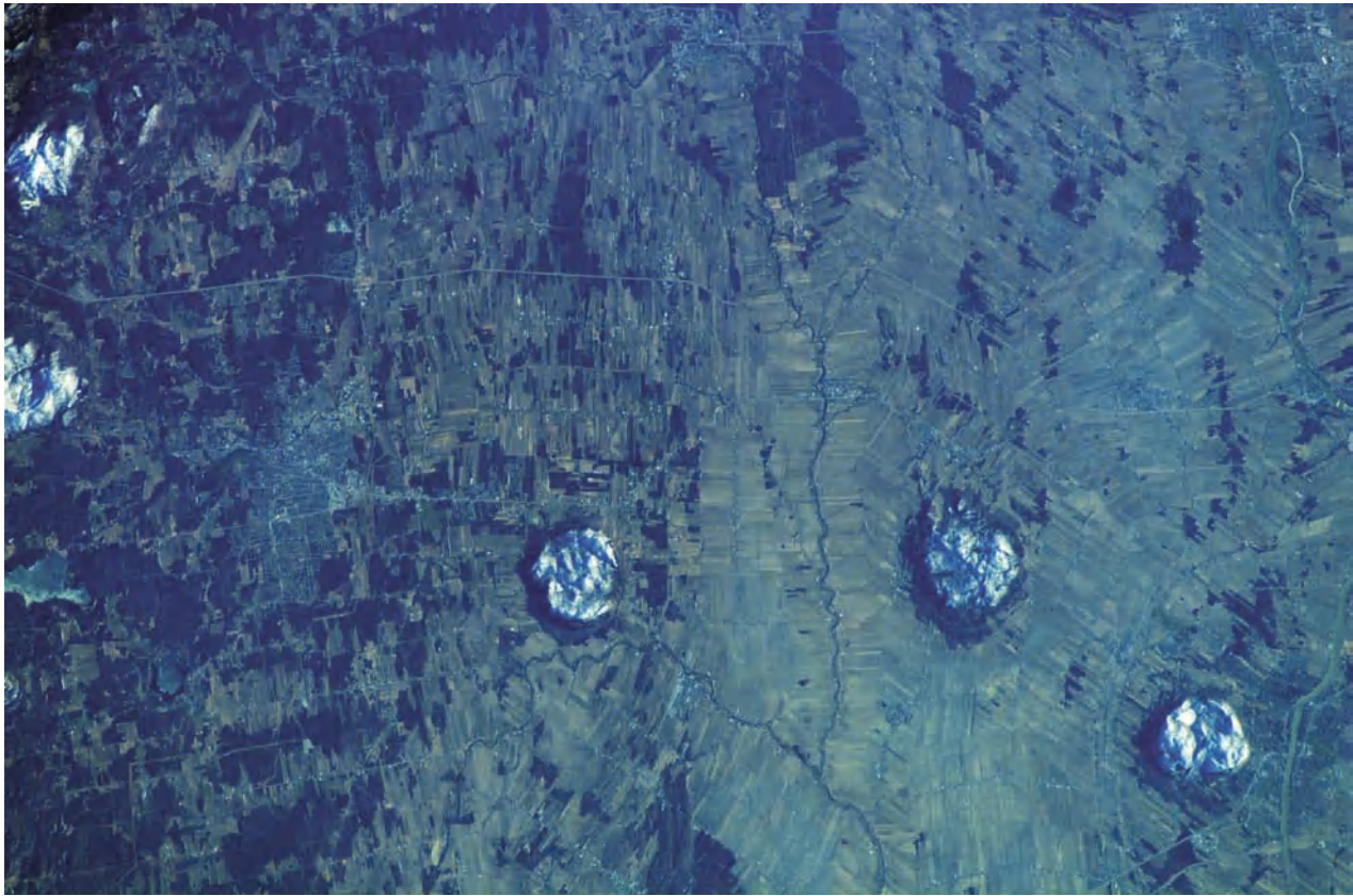
Plutons in Montegian Hills, Quebec, Canada, taken by Expedition 14 crew member in the International Space Station , April 18, 2007 (Earth Sciences and Image Analysis Laboratory, NASA Johnson Space Center)
