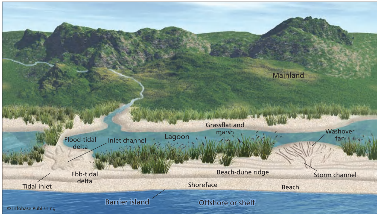
Sketch showing features of a barrier island, tidal inlet, and lagoon coastal system. Note the positions of the small deltas on either side of the tidal inlet, the coastal march, and beach-dune ridge. (modeled after R. Davis and D. Fitzgerald).
