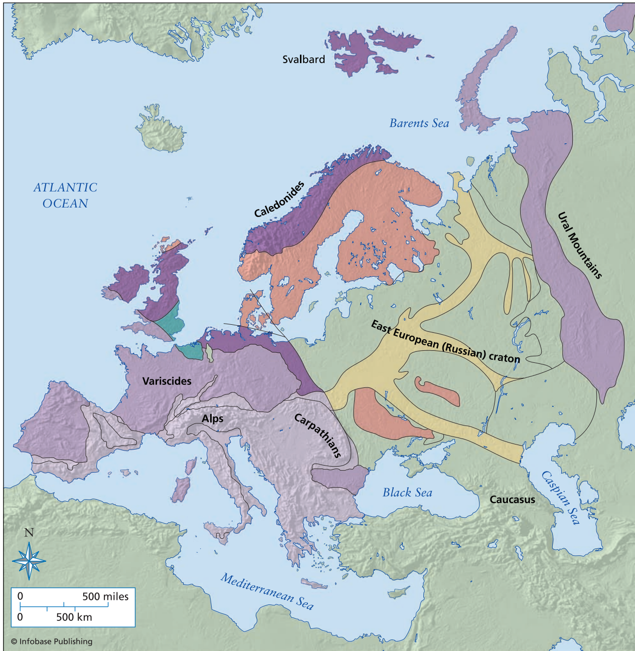
Simplified geological map of Europe showing the location of the Alps, Caledonides, East European (Russian) craton, Urals, Svalbard, and Caspian Sea
