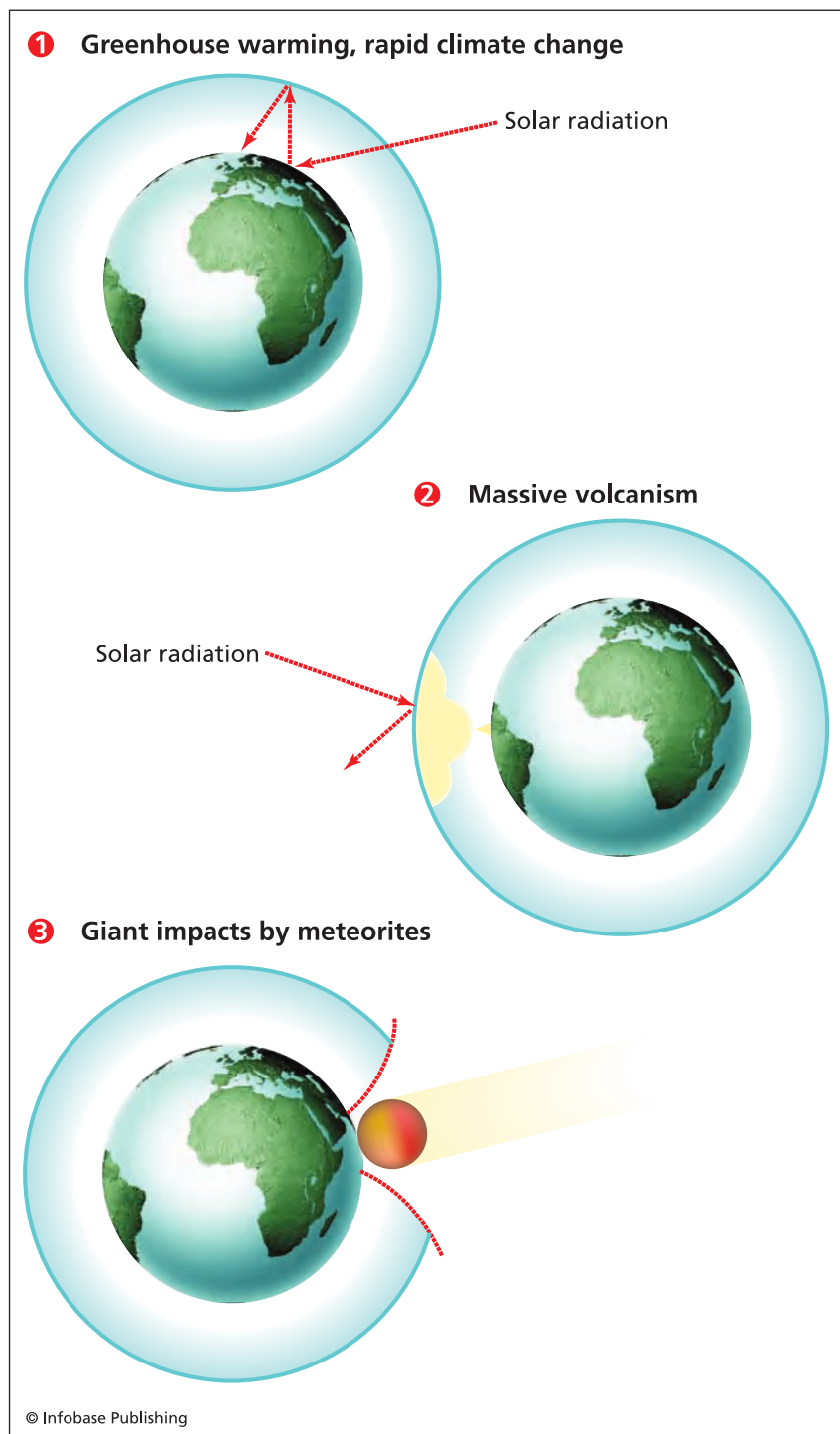
The main causes for mass extinctions, including (1) greenhouse warming and rapid climate change, followed by (2) massive volcanism, and (3) giant impact from space objects such as asteroids or comets
