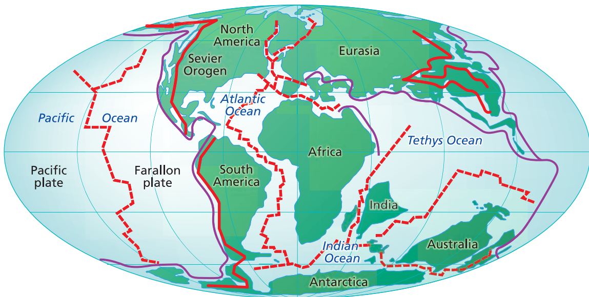
Late Cretaceous 80 Ma Global hothouse; high sea level; high seafloor spreading
