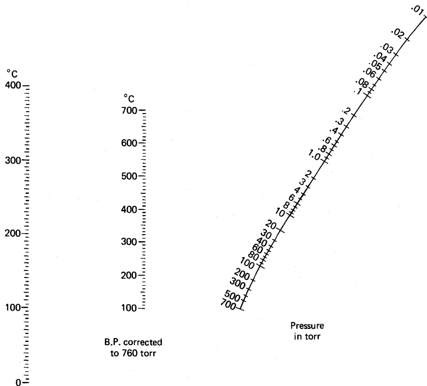
Fig. 77 A clean nomogram for your own use.
