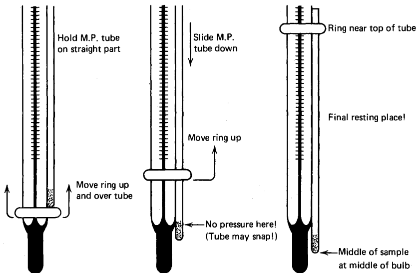
Fig. 40 Attaching M. P. tube to thermometer without a disaster.
