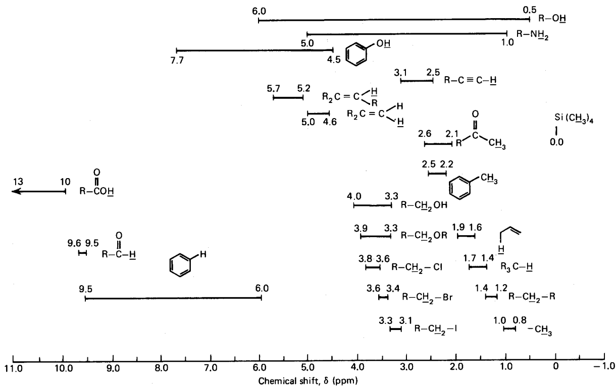
Fig. 136 A garden variety NMR correlation chart.
