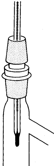
Fig. 25 The adapter stands on its head.
