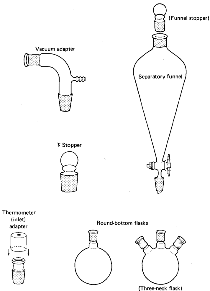
Fig. 19 Some jointware.
