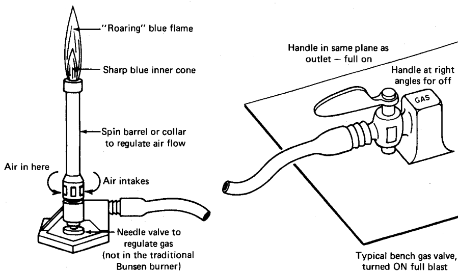
Fig. 58 More than you may care to know about burners.
