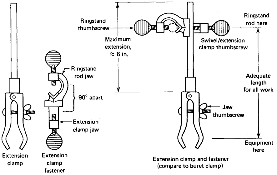
Fig. 66 The extension clamp and clamp fastener.
