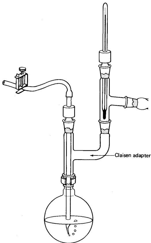
Fig. 78 A Claisen adapter so you can vacuum distill and take temperatures too.
