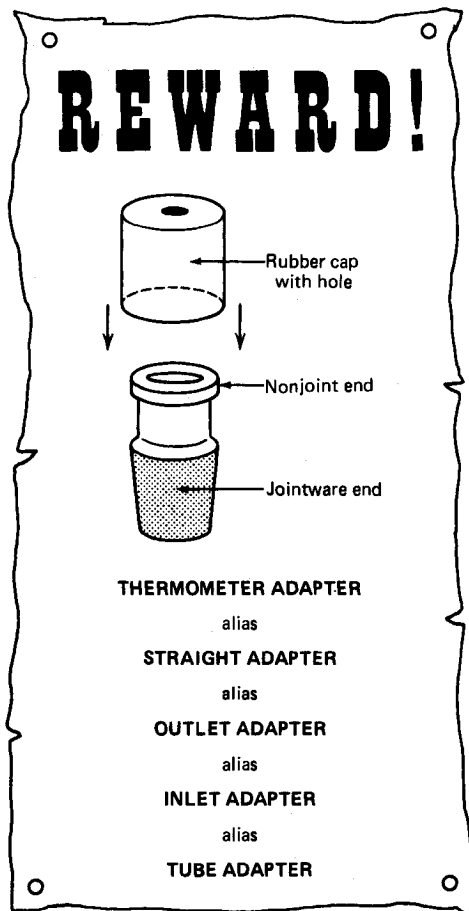
Fig. 22 Thermometer adapter.
