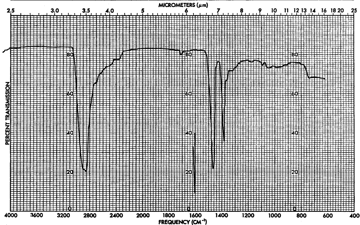
Fig. 122 A published reference Nujol spectrum.
