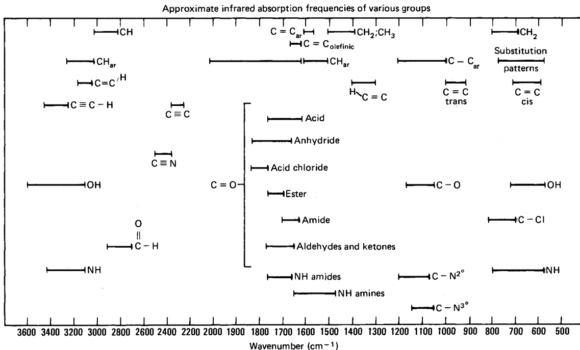
Fig. 120 The author's only IR correlation chart.
