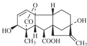
Gibberellin A_3
