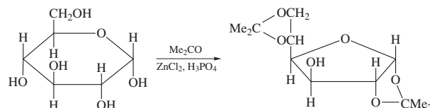
FIGURE 14 1,2:5,6-diisopropylidene D-glucopyranose. Formed by reaction of D-glucose with acetone in the presence of a suitable catalyst. The furanose product dominates due to kinetic control of the reaction.
