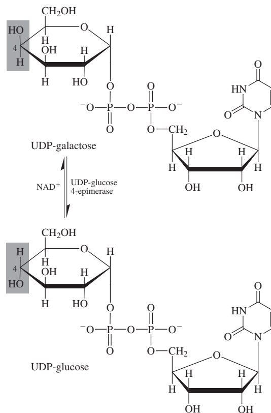
FIGURE 17 Biosynthesis of D-galactose by epimerization of uridine diphosphoglucose.
