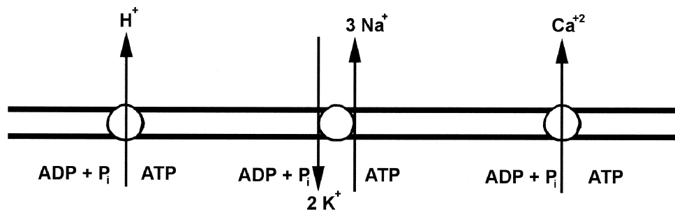
FIGURE 12 Some ion pumps in the plasma membrane. The Na^+/K^+ -ATPase of animal cells uses the energy of ATP hydrolysis to move three Na^+ ions out of the cells and two K^+ ions in, which results in the generation of ion gradients and a membrane potential. Plant, yeast, and fungal cells do not have a Na^+/K^+ -ATPase, but instead have a H^+ -ATPase, as the electrogenic pump. The plasma membrane also contains a Ca^{2+} -ATPase that pumps Ca^{2+} out of cells to help keep the intracellular Ca^{2+} concentration low.
