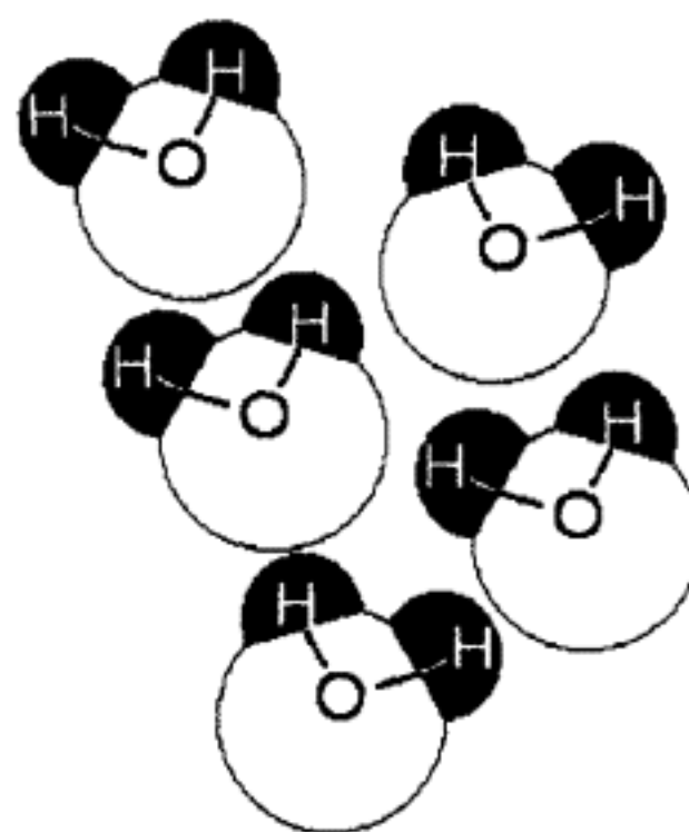
Figure 1.8. Hydrogen bonding
