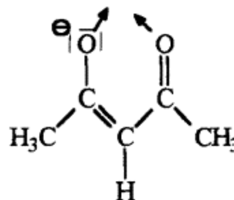
Acetylacetonate
