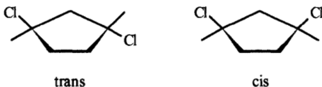
Figure 3.10. Trans and cis- 1,3-cyclopentane
