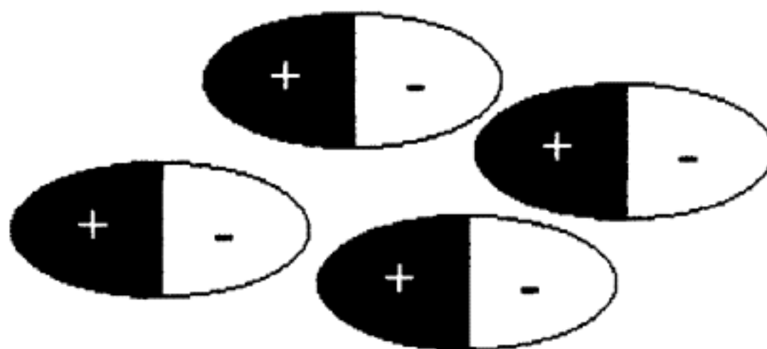
Figure 1.6. Dipole-dipole attraction
