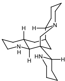
Ormosanine
