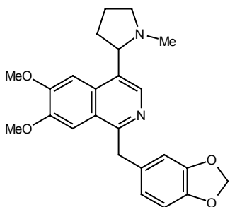
Macrostromine
