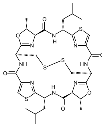
Ulithiacyclamide
