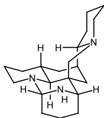
Panamine
