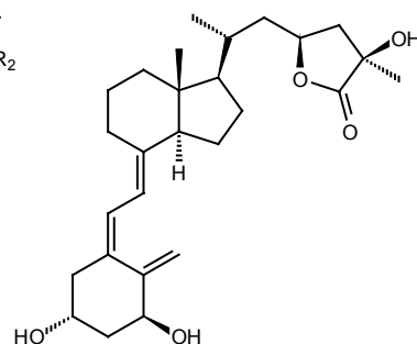
Calcitriol Lactone
