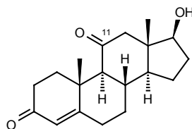
11-Ketotestosterone
