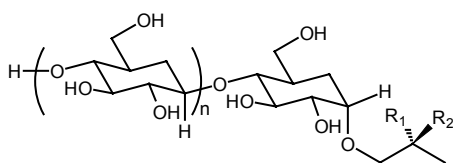
Rhynchosporosides
