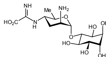
Kasugamycin
