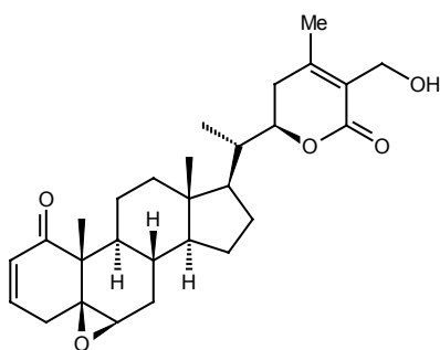
Jaborosalactone A
