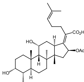
Fusidic Acid
