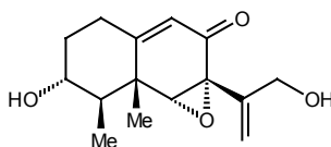
Phomenone
