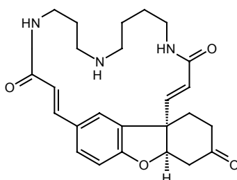
Lunarine
