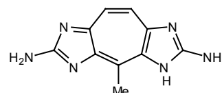
Parazoanthoxanthin A
