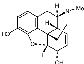
Morphine (Gates, 1956)
