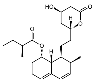
(+)-Compactin
