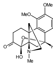
Metaphanine
