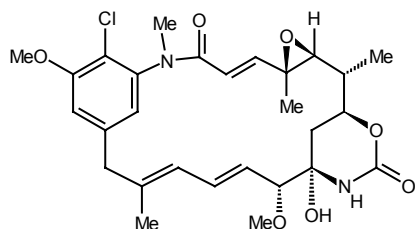
Maysine
