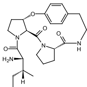
(-)-Dihydrozizyphin G
