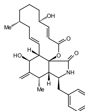
Cytochalasin B
