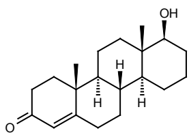
D-Homotestosterone
