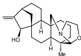
Garryine
