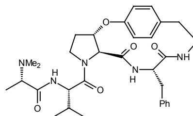
Dihydromauritine A
