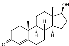
Testosterone
