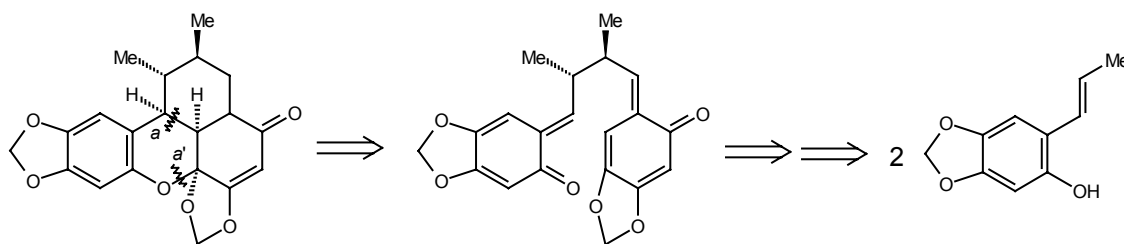
Carpanone (123)
