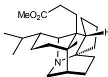
(+)-Methyl Homodaphniphyllate
