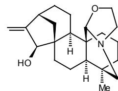
Veatchine
