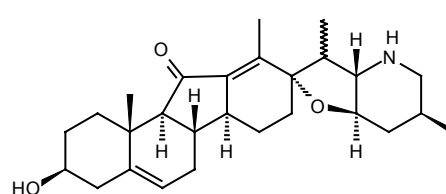
Jervine
