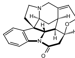
Strychnine (Woodward, 1954)
