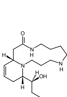
Palustrine
