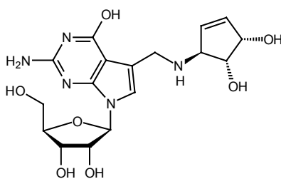
(+)-Nucleoside Q
