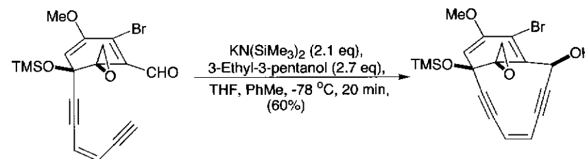
Scheme 8.5 Acetylenic anion ring-closure in Danishefsky's calicheamcinone synthesis.
