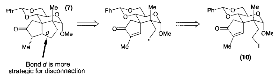
Scheme 10.3 Free radical retrosynthetic disassembly of bond d in 7 . Advantages: it does not necessitate the construction of a functionalised medium-sized ring. It forms the bicyclooctane ring system by a favourable 5-exo-trig pathway. Conformational and steric bias will allow the stereochemistry of the methyl \alpha to the ketone to be controlled.
