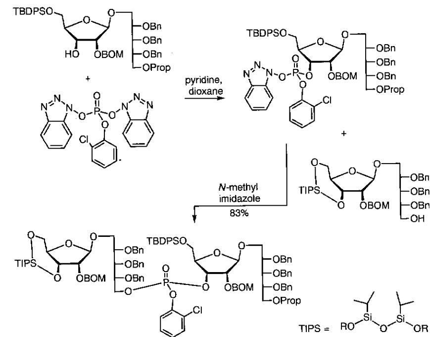
Scheme 3.17 Phosphorylation by phosphotriester method.
