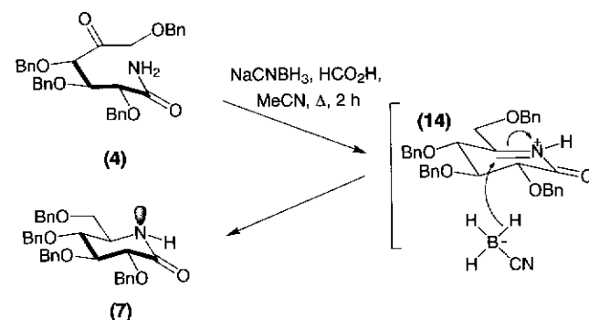
Scheme 9.3.
