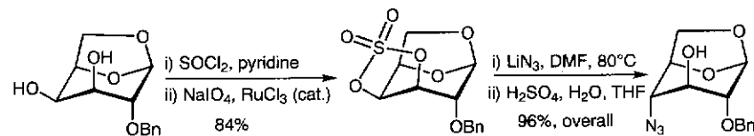
Scheme 3.10 (Continued).
