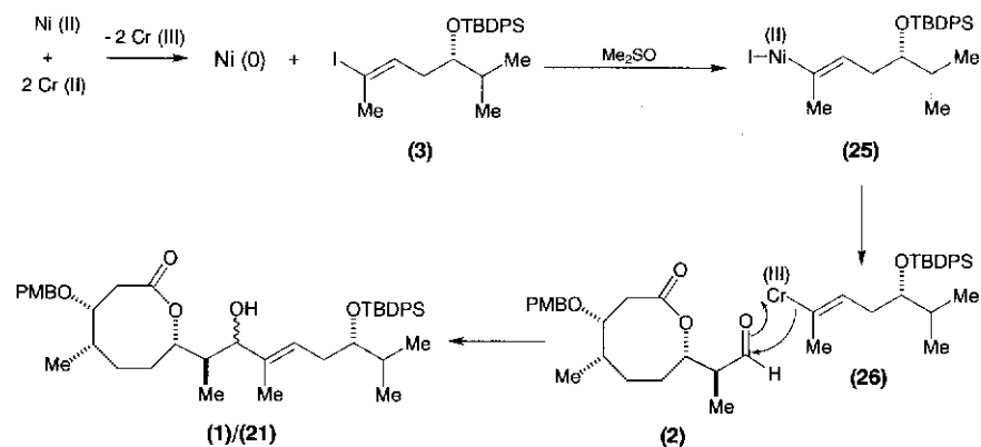
Scheme 13.6.
