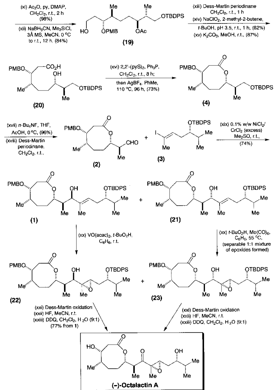
Scheme 13.4 (Continued).
