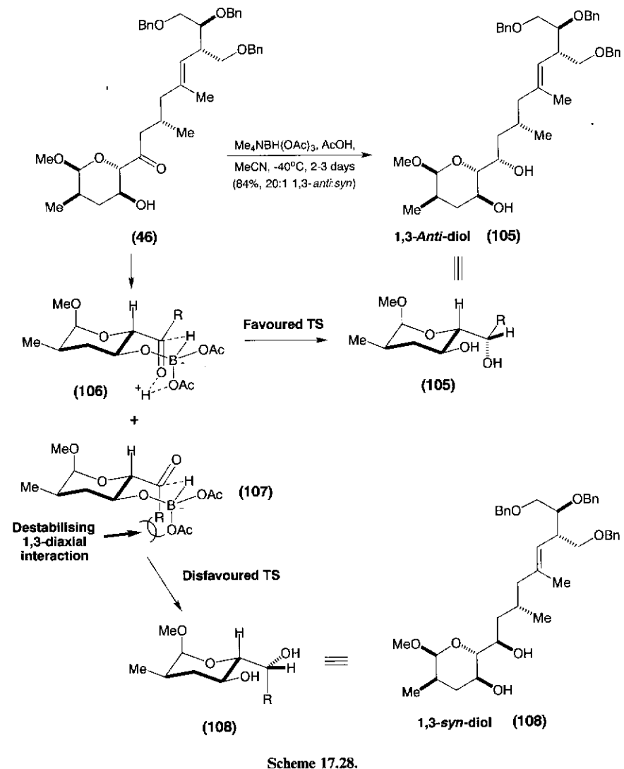
Scheme 17.28.
