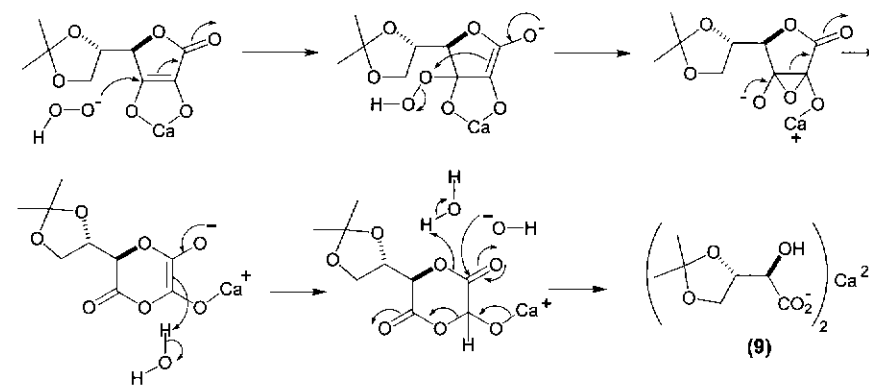
Scheme 6.5.
