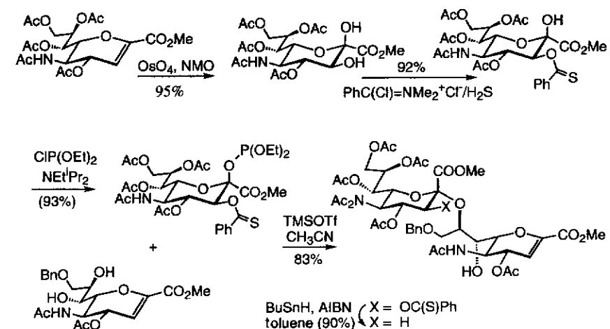
Scheme 4.12 (Continued).
