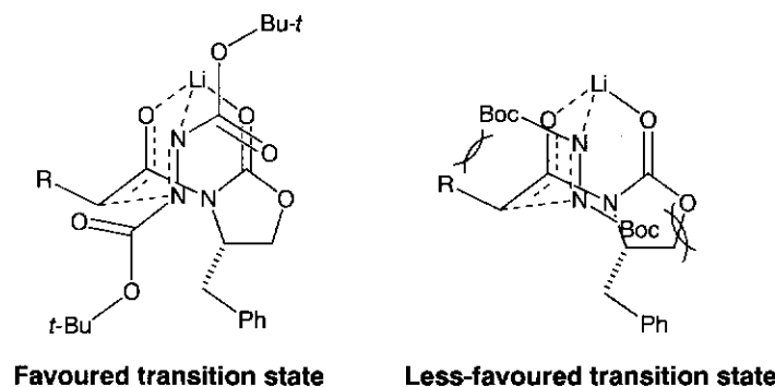
Scheme 18.3.
