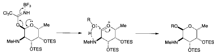
Scheme 8.13.
