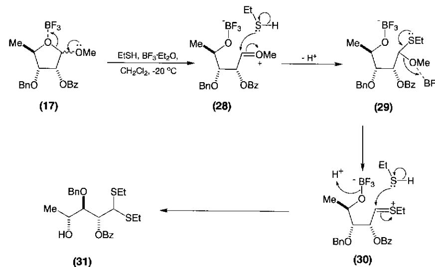
Scheme 12.9.
