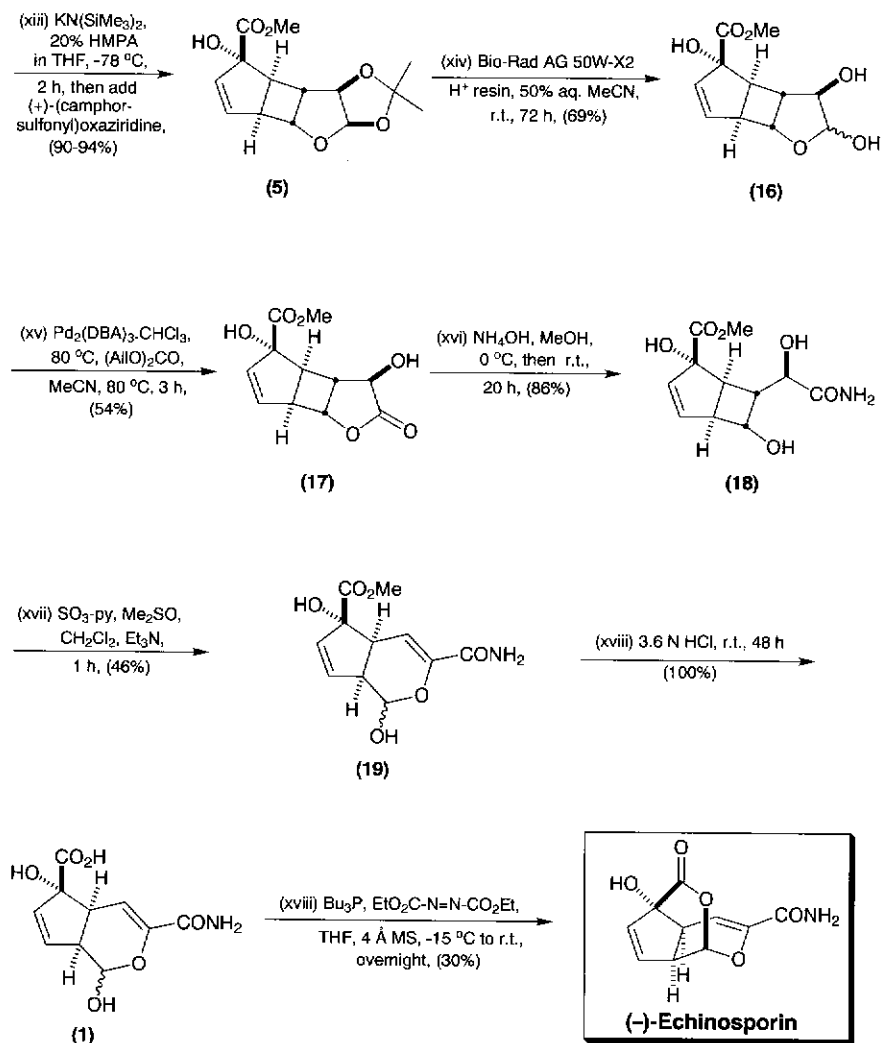
Scheme 6.3 (Continued).
