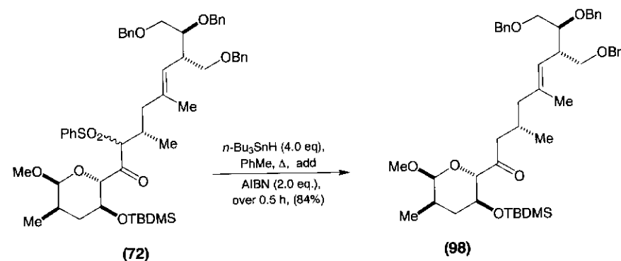
Scheme 17.25.
