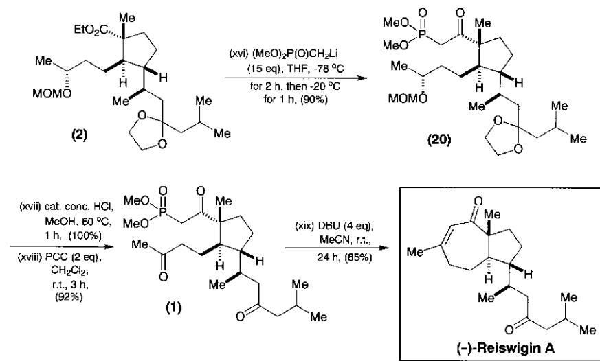
Scheme 12.6 (Continued).
