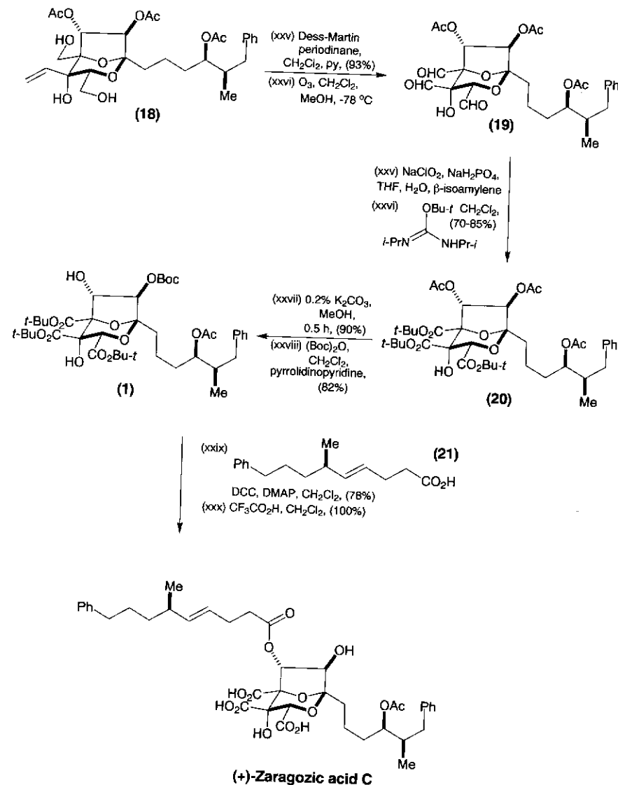
Scheme 7.4 (Continued).
