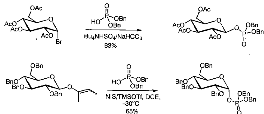
Scheme 3.20 Anomeric phosphorylation.
