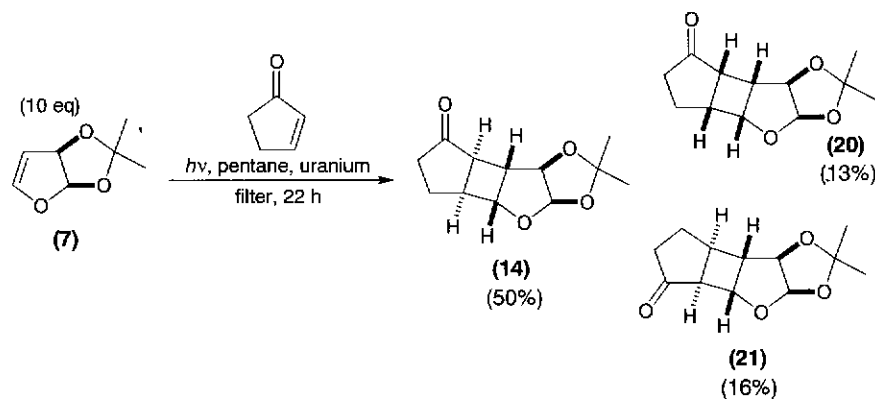
Scheme 6.4 [2+2]-Photocycloaddition reaction.
