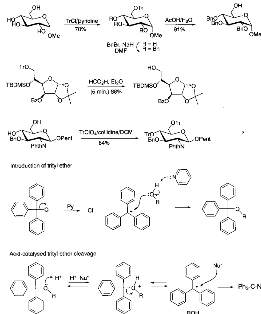
Scheme 2.8 Tritylation of sugar hydroxyls.
