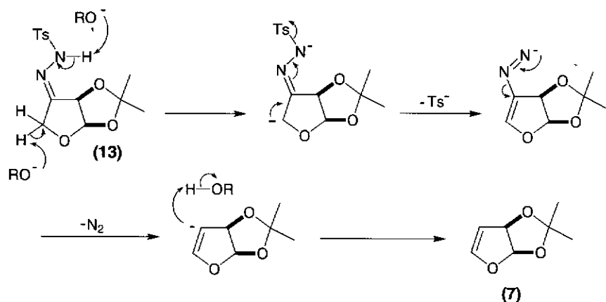
Scheme 6.6.
