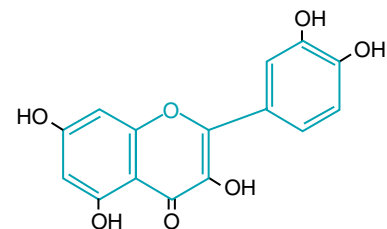
A flavonoid
