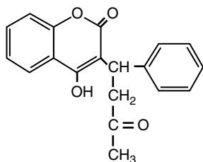
Warfarin
