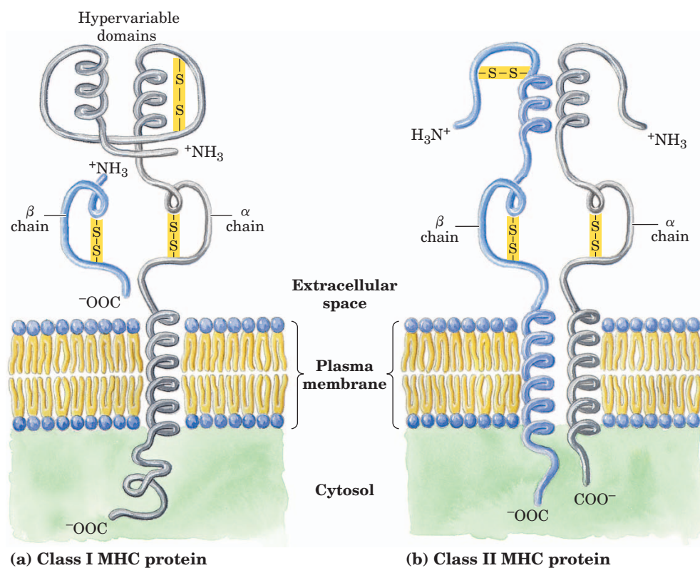
FIGURE 5-21 MHC proteins.
