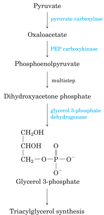
FIGURE 21-21 Glyceroneogenesis. The pathway is essentially an abbreviated version of gluconeogenesis, from pyruvate to dihydroxyacetone phosphate (DHAP), followed by conversion of DHAP to glycerol 3-phosphate, which is used for the synthesis of triacylglycerol.
