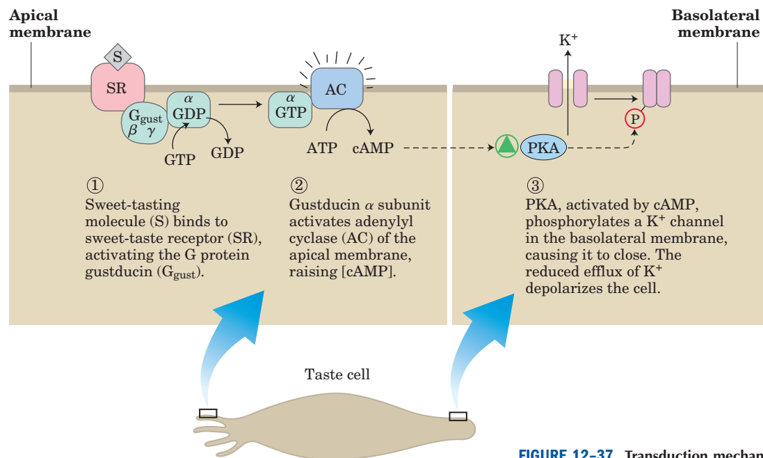
FIGURE 12-37 Transduction mechanism for sweet tastants.
