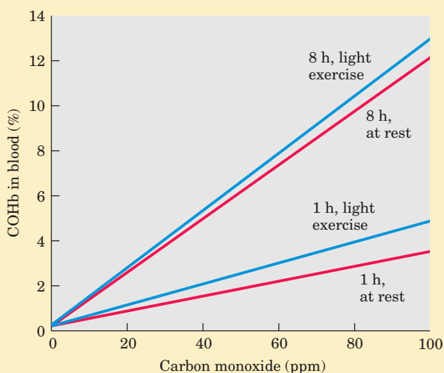
FIGURE 1 Relationship between the levels of COHb in blood and the concentration of CO in the surrounding air. Four different conditions of exposure are shown, comparing the effects of short versus extended exposure, and exposure at rest versus exposure during light exercise.
