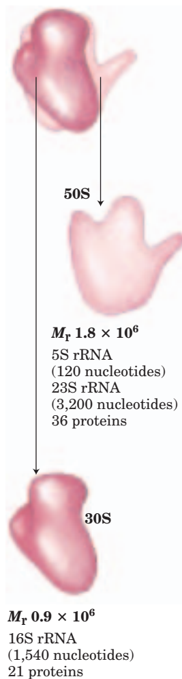
Bacterial ribosome 70S M_r 2.7 \times 10^6
