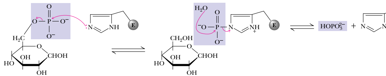
FIGURE 23.9 • The glucose-6-phosphate reaction involves formation of a phosphate-bound intermediate.
