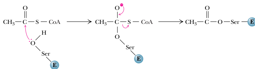
FIGURE 25.10 • Acetyl units are covalently linked to a serine residue at the active site of the acetyl transferase in eukaryotes. A similar reaction links malonyl units to the malonyl transferase.
