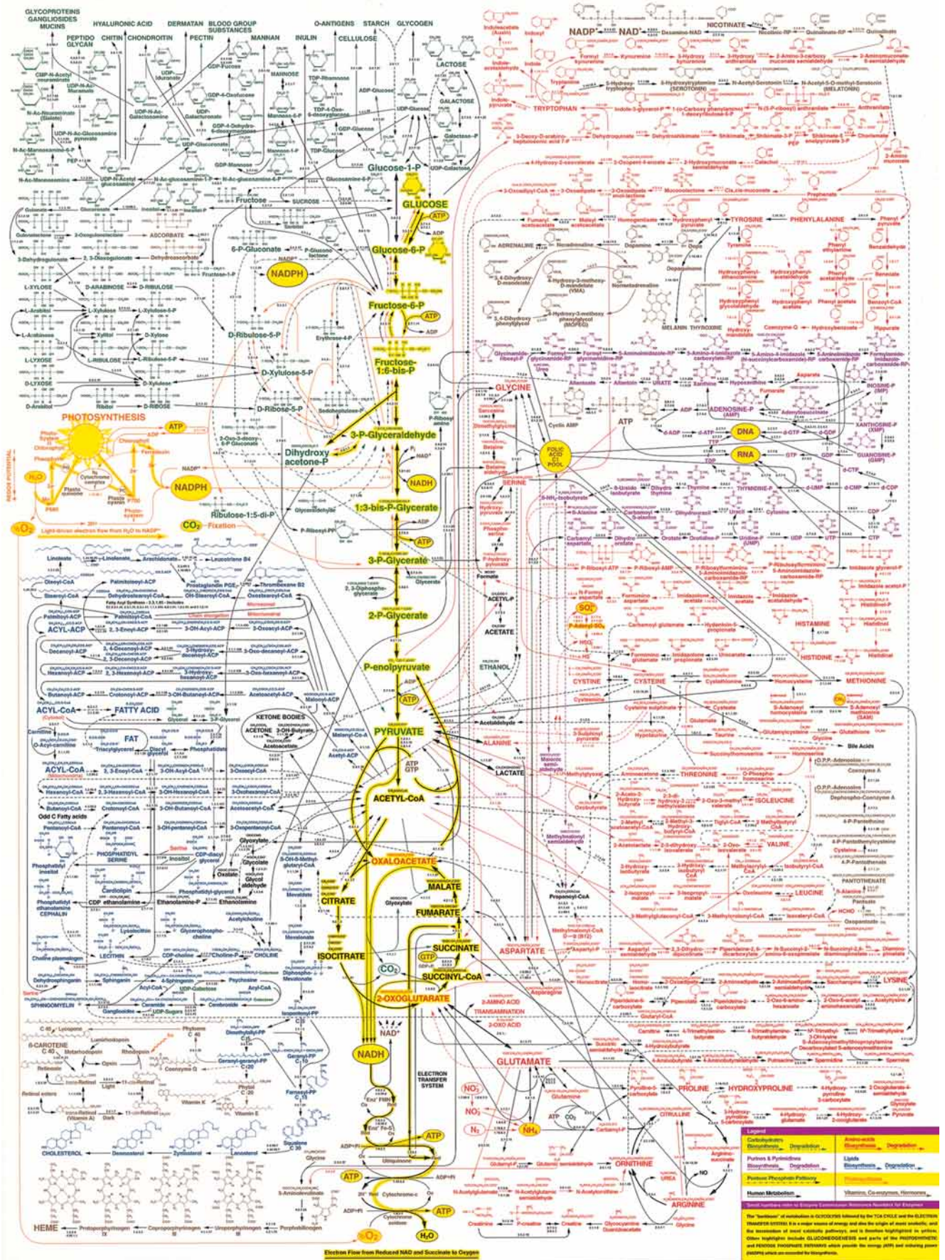
Electron Flow from Reduced NAD and Succinate to Oxygen
