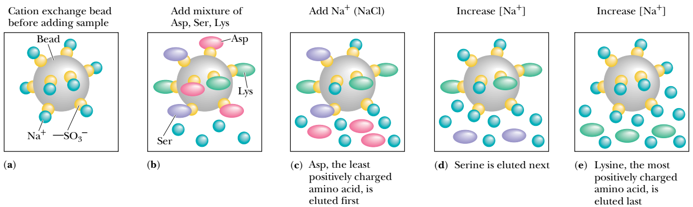
FIGURE 4.19 • Operation of a cation exchange column, separating a mixture of Asp, Ser, and Lys. (a) The cation exchange resin in the beginning, \text{Na}^+ form. (b) A mixture of Asp, Ser, and Lys is added to the column containing the resin. (c) A gradient of the eluting salt (e.g., NaCl) is added to the column. Asp, the least positively charged amino acid, is eluted first. (d) As the salt concentration increases, Ser is eluted. (e) As the salt concentration is increased further, Lys, the most positively charged of the three amino acids, is eluted last.
