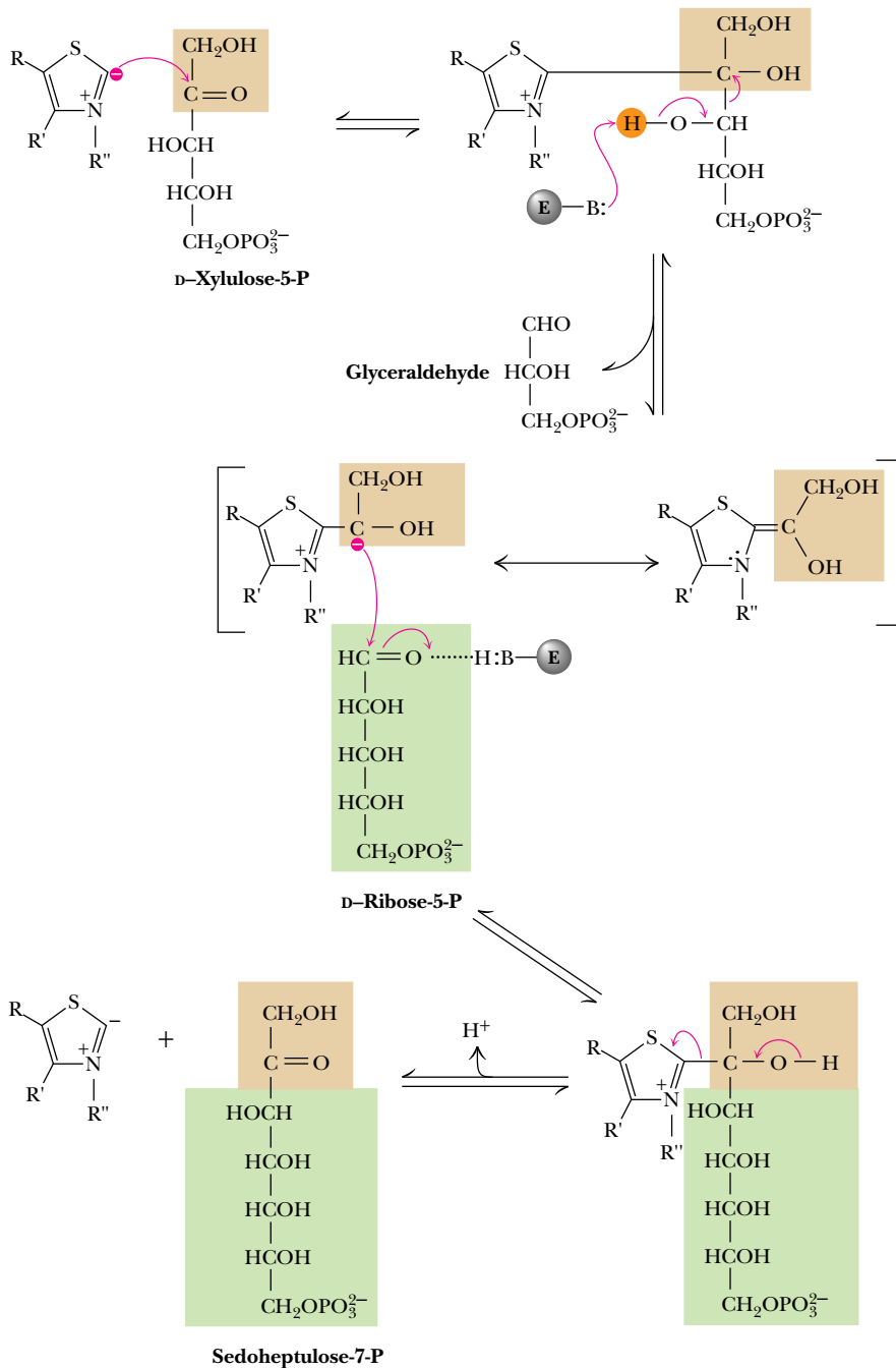
FIGURE 23.34 • The mechanism of the thiazolium-dependent transketolase reaction. In the transketolase reaction, the group transferred in the transketolase reaction might best be described as an acyl group, whereas the transferred group in the transaldolase reaction is actually a ketol. Despite this irony, these names persist for historical reasons.
