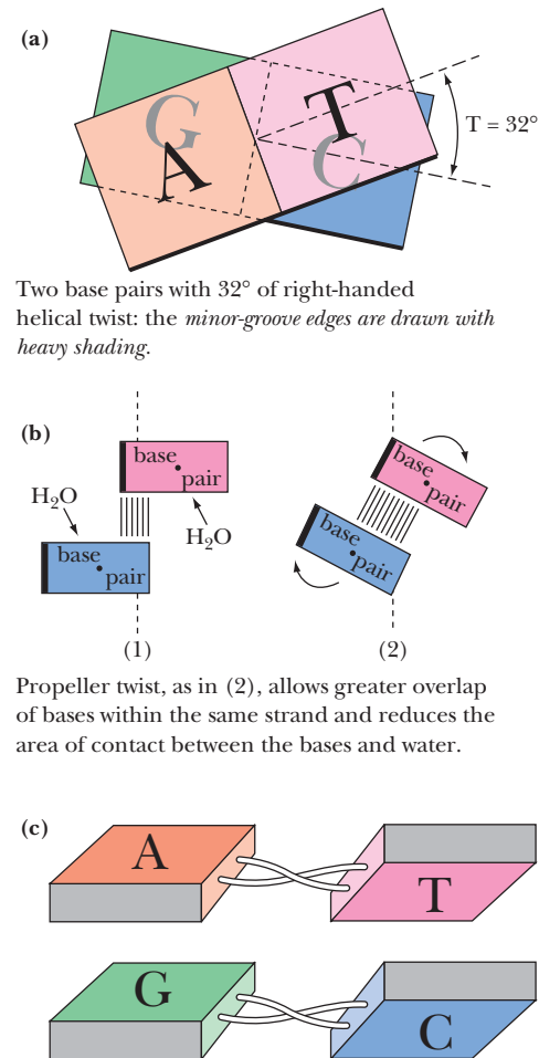
FIGURE 12.11 • The bases in a base pair are not directly across the helix axis from one another along some diameter but rather are slightly displaced. This displacement, and the relative orientation of the glycosidic bonds linking the bases to the sugar–phosphate backbone, leads to differently sized grooves in the cylindrical column created by the double helix, the major groove and the minor groove, each coursing along its length.
