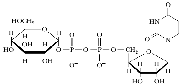
Uridine diphosphate glucose (UDPG)
