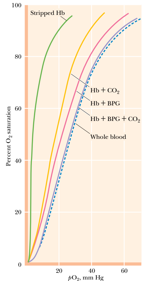
FIGURE 15.35 • Oxygen-binding curves of blood and of hemoglobin in the absence and presence of CO 2 and BPG. From left to right: stripped Hb, Hb + CO 2 , Hb + BPG, Hb + BPG + CO 2 , and whole blood.
