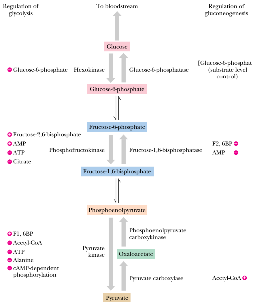
FIGURE 23.11 • The principal regulatory mechanisms in glycolysis and gluconeogenesis. Activators are indicated by plus signs and inhibitors by minus signs.
