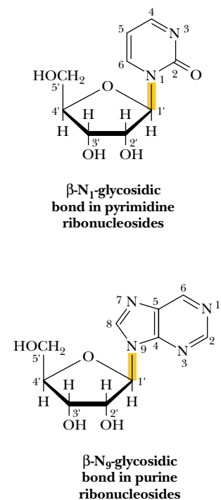
FIGURE 11.10 • \beta -Glycosidic bonds link nitrogenous bases and sugars to form nucleosides.
