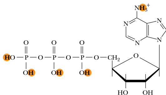
Color indicates the locations of the five dissociable protons of ATP.
