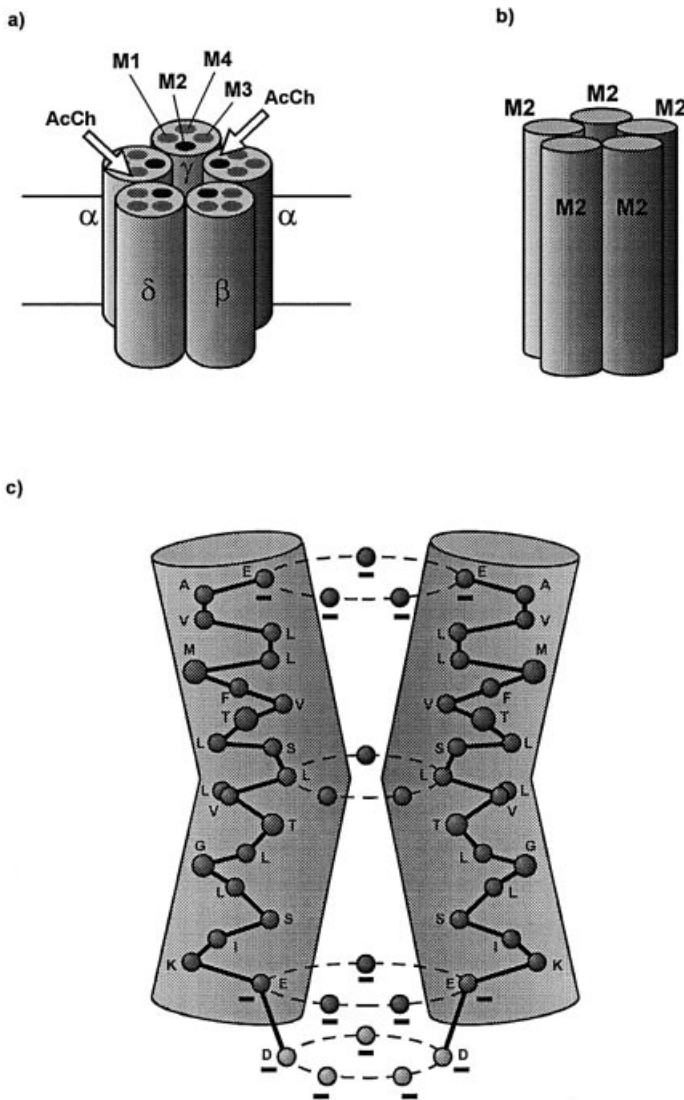
Fig. 16.12. Subunit structure of the acetylcholine receptor. a) The acetylcholine receptor has the subunit structure \alpha_2\beta\gamma\delta . The four transmembrane elements M1–M4 are shown for the \gamma subunit. The binding sites for acetylcholine (ACh) are located on the \alpha -subunits. b) It is assumed that the inner wall of the ion pore is formed by M2 helices of the five subunits. c) Postulated configuration of the M2 helices in the narrowest region of the ion channel. In the closed state, five leucine residues (one per subunit) lie in the ion channel and hinder passage of ions. Above and below the block, there are negatively charged residues that serve as prefilters for ion passage.
