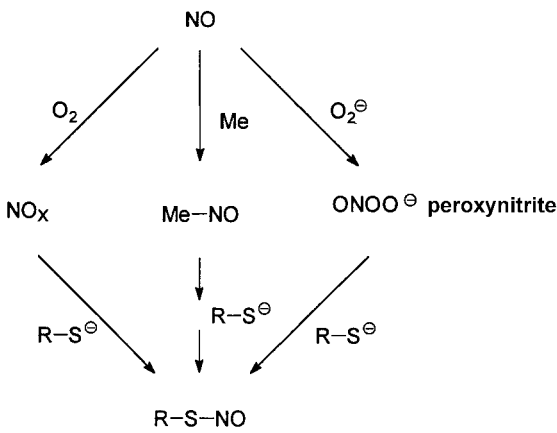
Fig. 6.13. Reactions of NO in biological systems. NO reacts in biological systems primarily with \text{O}_2 , with the superoxide anion \text{O}_2^- and with transition metals (Me). The products of the reaction, -\text{NO}_x , metal-NO adducts (Me-NO) and peroxynitrite ( \text{OONO}^\ominus ) react further by nitrosylation of nucleophilic centers. In the cell, these are especially -\text{SH} (or thiolate- \text{S}^- ) groups of peptides and proteins ( \text{RS}^- ).
