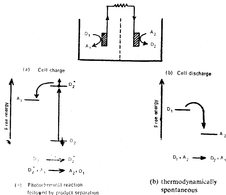
Figure 9.10 Photoelectrochemical cell: (a) Photochemically charged; (b) Spontaneously discharged producing electrical power. A_1 , A_2 , D_1 , D_2 are oxidized and reduced forms of dyes 1 and 2 respectively.
