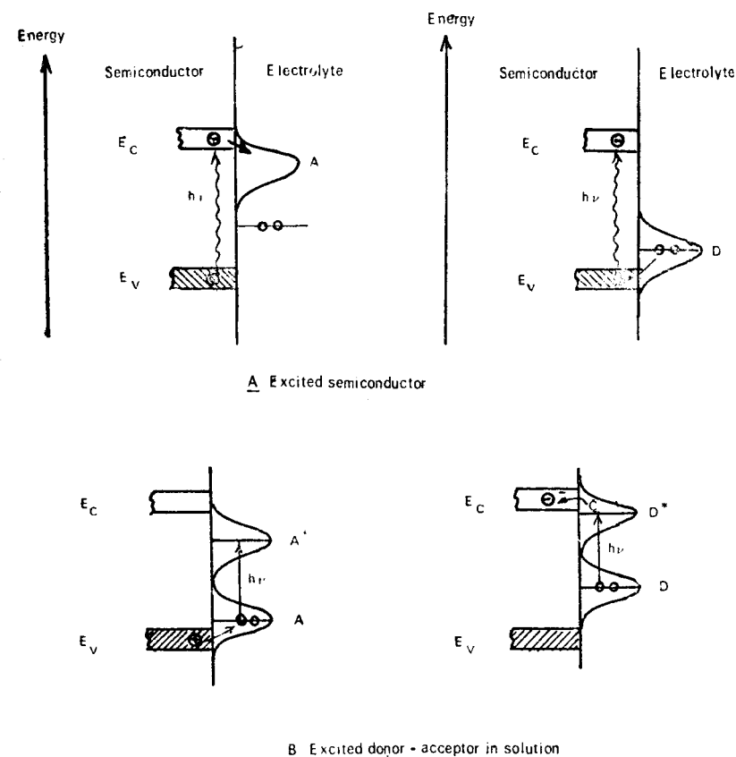
Figure 9.7 Energetics of donor-acceptor property in semiconductor-solution interface: (A) Photoexcited semiconductor: electron injection to the solution; hole injection; (B) Photoexcited donor or acceptor in solution: hole injection; electron injection to SC.
