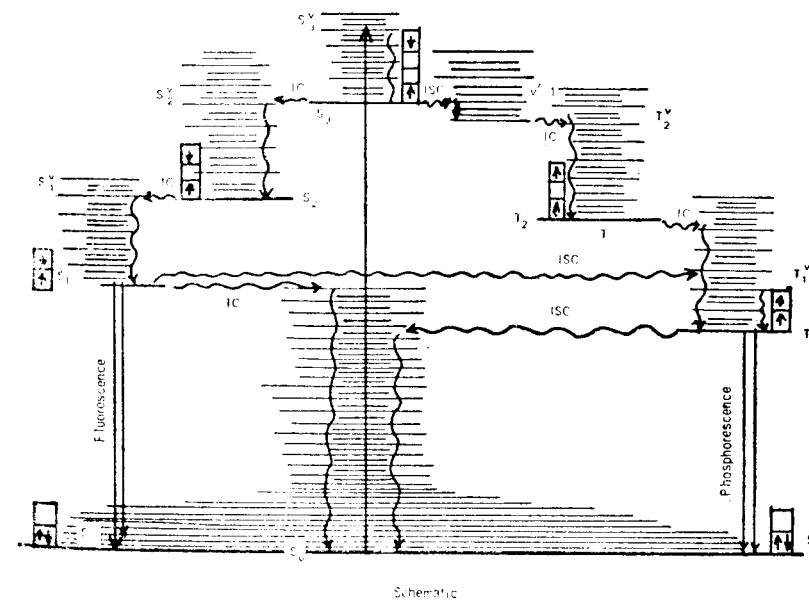
Figure 5.1 Jablonski diagram for photophysical pathways S_n, S_n^v = n th singlet energy state and vibronically excited state T_n, T_n^v = n th triplet energy state and vibronically excited state IC = internal conversion, ISC = intersystem crossing F = fluorescence emission, P = phosphorescence emission.
