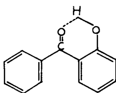
o-hydroxy benzophenones (R=H, Me, C 8 H 17 , C 10 H 21 etc.)
