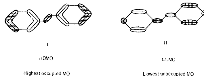
Figure 7.6 Nodal properties of HOMO and LUMO of stilbene.
