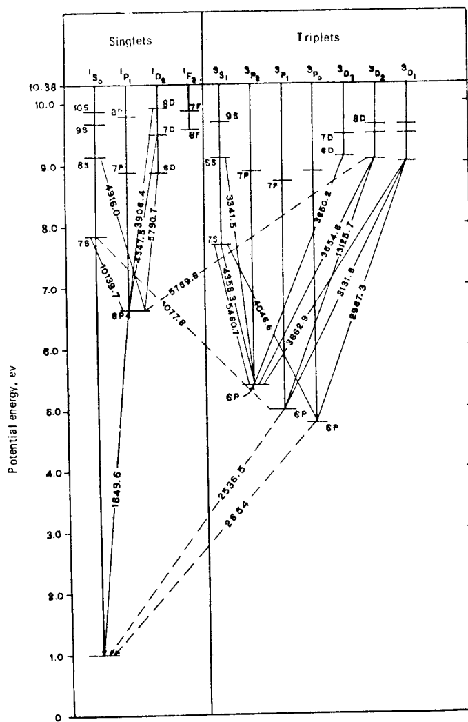
Figure 2.8 Grotrian diagram for Hg atom. Wavelengths are in Å units.
