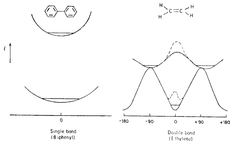
Figure 4.20 Variation of potential energy function for ground and excited states of biphenyl (single bond) and ethylene (double bond).
