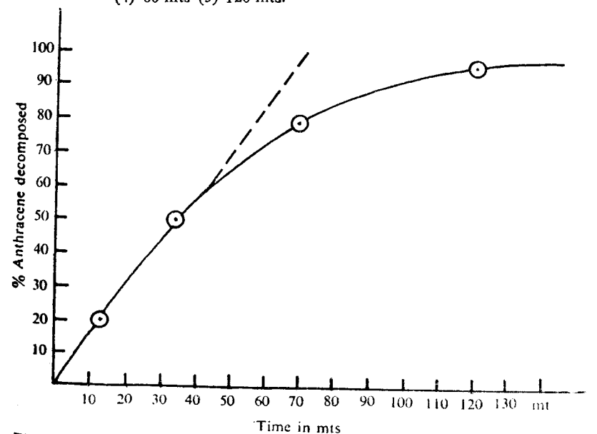
Fig. 11.2 Rate of disappearance of anthracene due to photochemical reaction. The dotted line gives the initial rate.
