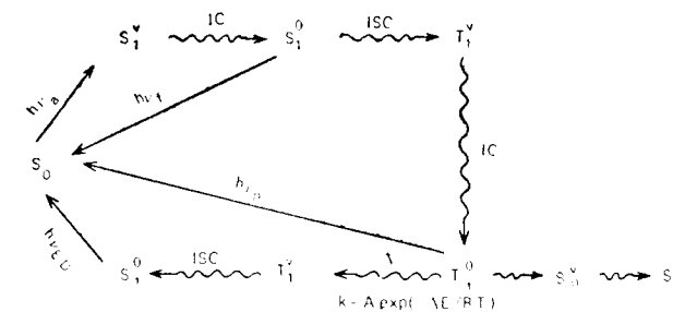
Figure 5.11 E-type delayed fluorescence pathways indicating possibility of emission from each relaxed state.
