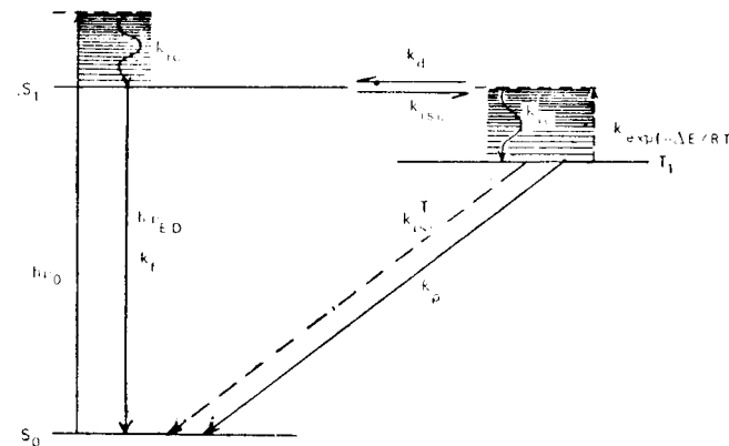
Figure 5.10 Jablonski diagram for E-type delayed fluorescence.
