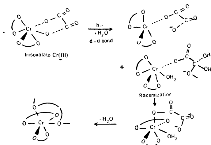
Figure 8.17 Photoracemization in Pt(III) complex.
