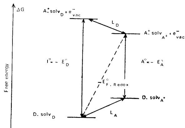
Figure 9.6 Free energy relations in defining electron donor-acceptor levels in solution of an electrolyte.
