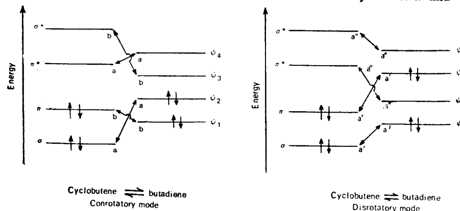
Figure 8.8 Reactant-product orbital correlation diagram for cyclobutene \rightleftharpoons butadiene transformation for (a) conrotatory and (b) disrotatory modes.
