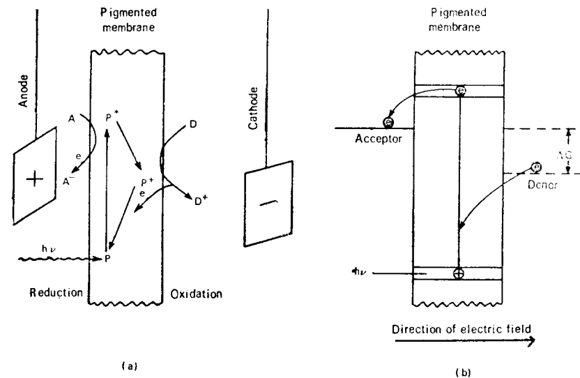
Figure 9.4 Membrane model for electron transfer reaction in photosynthetic cycle with acceptor A and donor D on either side of the membrane (a) P, \text{P}^* , \text{P}^+ are respectively normal state electronically excited state and oxidised form of pigment molecule. (b) Illustrating energy levels of ground and excited states of pigment molecule in the membrane and acceptor and donor molecules in solution. \Delta G = nFE is theoretically available electrochemical free energy; e^- = electron, + = positive hole.
