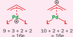
Pd \pi -allyl cation complex
