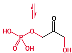
dihydroxyacetone-3-phosphate
