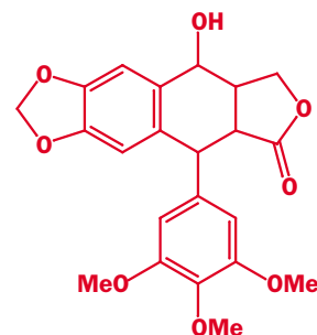
the anti-cancer compound podophyllotoxin
