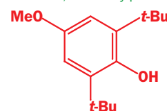
'butylated hydroxyanisole', BHA
