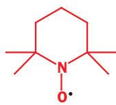
TEMPO TEtraMethylPiperidine N-Oxide m.p. 36–38°C
