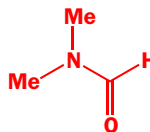
DMF (DiMethylFormamide)
