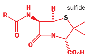
penicillin family of antibiotics
