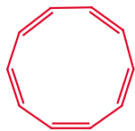
all- cis -[10]annulene
