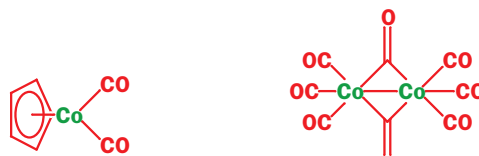
18-electron complex of Co(0)
