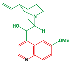
quinine
