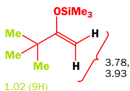
silyl enol ether
