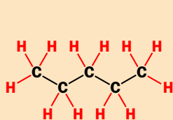
a chain
