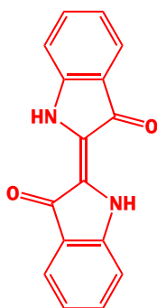
indigo the colour of blue jeans
