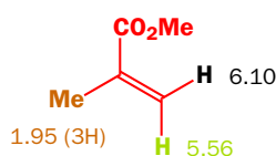
unsaturated ester
