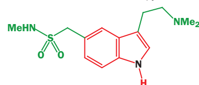
sumatriptan: for treatment of migraine
