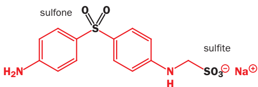
dapsone—water-soluble 'pro-drug' for leprosy
