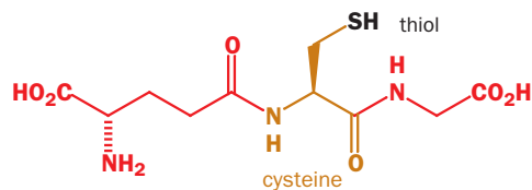
glutathione: scavenger of toxic oxidants
