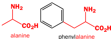
alanine
