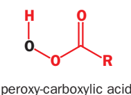
peroxy-carboxylic acid
