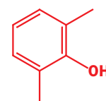
2,6-dimethylphenol
