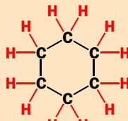
a ring
