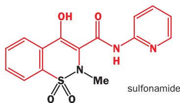
Pfizer's piroxicam or Feldene
