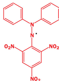
violet crystals
