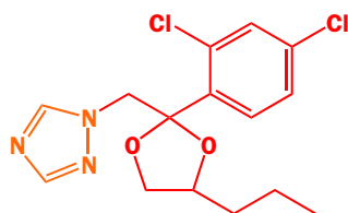
propiconazole a triazole fungicide
