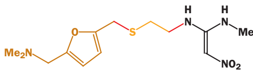
ranitidine—GlaxoWellcome's Zantac
