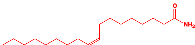
a sleep-inducing fatty acid derivative cis -9,10-octadecenoamide
