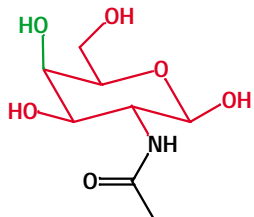
N -acetyl-galactosamine
