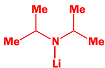
LDA Lithium Di-isopropylAmide
