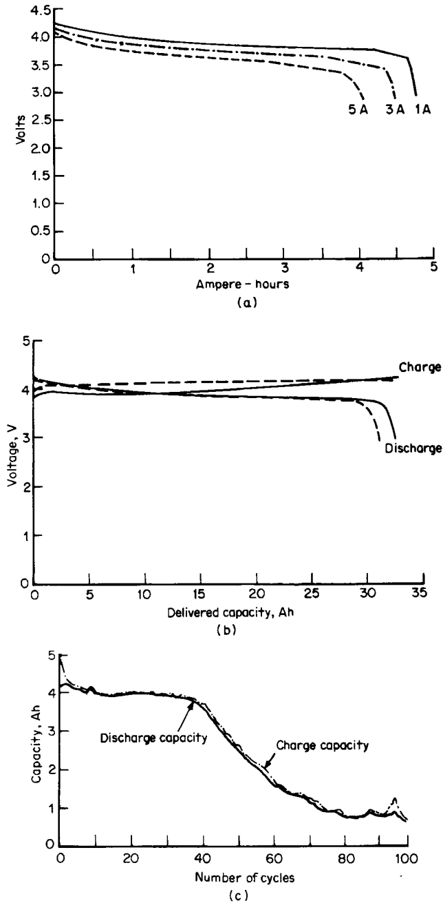
FIGURE 34.19 (a) Discharge characteristics of a 5-Ah \text{Li}/\text{Li}_2\text{CoO}_2 D-size battery at 20°C. (Delivered specific energy at 1.0 A, 70 Wh/lb.) (b) Effect of charging rates on discharge performance of 30-Ah \text{Li}/\text{Li}_2\text{CoO}_2 battery at 20°C. - - -, constant potential at 4.20 V [current limit at 5.0 mA/cm 2 ( C/2 )]. —, constant current at 1.0 mA/cm 2 ( C/10 ). Discharge rate at C/6 . (c) Cycle life characteristics of a \text{Li}/\text{Li}_2\text{CoO}_2 D-size battery. Charge at 300 mA, 4.3 V. Discharge at 3 A, 3.0 V. (From Alliant Technologies.).
