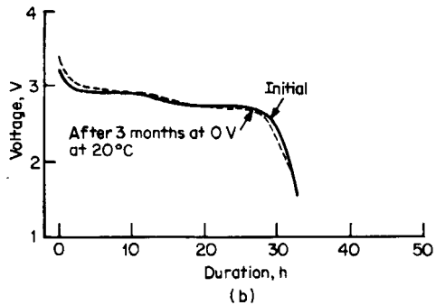
FIGURE 34.42 Overcharge and overdischarge characteristics of LiAl/V 2 O 5 coin-type battery (VL2020 size): (a) overcharge characteristics, (b) overdischarge characteristics (charge at 200 Ω for 48 h, discharge at 3 kΩ). (From Panasonic Division of Matsushita Electric Corp. of America.)
