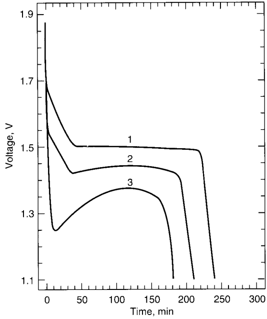
FIGURE 33.5 Typical discharge curves of HR-5 silver zinc battery at C/3 (2-A) rate. Curve 1— 25^{\circ}\text{C} ; curve 2— 0^{\circ}\text{C} ; curve 3— -18^{\circ}\text{C} .
