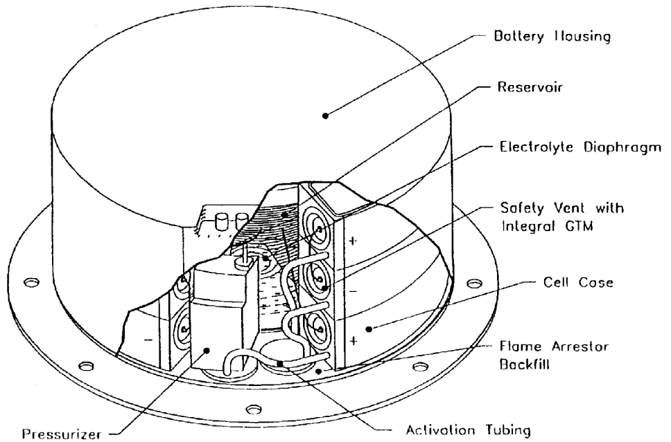
FIGURE 20.9 Design of reserve Li/Li x CoO 2 battery for Hand-emplaced Wide Area Munitions (HWAM). (Courtesy of Alliant Techsystems, Inc.)
