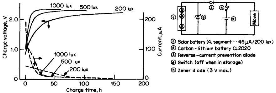
FIGURE 34.44 Charge characteristics of a carbon-lithium coin-type battery (CL2020 size) with solar batteries. (From Panasonic Division of Matsushita Electric Corp. of America.)
