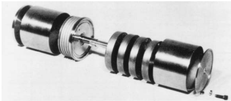
FIGURE 20.7 Pictorial view of 20-Ah Li/SO 2 multicell battery.
