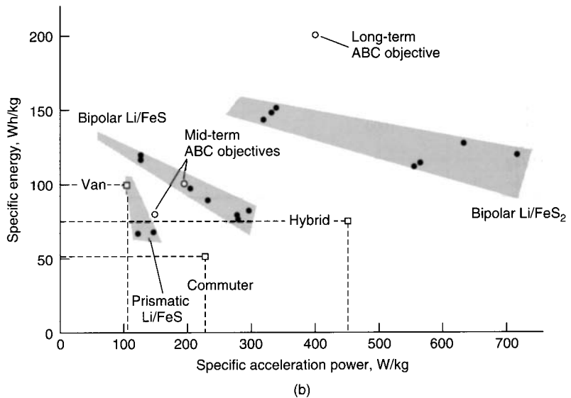
FIGURE 41.15 Energy vs. acceleration power projections for fully operational Li-Al/ \text{FeS}_2 battery designs based on laboratory cell data. (a) Volumetric. (b) Gravimetric. (From Henriksen et al. ) 15
