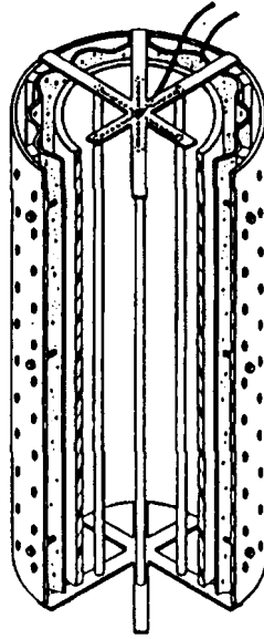
FIGURE 38.43 Schematic of concentric cylinder configuration of seawater cell. The output cylinder is comprised of porous fiberglass coated with an antifoulant. The corrugated structure is the air cathode, which is exterior to the magnesium anode. The entire structure is open to the seawater electrolyte. (Courtesy of Westinghouse Corp.)
