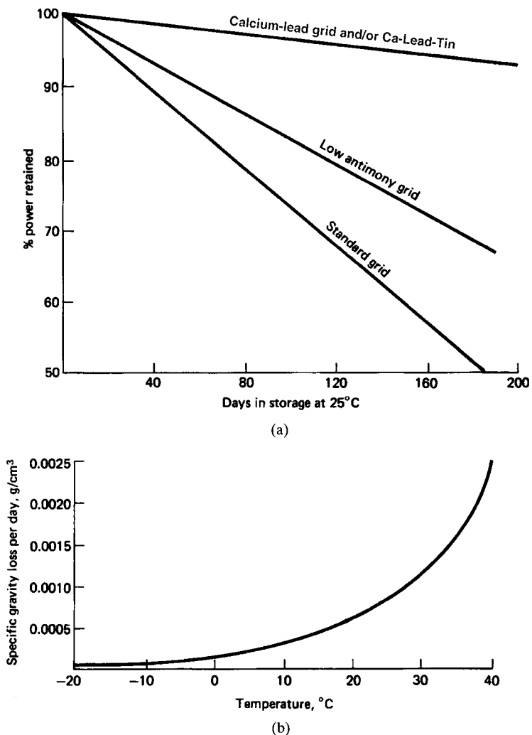
FIGURE 23.6 (a) Capacity retention during stand or storage at 25°C. (From Sabatino. 9 ) (b) Loss of specific gravity per day with temperature of a new, fully charged lead-acid battery with 6% antimonial lead grids. (From Ref. 10.)
