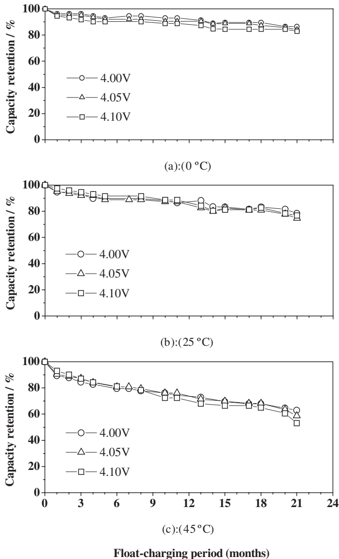
FIGURE 35.85 Capacity retention of wound ICP22846 C/LiCoO 2 Li-ion cells float charged at 0°C, 25°C or 45°C for up to 21 months at 4.0 V, 4.05 V or 4.1 V. (Courtesy of Japan Storage Battery Co., Ltd.)
