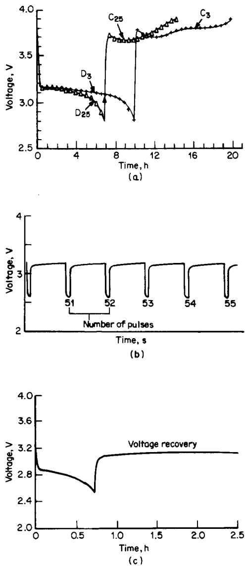
FIGURE 34.32 (a) Discharge/charge behavior of a Li/LiAlCl 4 · 6SO 2 C-size battery at 1 mA/cm 2 . Voltage limits; 2.8–4.0 V. Line—battery, symbols (Δ)—cathode vs. ref. (b) High-rate pulse discharge of a Li/LiAlCl 4 · 6SO 2 C-size battery. Pulse rate at 20 mA/cm 2 for 20 s. Rest period for 180 s. (c) Discharge characteristics and voltage recovery (without load) of a Li/LiAlCl 4 · 6SO 2 C-size battery at -20°C. Discharge at 3.2 mA/cm 2 . (From Yardney Technical Products, Inc.)
