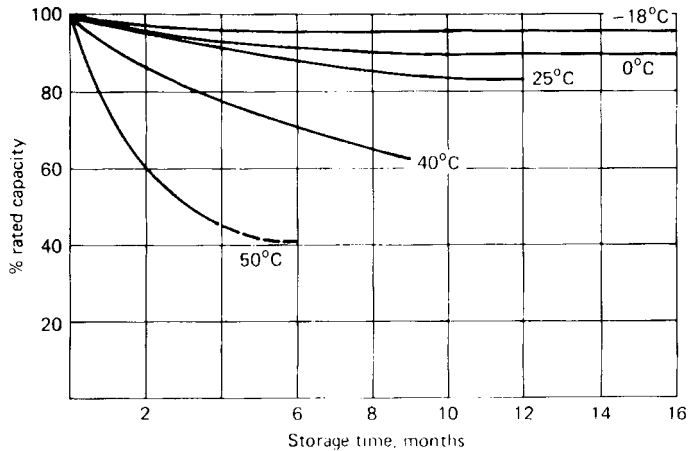
FIGURE 18.14 Wet (activated) storage of zinc/silver oxide primary batteries. (Courtesy of Eagle-Picher Industries.)
