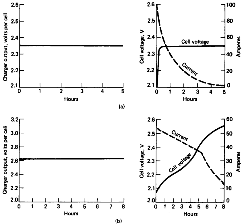
FIGURE 23.49 Typical charger and battery characteristics for constant-potential charging of lead-acid batteries. (a) Constant-potential charging. (b) Modified constant-potential charging. (From Ref. 10.)
