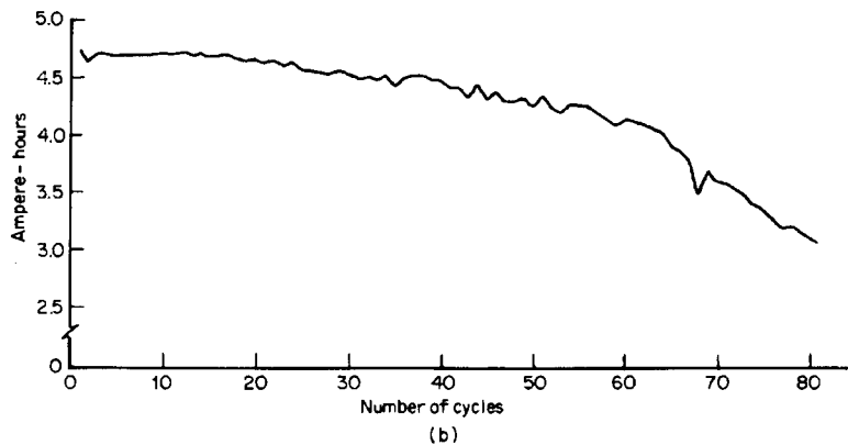
FIGURE 34.20 (a) Discharge characteristics of a Li/Li x NiO 2 D-size battery. Charge at 0.3 A to 4.1 V. (b) Cycle life characteristics of a Li/Li x NiO 2 D-size battery. Discharge at 2 A to 2.8 V. Charge at 0.4 A to 4.1 V. Taper to 0.1 mA. (From Ref. 42.)
