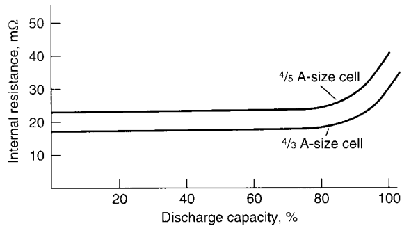
FIGURE 29.9 Internal resistance vs. discharge capacity of sealed cylindrical nickel-metal hydride cells.
