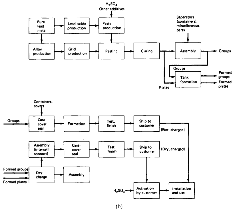
FIGURE 23.10 (a) Chemical compounds and process parameters in production of SLI batteries. (b) Production flow sheet for lead-acid batteries.
