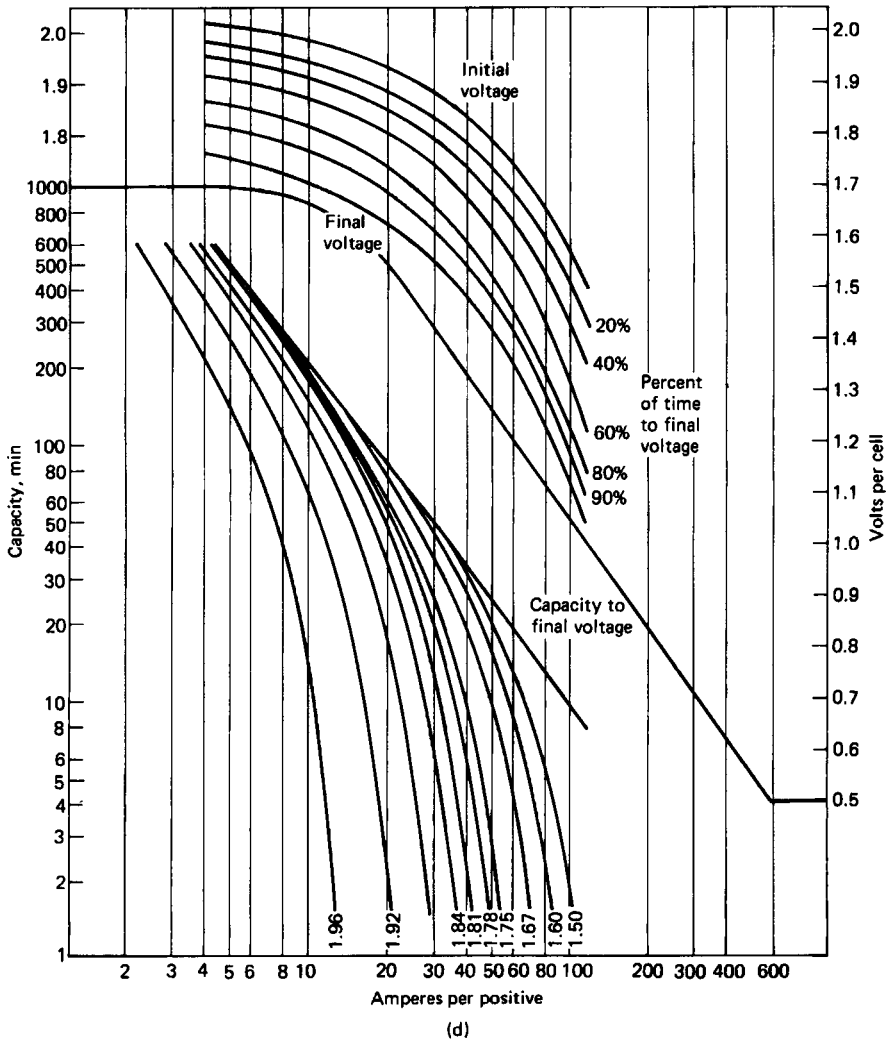
FIGURE 23.40 (d) Manhex plate, 40 Ah at 8-h rate; 197-mm height, 197-mm width, 11.2-mm thickness. (Courtesy of Energys, Inc.) (Continued).
