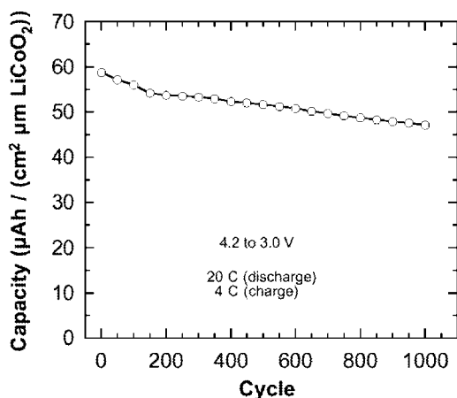
FIGURE 35.114 Capacity of a LiCoO 2 battery with an in-situ electroplated lithium negative electrode, normalized to 1 cm 2 and 1 µm LiCoO 2 . The battery was cycled between 4.2 V and 3.0 V at 25°C, charged at the 4C rate and discharged at the 20C rate. (Courtesy of Oak Ridge National Laboratory.)
