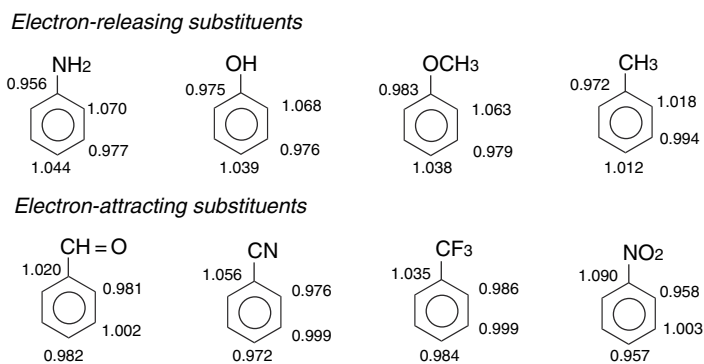
Fig. 9.5. Total \pi -electron density for some substituted benzenes. From HF/STO-3G calculations.
