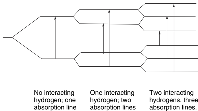
Fig. 11.1. Hyperfine splitting in ESR spectra.
