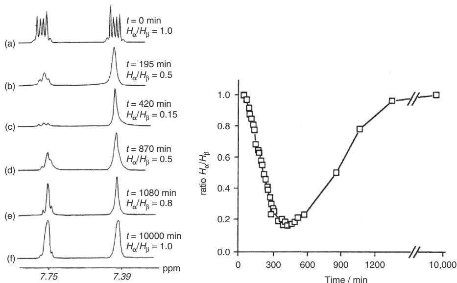
Fig. 9.9. Changes in ^1\text{H} -NMR spectrum of naphthalene heated with \text{CF}_3\text{CO}_2\text{D} in the presence of (\text{CF}_3\text{CO}_2)_2\text{O} and \text{Al}(\text{O}_2\text{CCF}_3)_3 (left). Ratio of ^1\text{H} level at C(1)/C(2) (right). Reproduced from J. Chem. Educ. , 76 , 1246 (1999), by permission of the journal.
