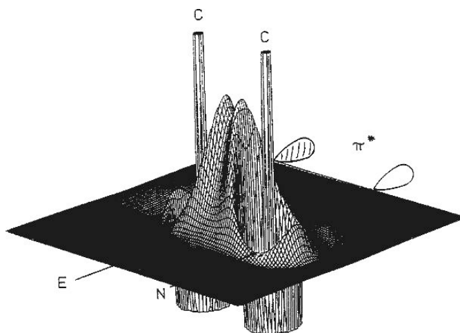
Fig. 1.40. Perspective of Laplacian -\nabla^2\rho_e(\mathbf{r}) of ethene in a plane perpendicular to the molecular plane. From E. Kraka and D. Cremer in The Concept of the Chemical Bond , Z. B. Maksic, ed., Springer-Verlag 1990, p. 533.
