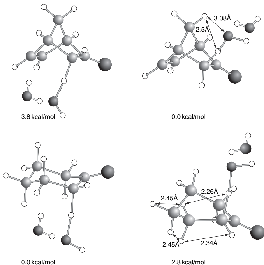
Fig. 6.3. Comparison of transition structures for deprotonation of 2-norbornanone (top) and cyclohexanone (bottom). In 2-norbornanone, exo protonation is favored by 3.8 kcal/mol. In cyclohexanone, axial deprotonation is favored by 2.8 kcal/mol. Reproduced from J. Org. Chem. , 65 , 8970 (2000), by permission of the American Chemical Society.
