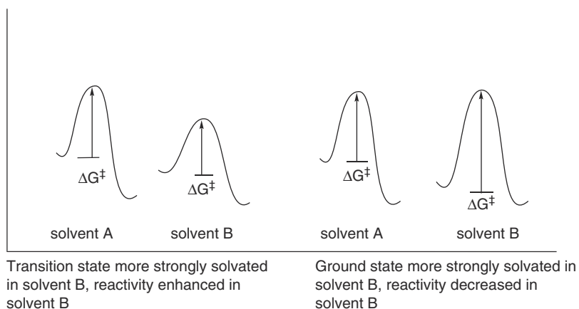
Fig. 3.34. Reaction energy profiles showing effect on E_a of (a) preferred solvation of the transition state and (b) preferred solvation of reactants.
