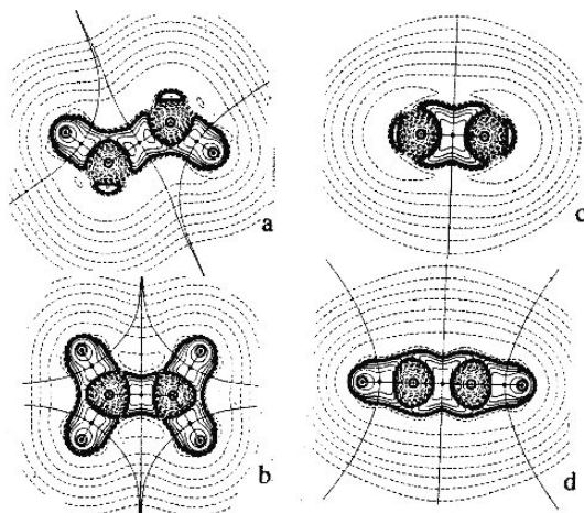
Fig. 1.39. Contour maps of L(r) for: (a) ethane in a plane bisecting anti -hydrogens; (b) ethane in the molecular plane; (c) ethane perpendicular to the molecular plane, and (d) ethyne. The solid lines depict the zero-flux surfaces of the C and H atoms. From J. Phys. Chem. 100 , 15398 (1996).
