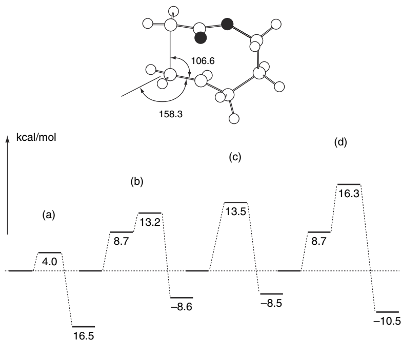
Fig. 11.10. Comparison of energies of (a) 8- endo-s-cis , (b) 8- endo-s-trans , (c) 7- exo-s-cis , and (d) 7- exo-s-trans transition structures. The s-trans conformation is 8.7 kcal/mol less stable than its s-cis . Reproduced from J. Am. Chem. Soc. , 120 , 7469 (1998), by permission of the American Chemical Society.
