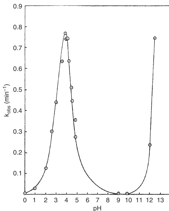
Fig. 7.P18. pH-Rate profile for hydrolysis of 3-acetoxyphthalic acid. Reproduced from J. Am. Chem. Soc. , 90 , 5833 (1968), by permission of the American Chemical Society.
