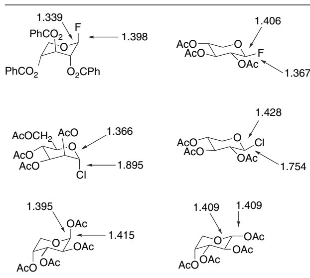
Scheme 2.17. Bond Distances in Å at Anomeric Carbons a
