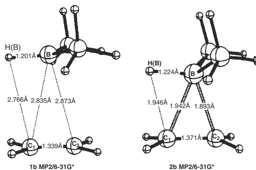
Fig. 5.6. Geometries (MP2/6-31G * ) of (a) \pi complex and (b) transition state in reaction of ethene and dimethylborane. Reproduced from J. Org. Chem. , 56 , 4074 (1991), by permission of the American Chemical Society.
