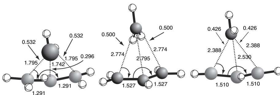
Fig. 10.34. Transition structures for suprafacial 1,3-migrations of BH 2 (left), CH 3 (center), and NH 2 (right) at the QCISD/6-311+G** level. Bond distances and NPA bond orders are shown. Adapted from J. Phys. Chem. A , 106 , 5709 (2002), by permission of the American Chemical Society.
