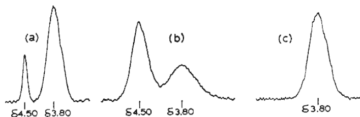
Fig. 2.15. 60-MHz ^1\text{H-NMR} spectrum for the C(1)H in chlorocyclohexane: (a) axial-equatorial equilibrium at -115^\circ\text{C} ; (b) axial-enriched mixture at -150^\circ\text{C} ; (c) pure equatorial conformer at -150^\circ\text{C} . Reproduced from J. Am. Chem. Soc. , 91 , 3223 (1969), by permission of the American Chemical Society.
