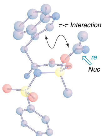
Fig. 7.15. Facial selectivity of 3-indolylmethylboronate ester catalyst. Reproduced from Tetrahedron Asymmetry , 9 , 357 (1998), by permission of Elsevier. (See also color insert.)
