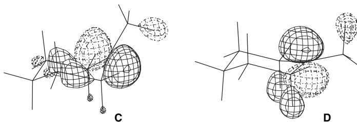
Fig. 4.9. Distribution of LUMO orbitals of isomeric 1-methylcyclohexyl cations showing dominant C–C (C) and C–H (D) hyperconjugation. Reproduced from J. Am. Chem. Soc. , 118 , 3761 (1996), by permission of the American Chemical Society.
