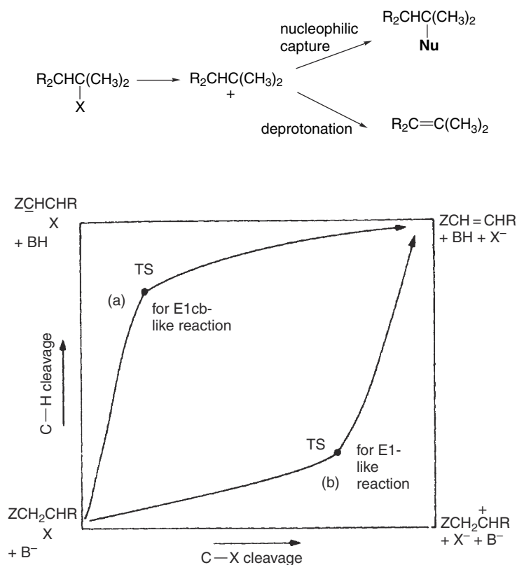
Fig. 5.13. Representation of changes in transition structure character in the E2 elimination reaction as a result of substituent effects: (a) substituent Z stabilizes carbanion character of E1cb-like TS; (b) substituent R stabilizes carbocation character of E1-like TS.
