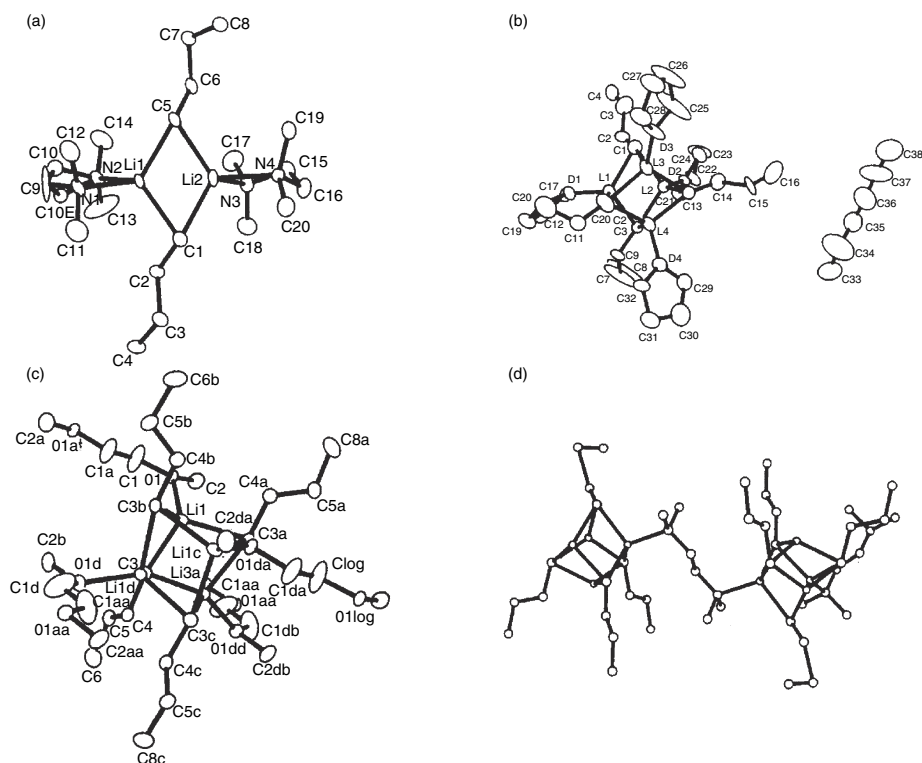
Fig. 6.2. Crystal structures of n -butyllithium: (a) [(n\text{-BuLi-TMEDA})_2]_2 ; (b) [(n\text{-BuLi-THF})_4]\text{hexane} ; (c) [(n\text{-BuLi-DME})_4] ; (d) [(n\text{-BuLi})_4]\text{TMEDA} . Reproduced from J. Am. Chem. Soc. , 115 , 1568, 1573 (1993), by permission of the American Chemical Society.
