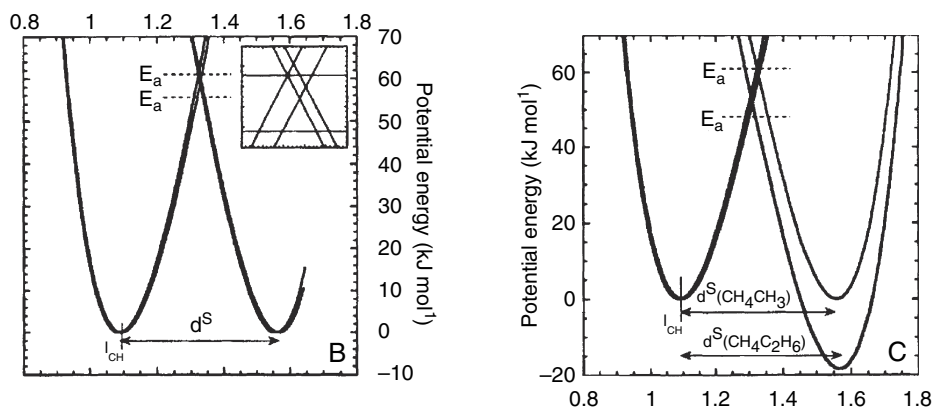
Fig. 11.18. Comparison of Morse curves from: (a) \text{CH}_3\cdot + \text{CH}_4 and \text{C}_2\text{H}_5\cdot + \text{C}_2\text{H}_6 thermoneutral; and (b) \text{CH}_3\cdot + \text{C}_2\text{H}_6 exothermic hydrogen atom transfer reactions. Reproduced from J. Mol. Struct. , 563 , 1 (2001), by permission of Elsevier.
