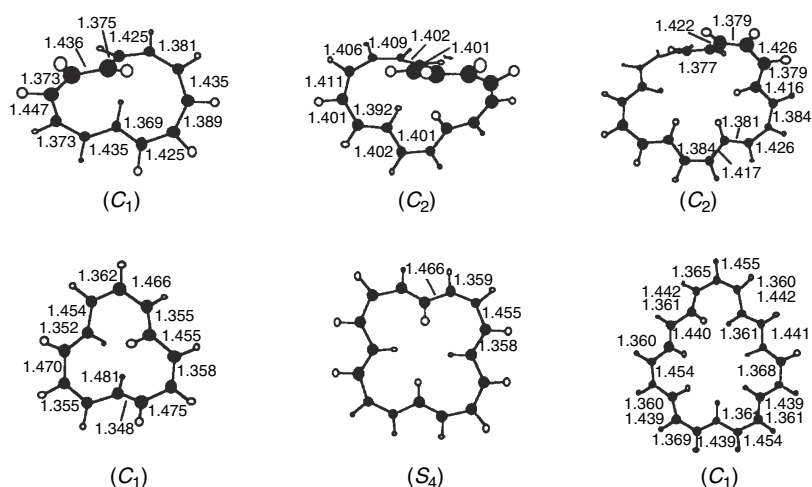
Fig. 8.7. Most stable (top) and most aromatic (bottom) Möbius structures for [12], [16], and [20]annulene. Reproduced from Org. Lett. , 4 , 3431 (2002), by permission of the American Chemical Society.
