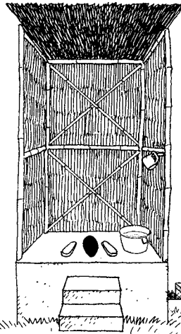
Above ground chamber allows wastewater to flow down to pits. With regular care, this toilet will last many, many years.
