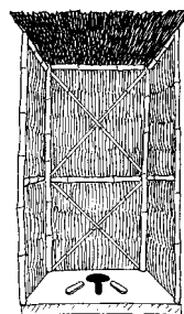
Closed pit toilet Best in places with deep groundwater and no risk of flooding (see page 120).
