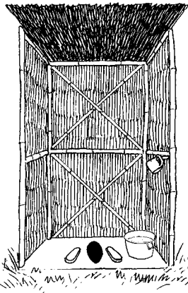
One lined pit underground, 2 meters deep. A family of 5 will fill this pit in about 5 years time.
