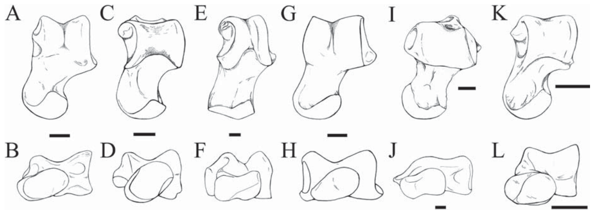
FIGURE 5.13. Comparison of apheliscid astragali to other taxa in dorsal and distal views. A, B, Apheliscus (USNM 521791, reversed): A, dorsal; B, distal. C, D, Haplomylus : C, dorsal (composite of USNM 493902 and 513632); D, distal (USNM 513632). E, F, Rhynchocyon (USNM 537657): E, dorsal; F, distal. G, H, Prodiacodon (USNM 513636, reversed): G, dorsal; H, distal. I, J, Hyopsodus : I, dorsal (USNM 25331, reversed; details from USNM 493782 and YPM unnumbered); J, distal (YPM unnumbered). K, L, Macrocranion : K, dorsal (UCMP uncat., reversed); L, distal (USNM 493780). All scale bars equal 1 mm.
