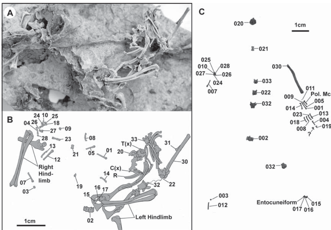
FIGURE 11.7. Documentation of association of micromomyid skeleton, cf. Tinimomys graybulliensis from UM locality SC-026 (currently uncatalogued). A, Photograph of a partly prepared limestone yielding a Wasatchian-aged micromomyid skeleton. B, Map of distribution of the bones in the limestone. Although it lacks craniodental remains, this specimen does preserve many of the same elements as that in Figure 11.6, so we can confidently identify it to the familial level, given its age, we tentatively refer to Tinimomys graybulliensis . The specimen includes complete tibiae, fibulae, innominates, and a complete radius. C, Some of the fully removed and prepared bones from this specimen in rough anatomical position. Note that most of the right wrist, the left hand, many vertebrae, and the left distal tarsal row are preserved. Scale = 1 cm.
