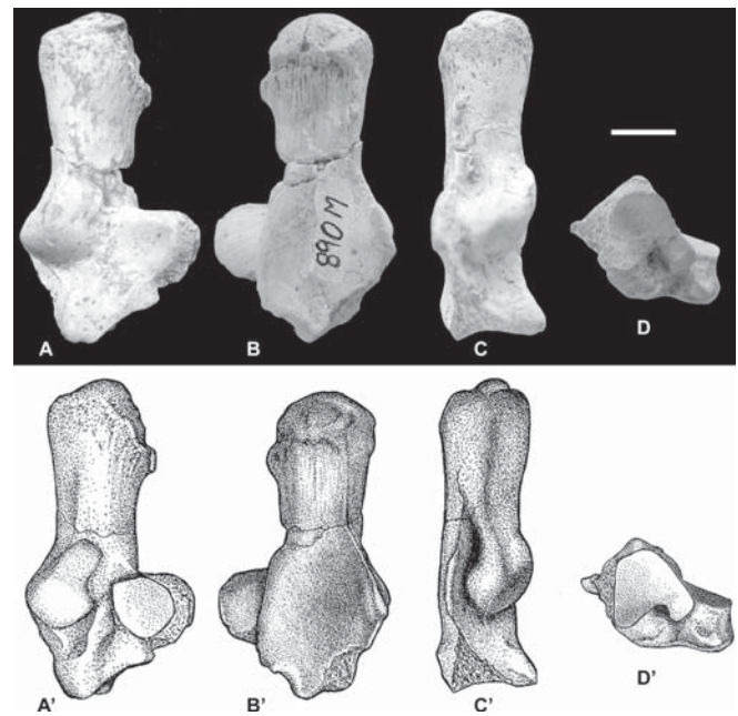
Figure 6.22. Right calcaneum of “Condylarthra” indet. A , dorsomedial; B , plantar; C , lateral, and D , distal views of DGM 890M. Outline drawings of calcaneum in A' , B' , C' , and D' in the same views. Scale bar: 1 cm.
