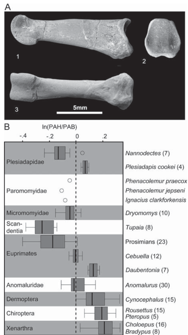
FIGURE 11.12. A, Plesiadapis cookei (UM 87990) intermediate phalanx. 1, lateral; 2, proximal; and 3, volar view. P. cookei has a proximal articular surface that is dorsoventrally taller than it is mediolaterally wide. The shaft is straight, or slightly dorsally convex (depending on how the central axis is defined) with no dorsal re-curvature at the distal end. Contrary to what this specimen shows, these features (and others) were said to be uniquely shared by paromomyids and dermopterans among “plesiadapiforms,” primates, treeshrews and most other mammals (Beard, 1993b). Scale = 5 mm. B, Plot of natural log ratio of dorsoventral height of the proximal articular surface (PAH) to mediolateral breadth of surface (PAB) of intermediate phalanges. Alternating gray and white bars demarcate higher-level taxa. Contrary to previous claims paromomyids, dermopterans and bats are not uniquely characterized by a high value of this ratio (plotting right of the dashed line). Plesiadapis (as shown qualitatively in A), Daubentonia , and sloths plot in this realm, but paromomyids do not. Intermediate phalanges of Acidomomys hebeticus were not included here because none were preserved with their proximal epiphyses solidly attached. Sample sizes are given after taxon names in parentheses. See Appendix II, Table 1 for specimens included.
