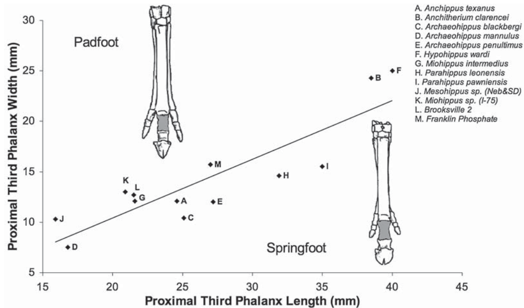
FIGURE 8.2. Plot of PPIIIL/MW index for ASL equids included in this study. The trend line differentiates the broad phalanx of the padfoot equid from the narrow waisted phalanx of the springfoot equid. The Mesohippus (padfoot) and Merychippus (springfoot) manual skeletons are redrawn from Simpson (1951).
