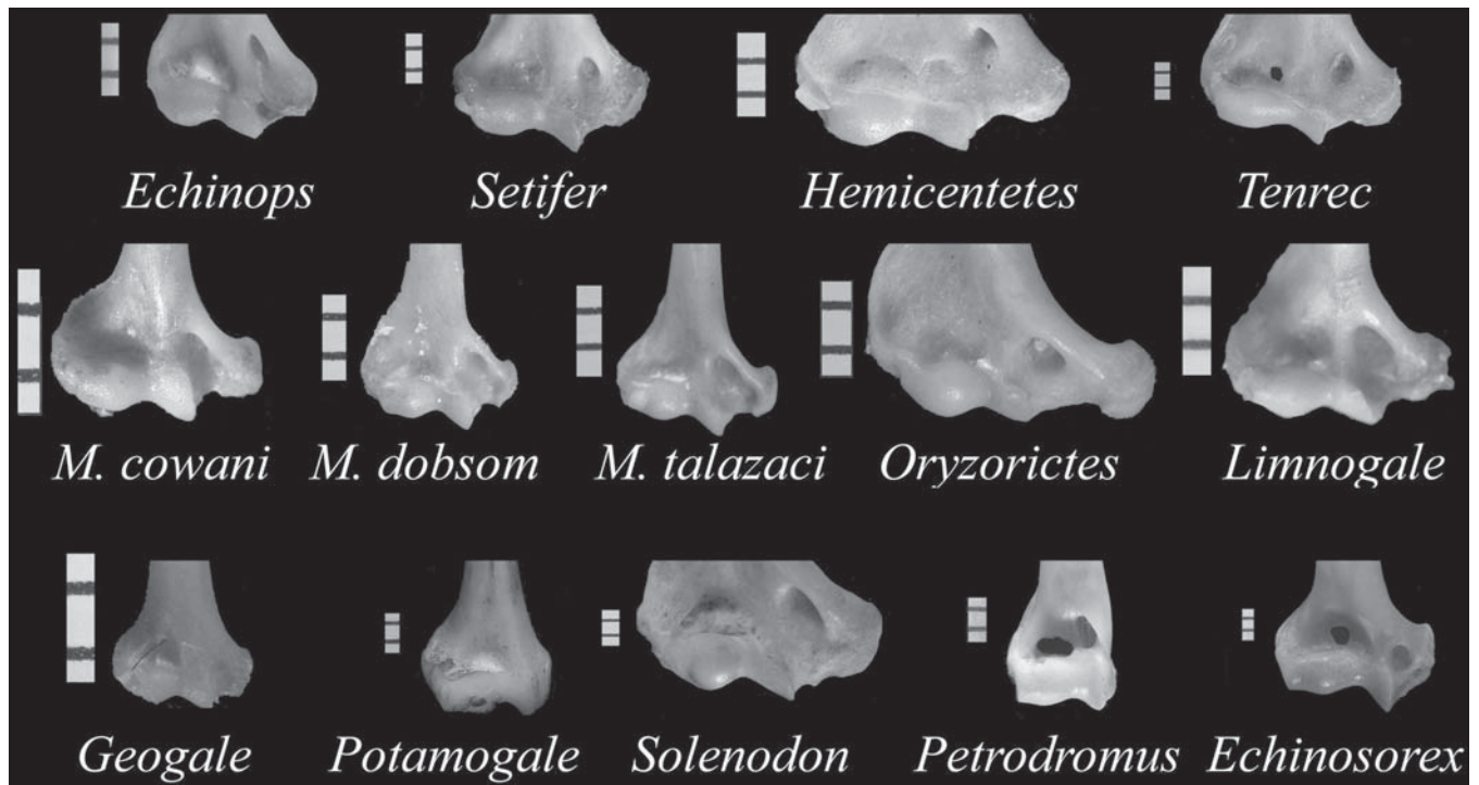
FIGURE 4.11. Anterior view of right distal humerus in tenrecines (top), oryzoricetines (middle), two other tenrecoids (bottom left), and three outgroup taxa (bottom right). Note differences in the shape of the trochlea and capitulum, especially the convergence in form between Potamogale and Petrodromus . Subdivisions on scale are 1.0mm.
