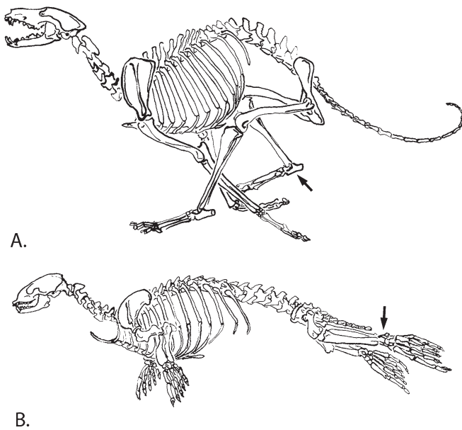
FIGURE 9.1. Skeleton of Canis familiaris , the domestic dog (A) and Phoca vitulina , the Harbour seal (B). (After Gregory, 1951.) Arrows point to the calcaneum and astragalus.
