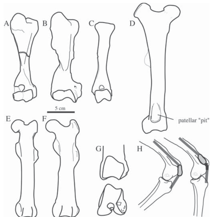
FIGURE 7.7. Ungulate limb bones. Cranial views of humeri (A, Eurygenium pacegnum Bol-V-00364; B, Trachytherus alloxus , UF 91933; C, Coniopternium sp., UF 149207) and femora (D, Coniopternium sp. MNHN-Bol-V-004502; E, Eurygenium pacegnum Bol-V-00364; F, Trachytherus alloxus , UF 90960; and G, Proadinothierium , cf. P. saltoni sp. nov. (anterior view also provided) MNHN-Paris [uncataloged]), and H, a functional reconstruction of the knee lock of Coniopternium sp. show as flexed (left) and hyper-extended and locked (right). (H modified from Shockey, 1999.)
