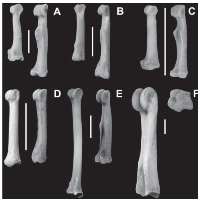
FIGURE 11.13. Intermediate and proximal phalanges of various taxa. A, Ignacius clarkforkensis ; B, Cebuella pygmaea ; C, Dryomomys szalayi ; D, Pteropus pumillio ; E, Cynocephalus volans ; F, Choloepus hoffmani . Ventrolateral view of intermediate phalanx (on the left) and proximal phalanx (on the right). Manual elements are represented except in the case of Pteropus , for which toe bones are shown. Functionally, its toes are more comparable to the fingers of the other taxa shown, than are its own fingers, which are modified as wings. Phalanges are normalized to length of the proximal phalanx to show variation in intermediate phalanx length, except for F, which is normalized to the length of intermediate phalanx in E. Note that suspensory taxa D–F differ from fossils (A and C) and vertical climber and climber (B) in having intermediate phalanges that are relatively longer, with more ventrally facing distal articular surfaces and less distinct flexor sheath tubercles. The proximal phalanges of the suspensory taxa have more deeply trochleated distal articular surfaces. See Appendix II, Table 1 for specimen numbers. Scale bars = 3 mm.
