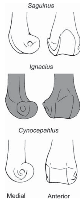
FIGURE 11.31. Distal femora showing patellar morphology. From top to bottom is Saguinus mystax (UMMZ 160148), Ignacius clarkforkensis (UM 82606), and Cynocephalus volans (USNM 56530) in medial and anterior view. Note that despite being an agile arborealist the distal femur in Saguinus is nearly identical to that in Ignacius . Both of these taxa differ only slightly from the condition in C. volans with respect to patellar groove morphology. However, other features discussed and figured in this chapter differentiate the fossil and Saguinus from C. volans , showing the former two taxa to be capable of pronograde postures and to be more agile than the latter. Images are standardized to distal femur mediolateral breadth.
