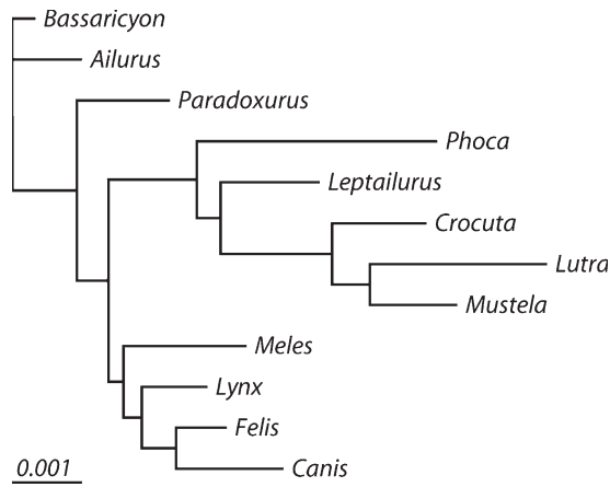
FIGURE 9.13. A maximum likelihood tree constructed from calcaneum and astragalus shape. The groupings are influenced by low-level phylogenetic relationship and locomotor type, but do not clearly indicate either.
