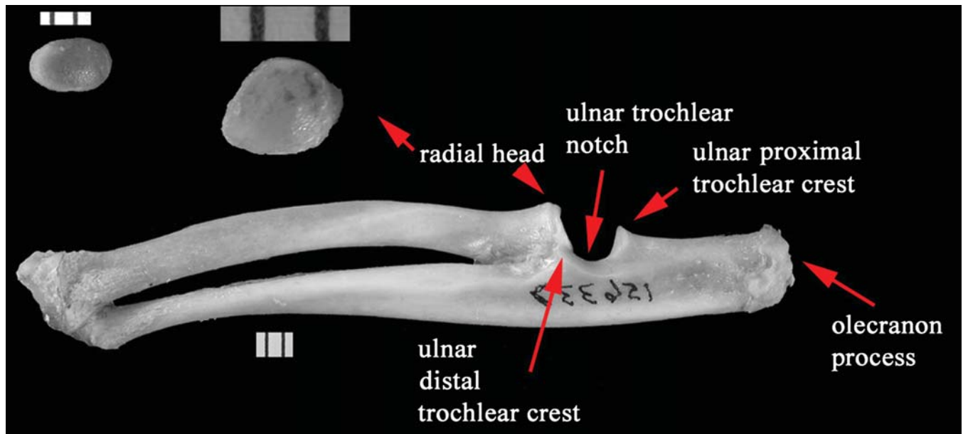
FIGURE 4.3. Right radii and ulna of Setifer , Limnogale , and Tenrec . Proximal view of Setifer radius (top left), illustrating mediolaterally elliptical radial head, proximal view of Limnogale radius (middle top), demonstrating a rounded head, and medial view of Tenrec antebrachium (bottom). Subdivisions on scale are 1.0 mm.
