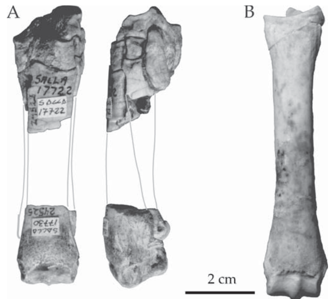
FIGURE 7.5. Proterotheriid pes. A, partial right pes of the proterotheriid of Salla, composite of the distal tarsals and proximal Mt II-IV (PU 24528) and distal metapodials (PU 24525). (Reconstructed as if from a single individual.) B, left Mt III from Cabeza Blanca (AMNH 14153).
