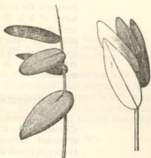
Strepitium floribundum : culms with leaves during the day, and when asleep at night. Figures reduced.
