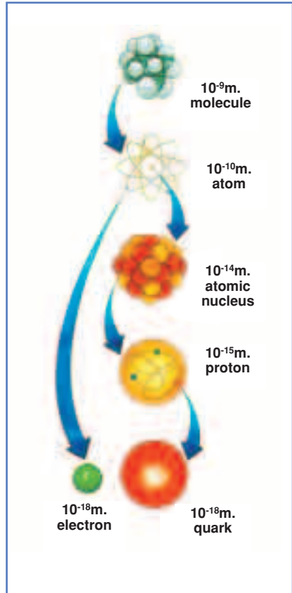
From the structure of the atom to the structure of the quark, it is possible to analyse the smallest particles forming the atom using modern accelerators. The diagram above illustrates this relationship in a progressive fashion.
