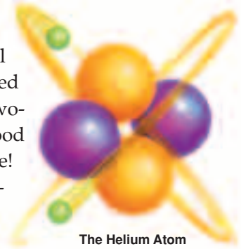
The Helium Atom
