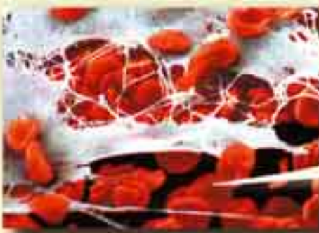
Blood cells
