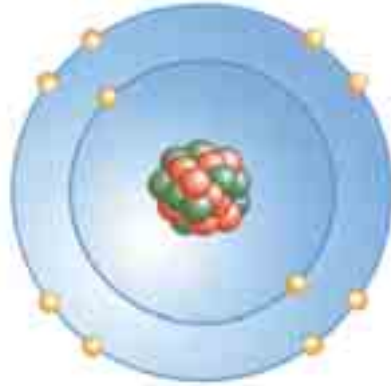
Atoms achieve a stable structure only when the number of electrons in their outer shell reaches 8. The neon is a very stable atom with eight electrons in its outermost orbit.
