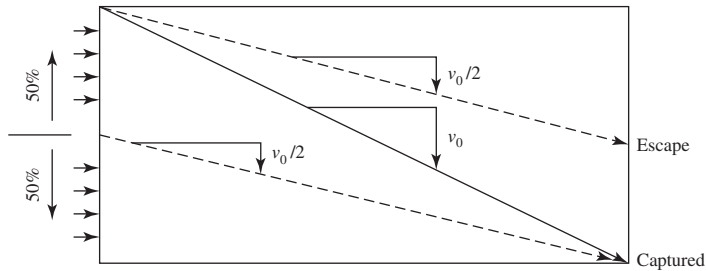
FIGURE 10-7 Partial particle removal in an ideal sedimentation tank. (Source: Davis and Cornwell, 2008.)
