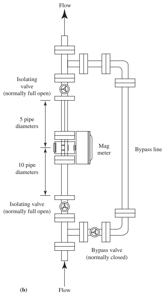
FIGURE 20-4 (a) Schematic of magnetic flowmeter and (b) correct installation locations. (Schematic courtesy of Fisher & Porter.)
