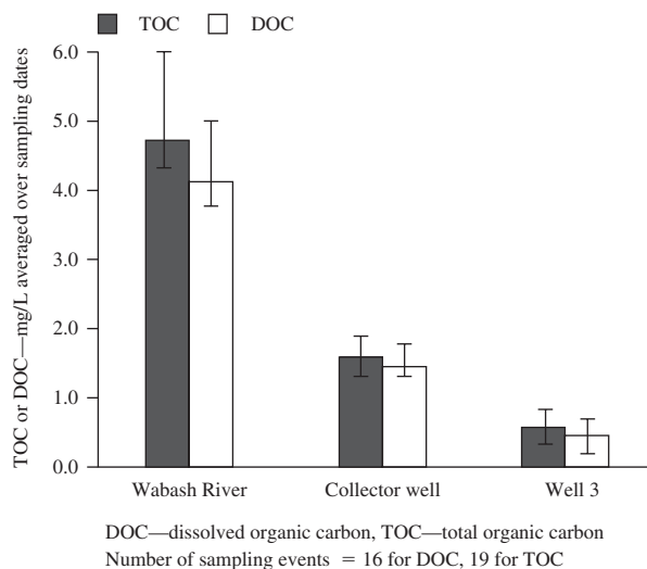
FIGURE 16-3 Average TOC and DOC concentrations at Terre Haute, Indiana. (Source: Weis et al., 2003.)
