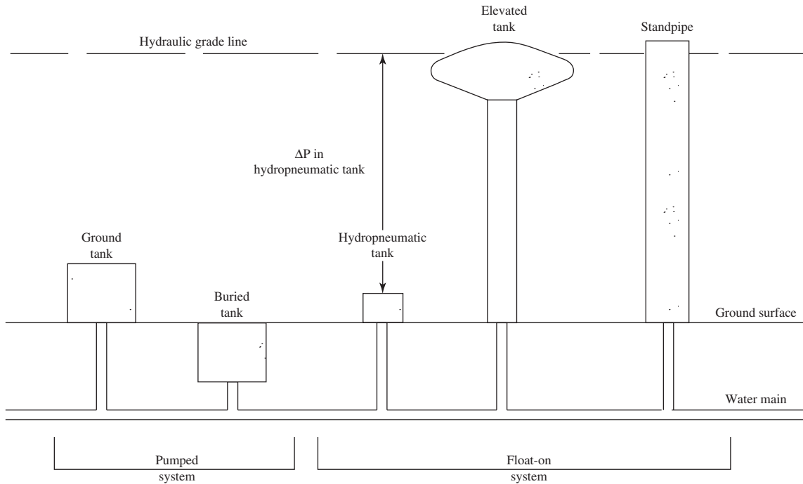
FIGURE 17-10 Tank terminology.
