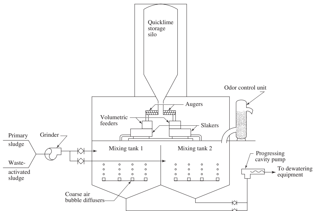
FIGURE 27-10 Conceptual design for a lime stabilization facility. (Source: U.S. EPA, 1979.)
