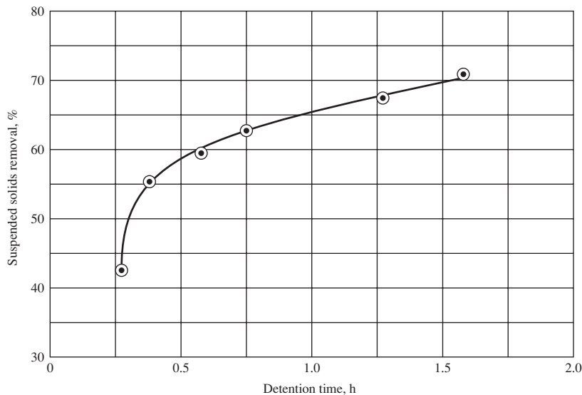
FIGURE 10-9 Suspended solids removal versus detention time. (Source: Davis and Cornwell, 2008.)
