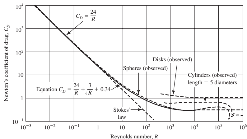
FIGURE 10-2 Newton's coefficient of drag as a function of Reynolds number. (Source: Camp, 1946.)
