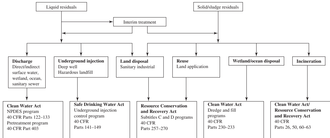
FIGURE 15-13 Arsenic residuals disposal—federal regulations. (Adapted from U.S. EPA, 2000.)
