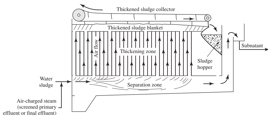
FIGURE 15-3 Dissolved air flotation (DAF) thickener.
