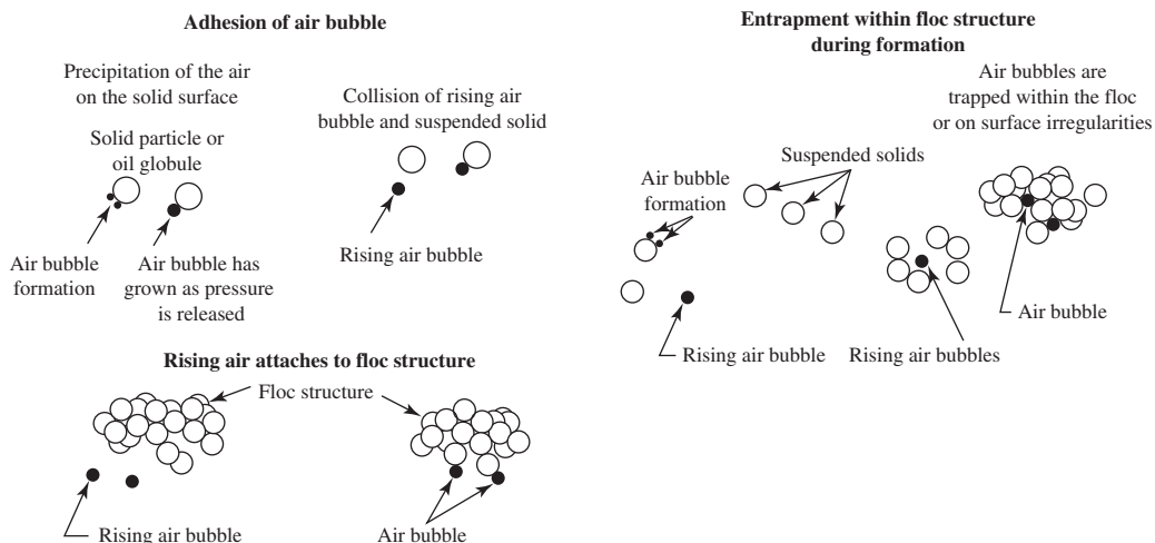
FIGURE 27-7 Solid-bubble contacting mechanisms.
