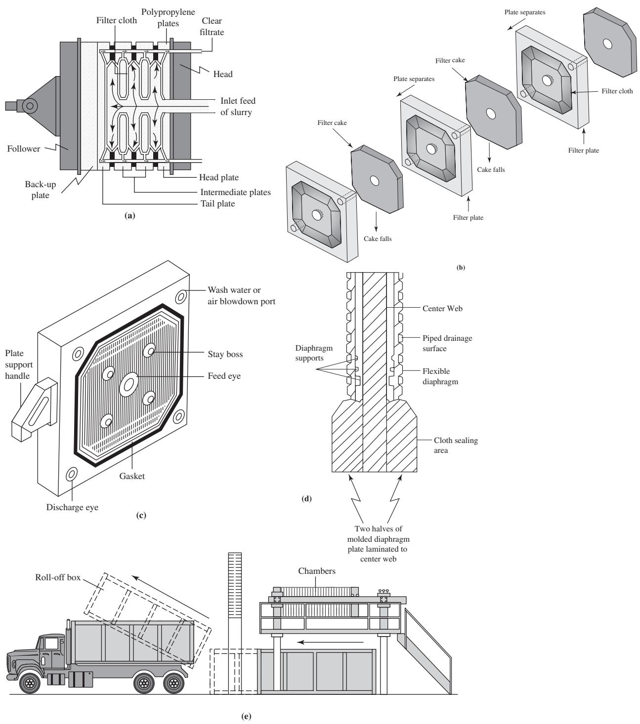
FIGURE 15-10 Plate and frame filter press. (a) Filling the press, (b) cake breaking, (c) plate details for recessed plate, (d) diaphragm plate details, (e) plate and frame solids off-loading system.
