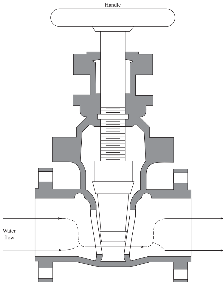
FIGURE 17-3 Gate valve.
