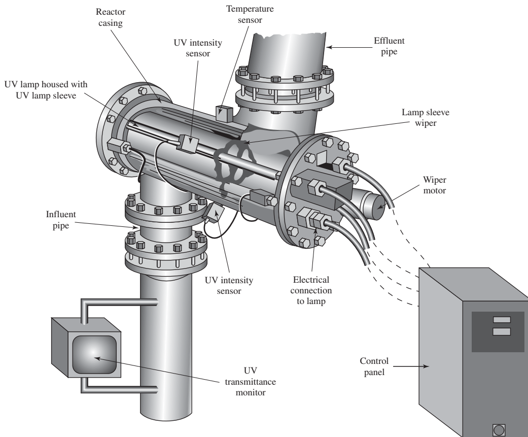
FIGURE 13-14 UV disinfection system schematic. (Source: Aquionics.)
