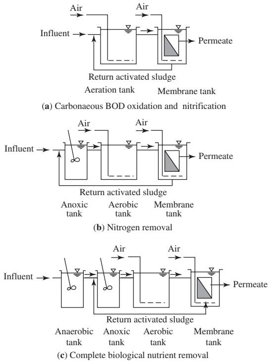
FIGURE 23-7 Process arrangements for membrane bioreactors (MBR).
