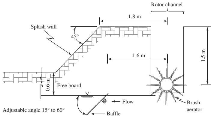
FIGURE 23-20 Downstream baffle for liquid depth greater than 2 m.
