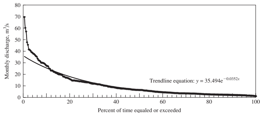
FIGURE 2-3 Complete series analysis for Troublesome Creek at Nosleep.
