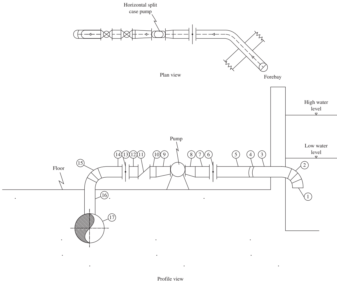
FIGURE 17-15 High-service pump piping system. See Table 17-10 for key to numbered components.
