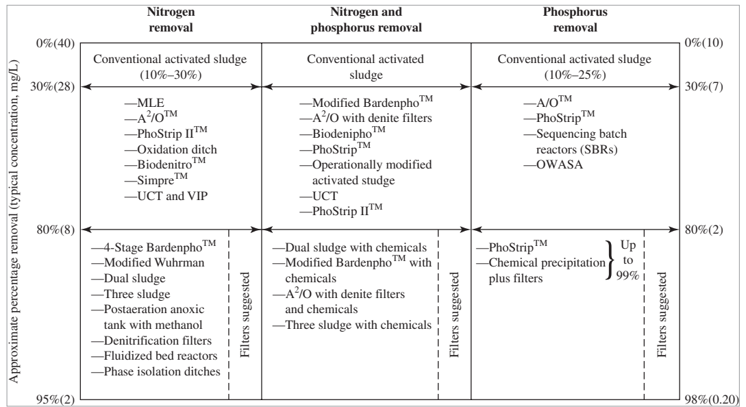
FIGURE 28-1 Process selection matrix for nutrient removal (MLE = modified Ludzack-Ettinger and UTC = University of Cape Town). (Source: WEF, 1998.)
