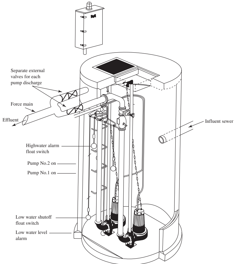
FIGURE 19-18 Factory-assembled lift station with submersible pumps. The external valves are placed in a chamber that allows access without entering a confined space. (Adapted from Steel and McGhee, 1979.)
