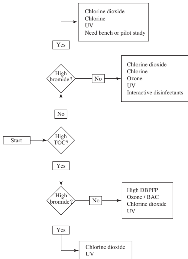
FIGURE 13-8 Flow diagram to narrow selection of a new primary disinfectant for systems that filter. (Source: Adapted from U.S. EPA, 1999.)
