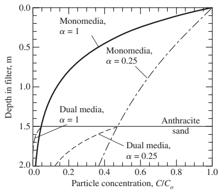
FIGURE 11-6 Effect of attachment efficiency on effluent from monomedia and dual-media filters. (Source: MWH, 2005.)
