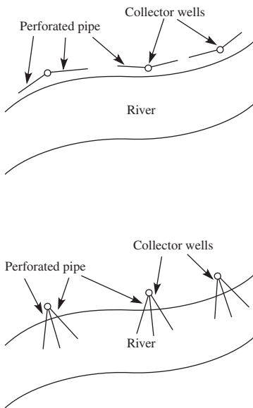
FIGURE 3-5 Two arrangements of infiltration galleries with wells.
