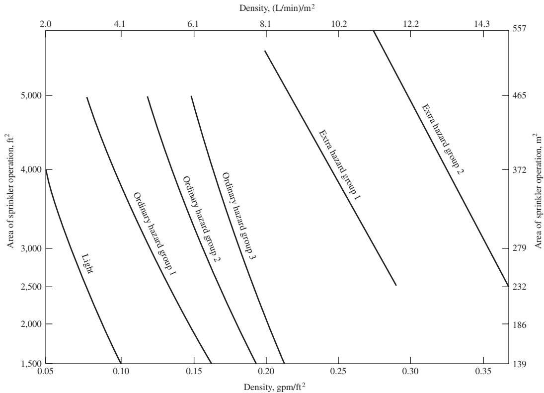
FIGURE 17-1 Sprinkler system design curves. Reprinted with permission from NFPA, 13-1987. (Source: NFPA, 1987.)
