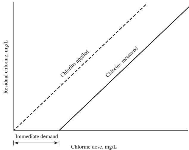
FIGURE 13-3 Chlorine demand exhibited by a very fast reaction such as that with sulfur dioxide.
