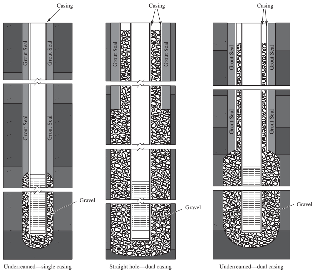
FIGURE 4-4 Some alternative schemes for packing gravel in a gravel-packed well.
