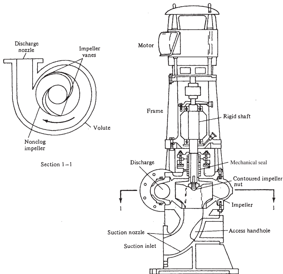
FIGURE 19-15 Typical vertical shaft radial-flow wastewater pump. (Source: Metcalf & Eddy, 1981.)
