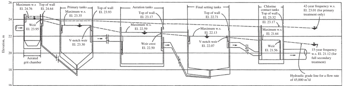
FIGURE P-28-4 Hydraulic profiles for clean water plant. (Note: WS = water surface.)
