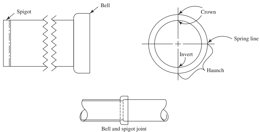
FIGURE 19-3 Nomenclature of a sewer pipe.
