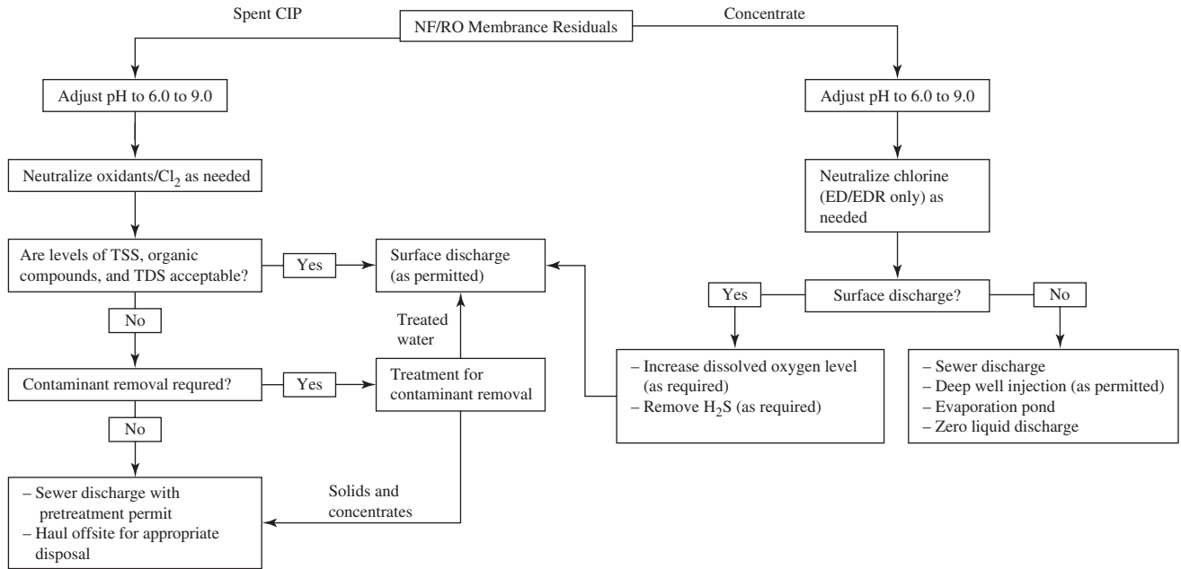
FIGURE 15-12 Decision tree for NF/RO membrane residuals management. (CIP—clean in place chemicals, TSS—total suspended solids, TDS—total dissolved solids.)
