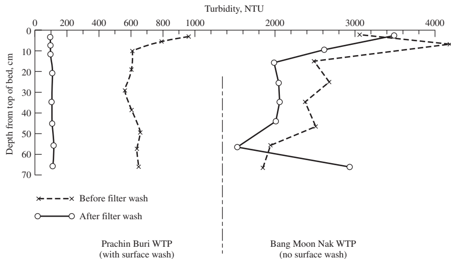
FIGURE 11-12 Sludge profile in filter beds. Amount of sludge is shown as turbidity (NTU). (Source: Kawamura, 2000.)
