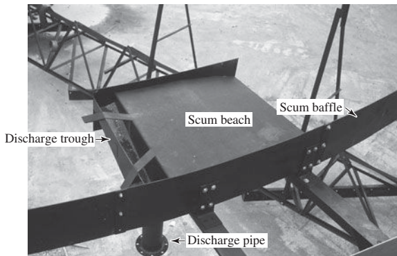
FIGURE 21-12 Scum “beach” for circular clarifier.
