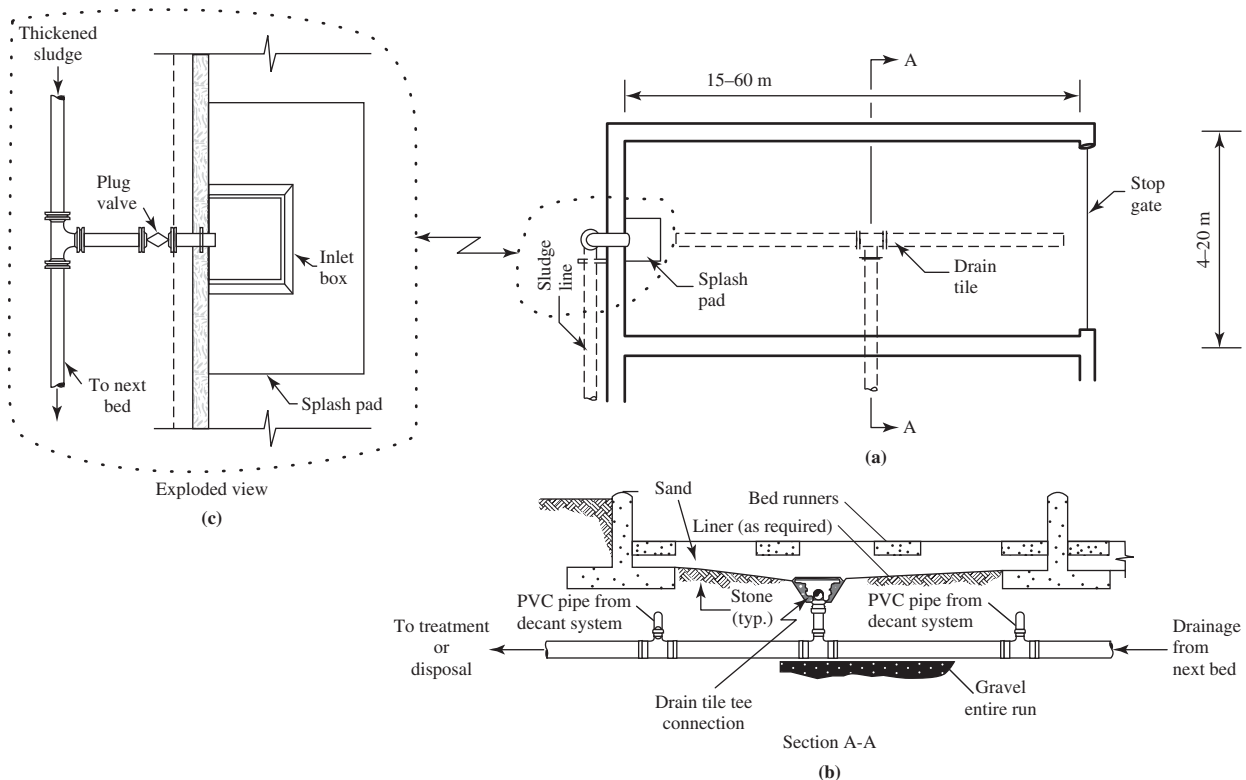
FIGURE 15-7 Sand drying bed. (a) Plan view, (b) cross section, (c) exploded view of inlet.
