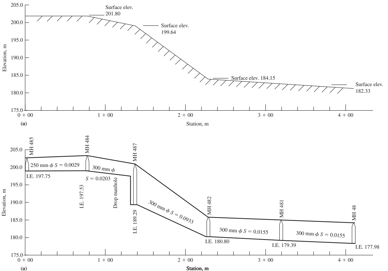
FIGURE 19-13 Profiles for Example 19.2. (a) Surface profile. (b) Sewer profile. Note: drop through manhole has been ignored.
