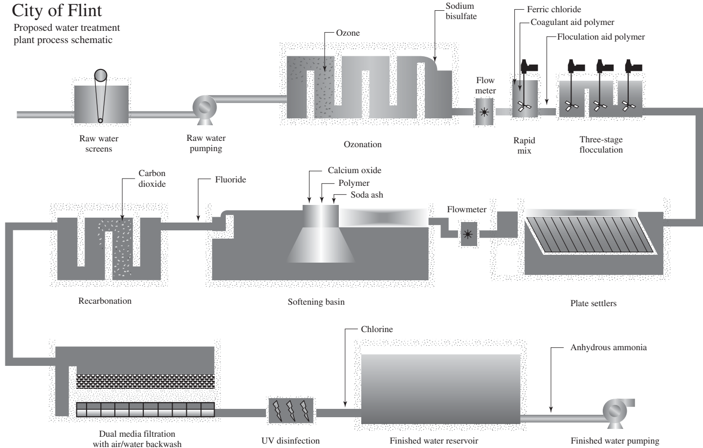
FIGURE P-16-10 Flint's WTP.
