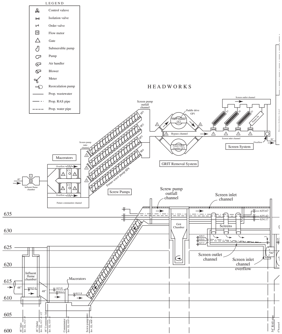
FIGURE 28-5 Hydraulic profile of PARCC Side Clean Water Plant.
