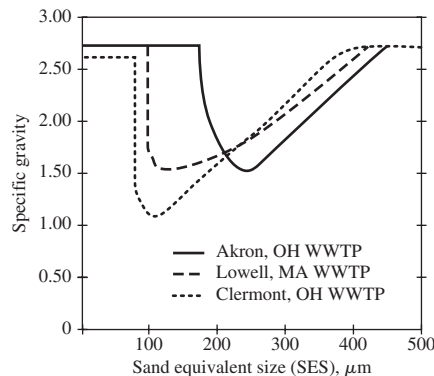
FIGURE 20-10 Variation in specific gravity of grit. (Source: Courtesy of Eutek, 2008.)
