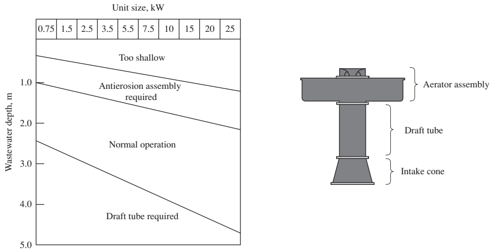
FIGURE 20-18 Floating aerator depth requirements and an illustration of a draft tub.
