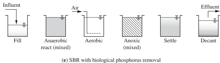
FIGURE 23-5 Processes for biological phosphorus removal. (Adapted from Metcalf & Eddy, 2003.)
