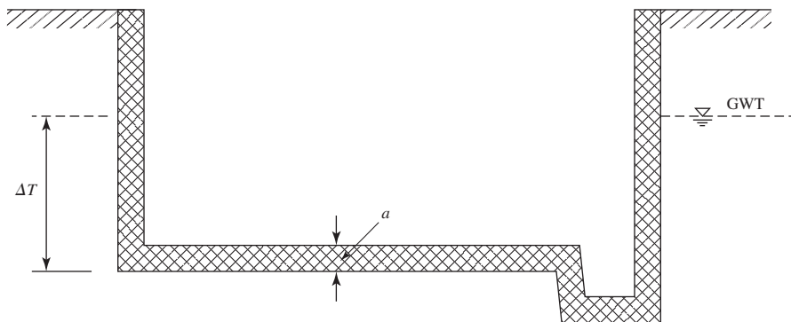
FIGURE 21-5 Empty tank with high ground water table (GWT). concrete thickness = a .
