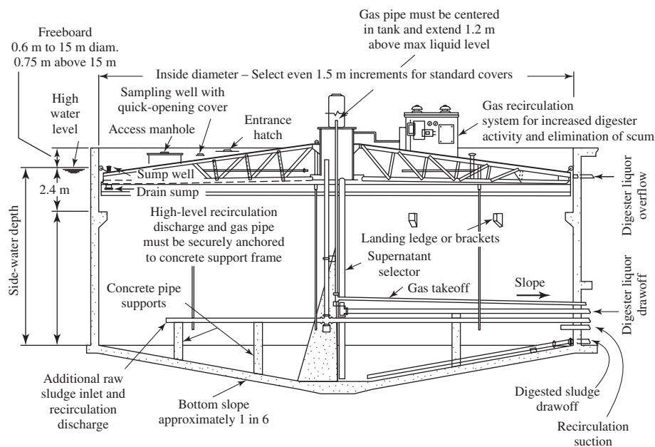
FIGURE 27-17 Cross section detail of an anaerobic digester with a floating cover. (Courtesy of Envirex.)
