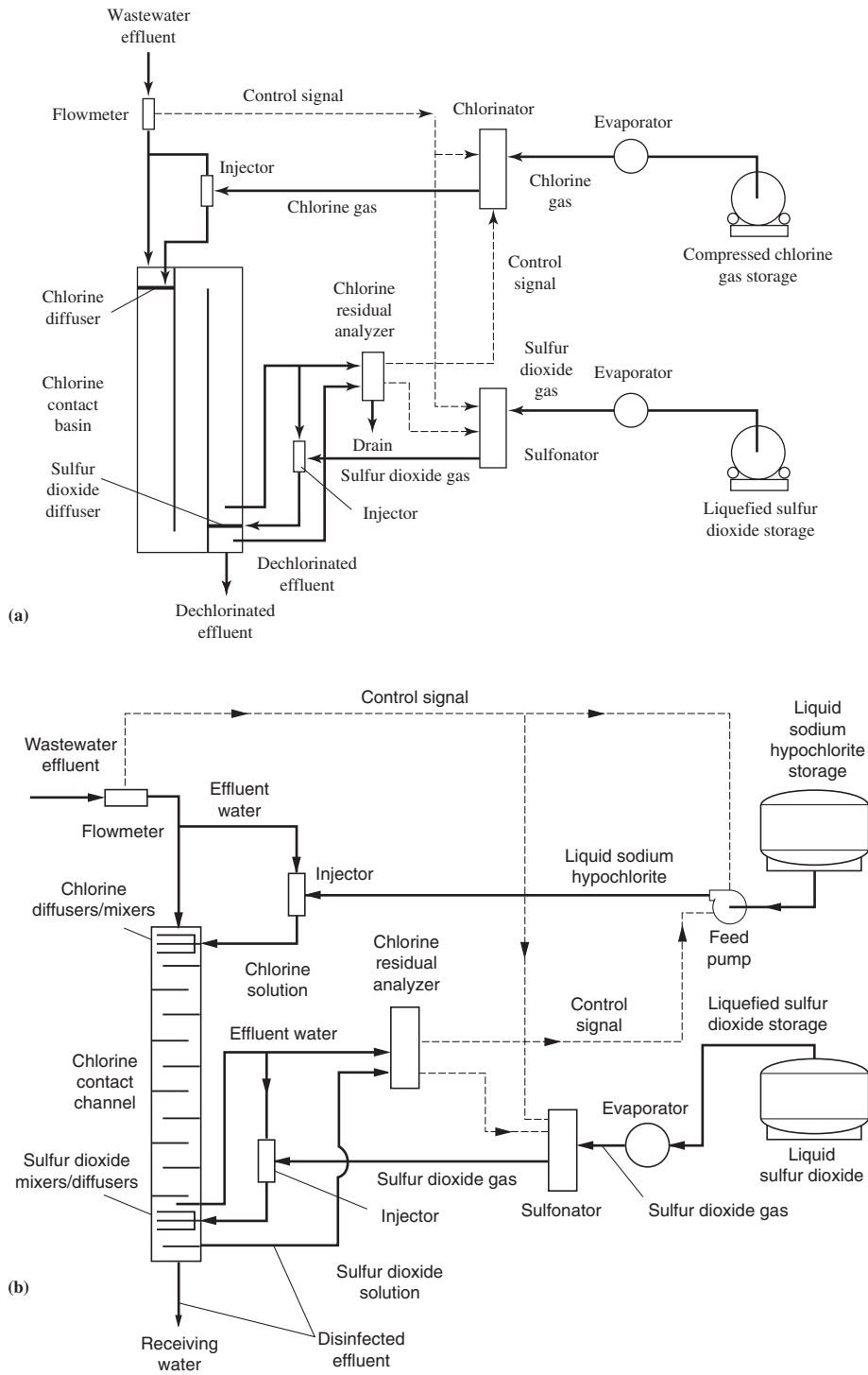
FIGURE 25-7 Schematic flow diagrams for chlorination/dechlorination. Schematic (a) uses a chlorine injector. Schematic (b) is for sodium hypochlorite injection. Both schematic use SO 2 for dechlorination. (Source: Metcalf & Eddy, 2003.)
