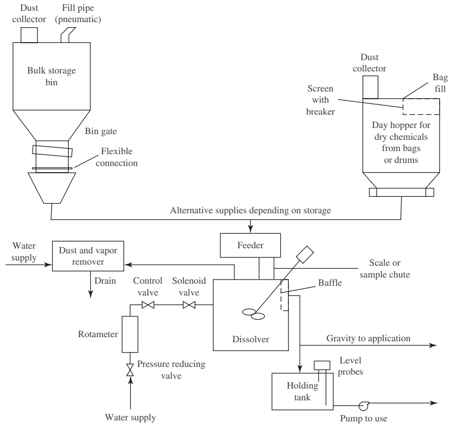
FIGURE 5-3 Dry chemical feed system. (Source: Metcalf & Eddy, 2003.)
