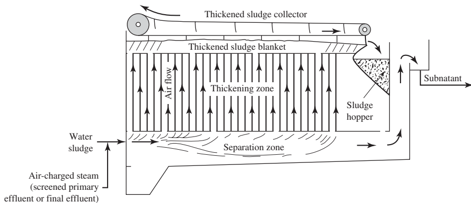
FIGURE 27-8 Air flotation thickener. (Source: Davis and Cornwell, 2008.)
