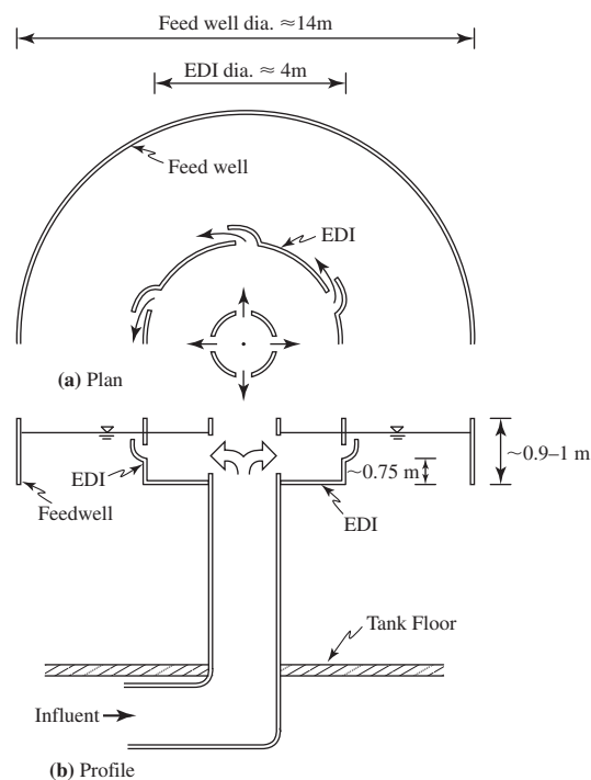
FIGURE 21-8 Center Feed with energy dissipating inlet (EDI). Approximate dimensions are for a 55 m diameter primary tank with a 4.6 m side water depth.
