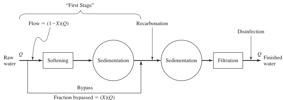
FIGURE 7-9 Split-flow treatment scheme. (Source: Davis and Cornwell, 2008.)
