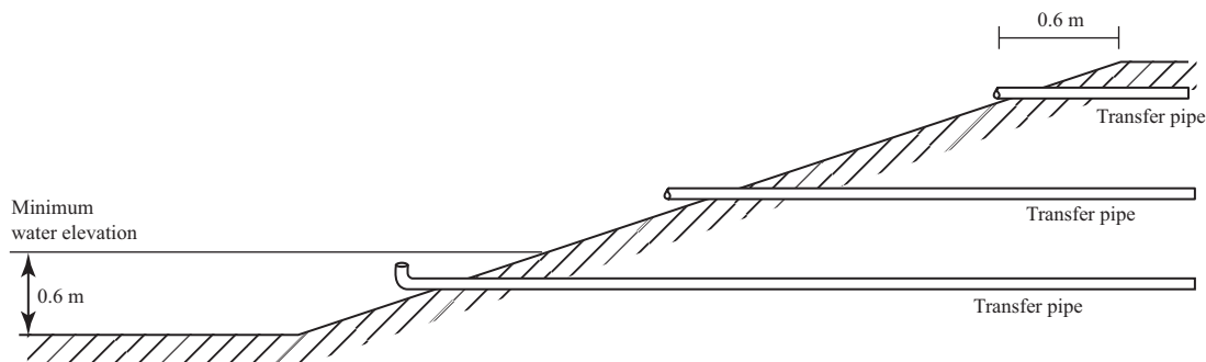
FIGURE 23-16 Dimensions for transfer pipes. Note lowest pipe has upturned intake.
