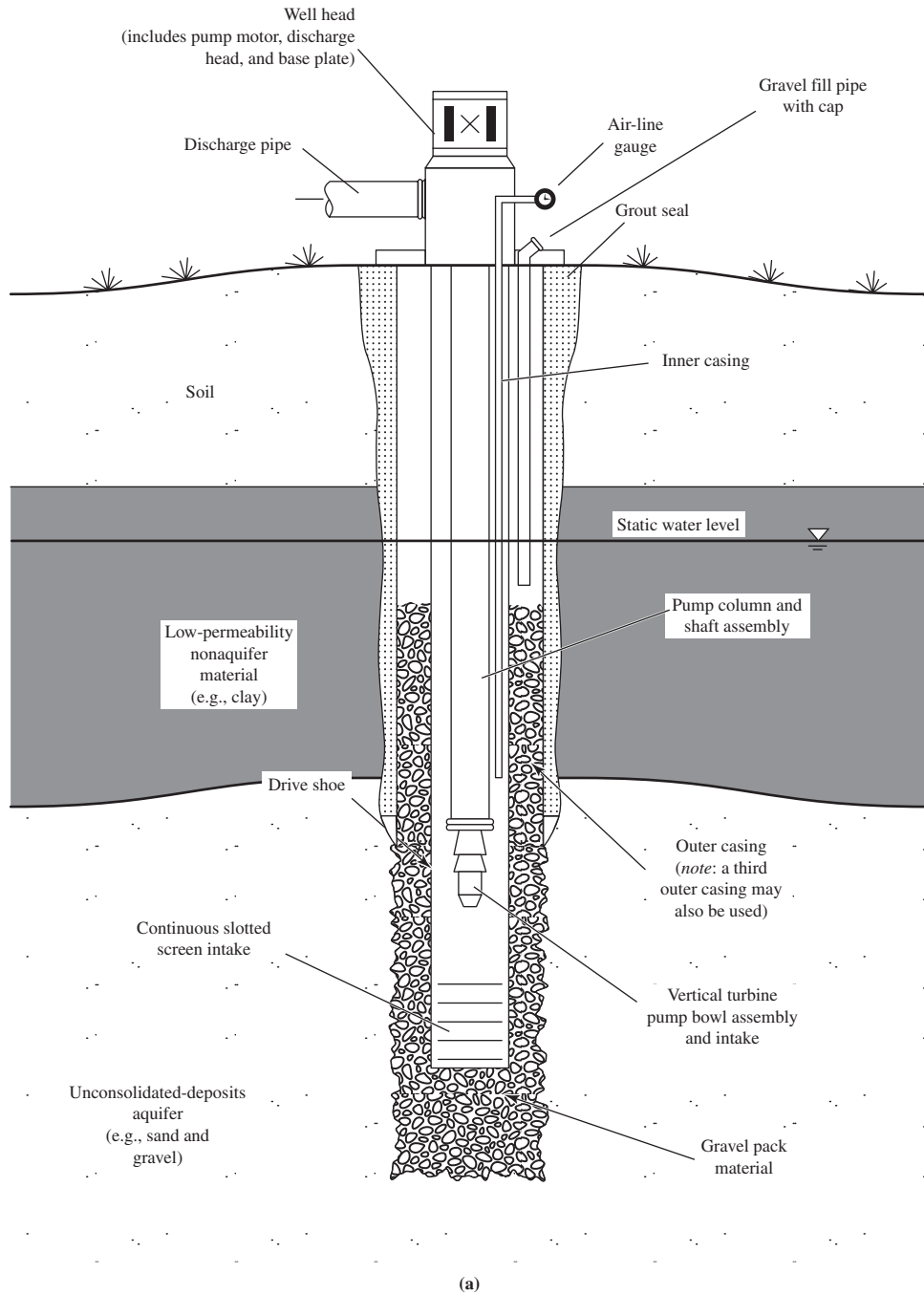
FIGURE 4-1 (a) Typical construction of a screened, gravel-packed well in an unconsolidated-deposits aquifer.
