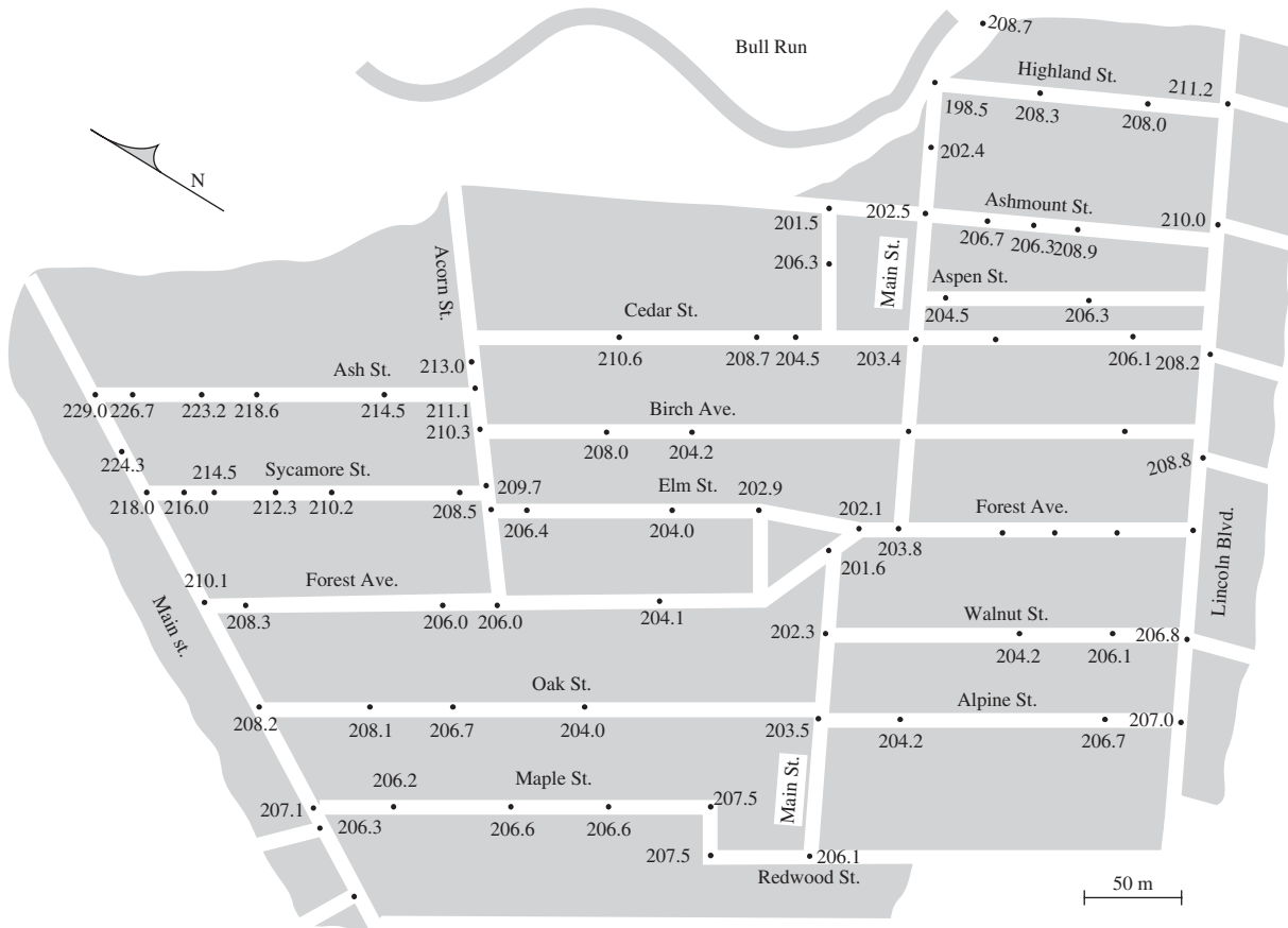
FIGURE P-19-9 Map for sewer layout. Elevations are in meters above mean sea level at points noted by dots. These are not manhole locations. (Adapted from Metcalf & Eddy, 1981.)
