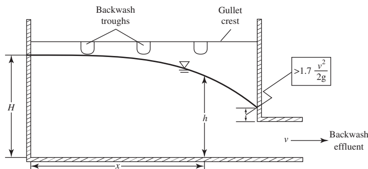
FIGURE 11-14 Illustration of terms used for gullet design (Equation 11-20).
