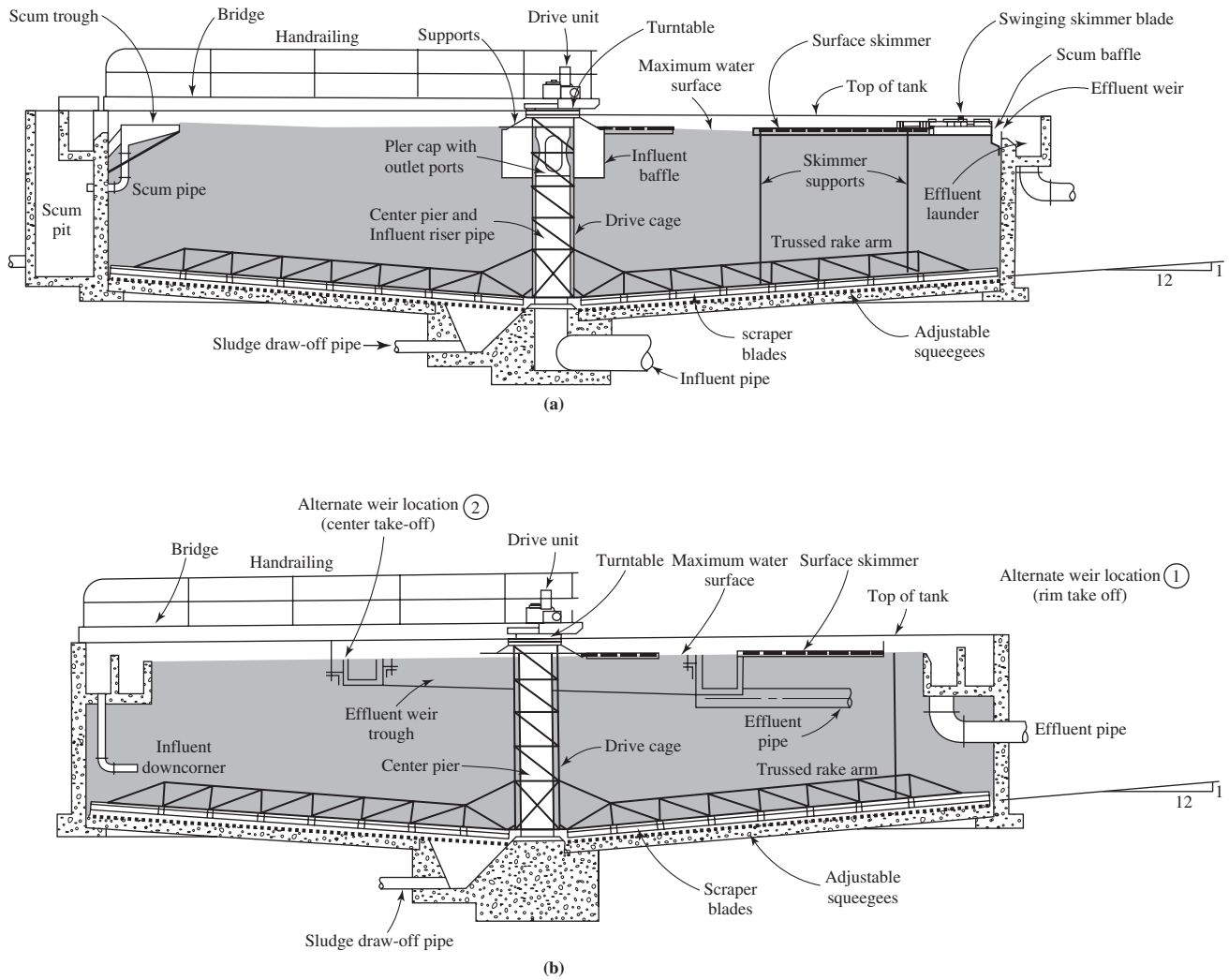
FIGURE 21-1 Circular primary setting tanks: (a) center-feed, (b) peripheral feed. (Source: Metcalf & Eddy, 1991.)
