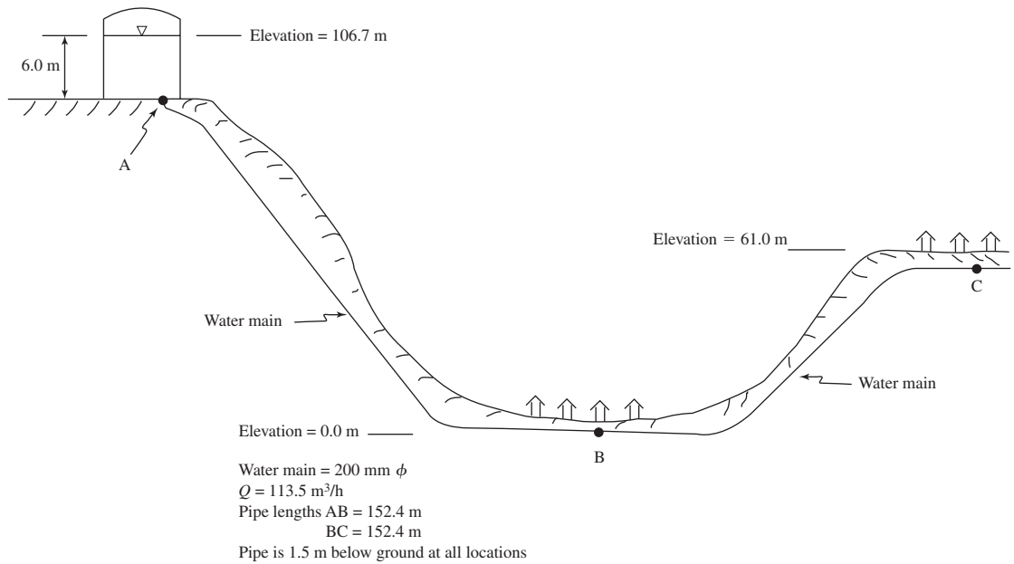
FIGURE P-17-11 Valley water distribution system.
