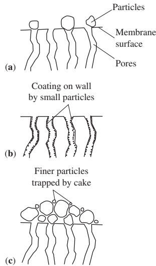
FIGURE 12-3 Mechanisms of membrane filtration: (a) Straining, (b) adsorption, (c) cake filtration.
