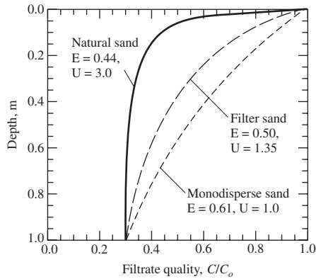
FIGURE 11-5 Effect of media uniformity on solids penetration in filter bed. (Source: MWH, 2005.)
