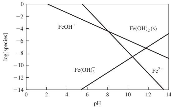
FIGURE 7-11 Solubility diagram for \text{Fe}(\text{OH})_2 .
