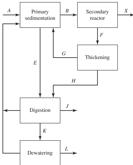
FIGURE P-27-9 Revised flowsheet for Doubtful WWTP.
