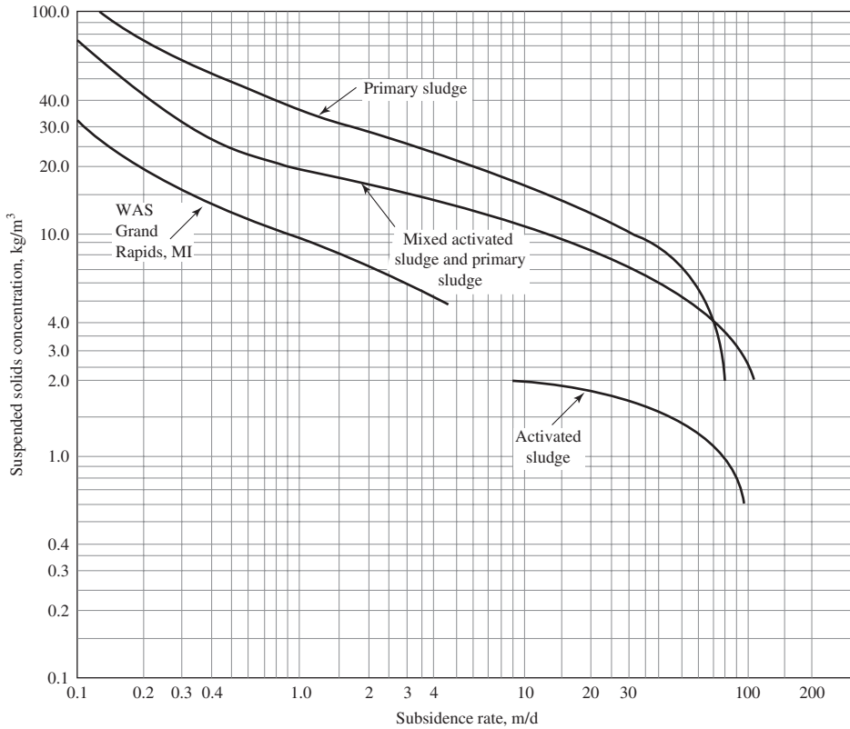
FIGURE 25-2 Batch settling curves. (Source: Davis and Cornwell, 2008.)
