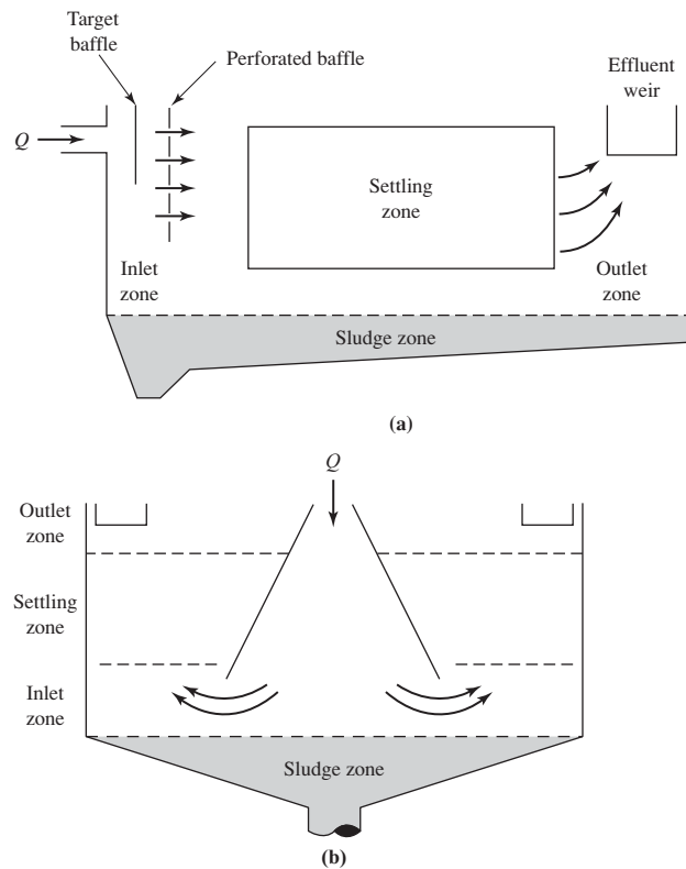
FIGURE 10-4 Zones of sedimentation: (a) horizontal flow clarifier; (b) upflow clarifier. (Source: Davis and Cornwell, 2008.)
