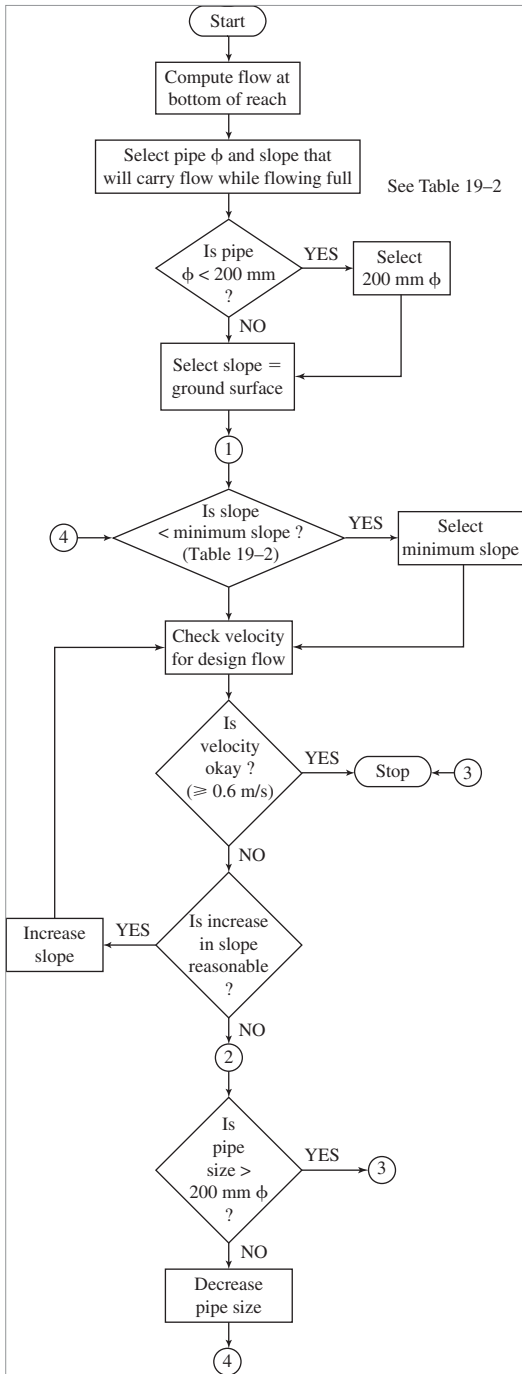
FIGURE 19-11 Sewer design flow chart for selecting pipe size for a reach between manholes.
