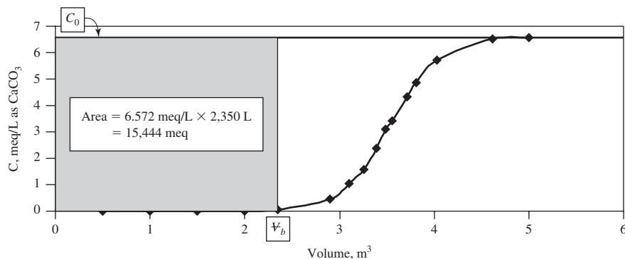
FIGURE 8-5 Ion exchange softening breakthrough curve.
