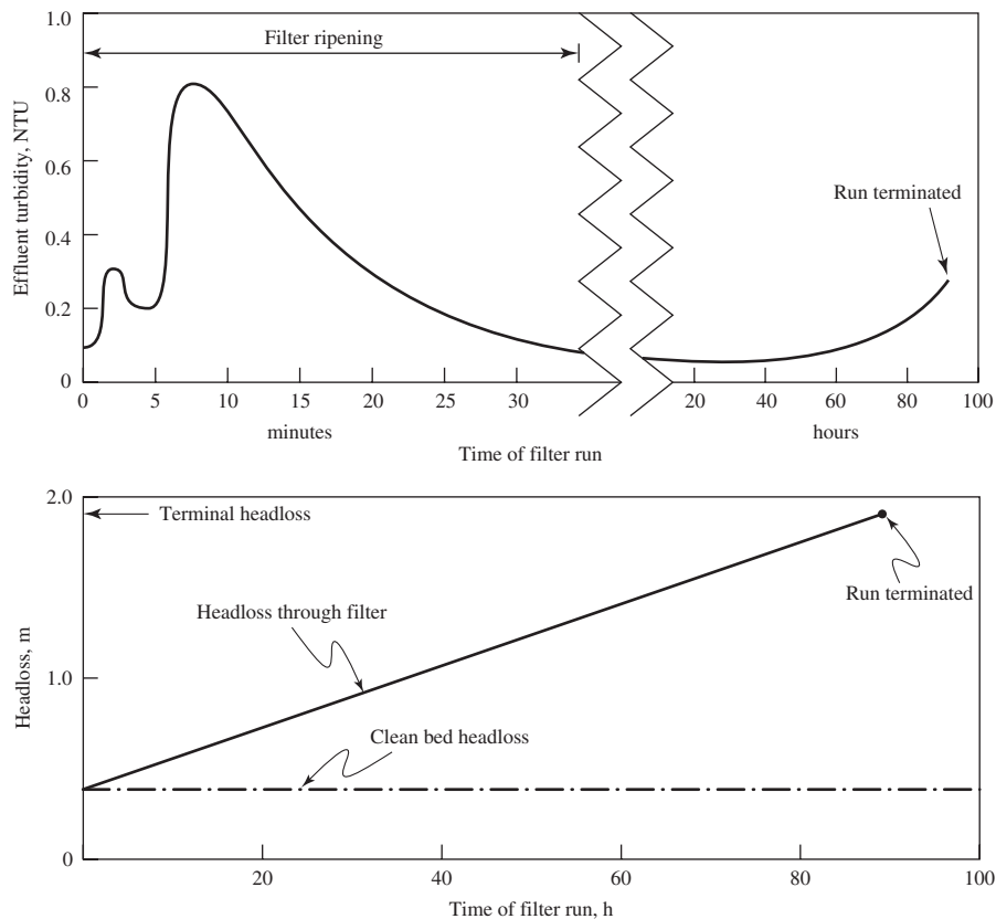
FIGURE 11-2 Idealized turbidity and headloss during a filter run. Note changes in time scale.
