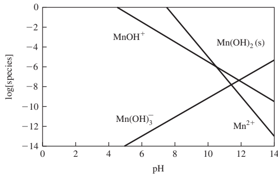
FIGURE 7-12 Solubility diagram for \text{Mn}(\text{OH})_2 .
