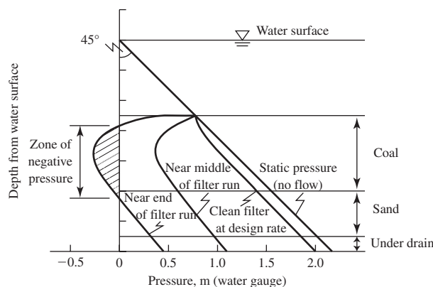
FIGURE 11-15 Pressure development within filter bed during filtration.
