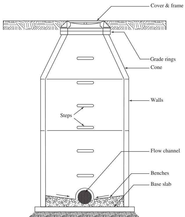
FIGURE 19-4 Manhole nomenclature.
