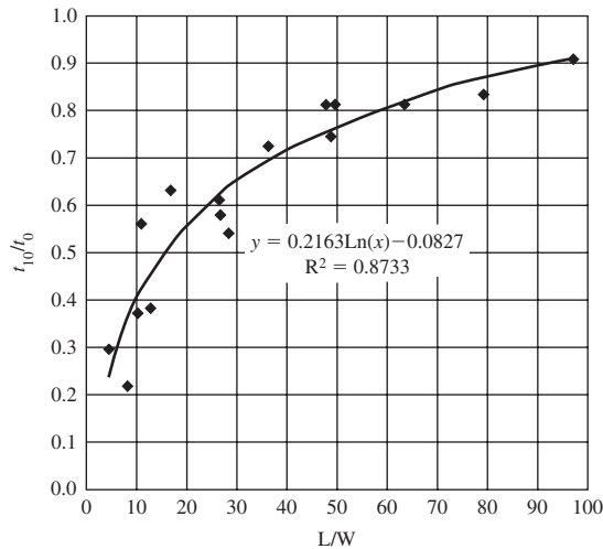
FIGURE 13-12 Impact of L/W on t_{10}/t_0 ratio.
