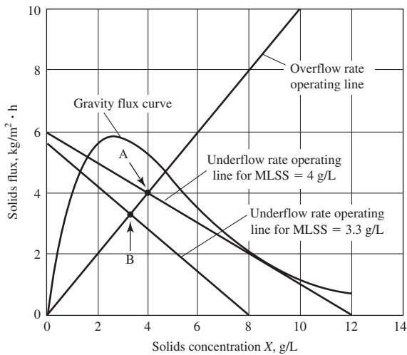
FIGURE 25-3 State point analysis illustrating critically loaded (A) and underloaded (B) state points relative to the gravity flux curve. (Source: Metcalf & Eddy, 2003.)
