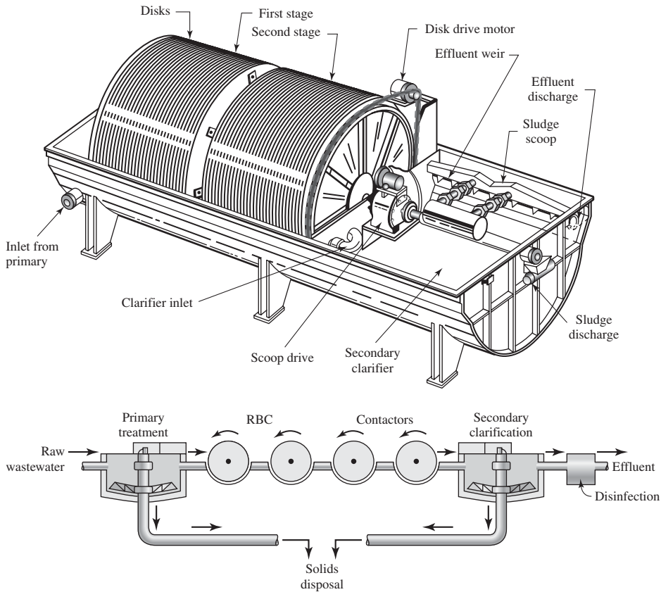
FIGURE 24-4 Rotating biological contactor (RBC) and process arrangement. (Source: U.S. EPA, 1977.)
