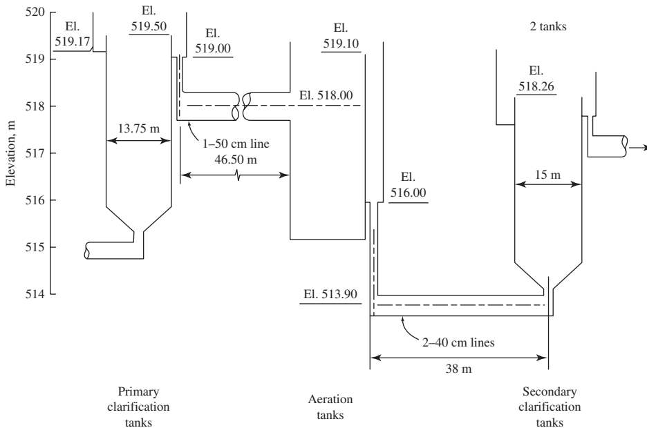
FIGURE P-28-5 Hydraulic profile for clean water plant.
