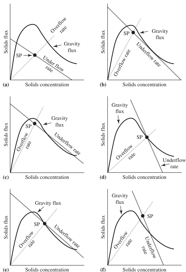
FIGURE 25-4 State point (SP) analysis for varying conditions to be interpreted with Table 25-1. SP = State Point.
