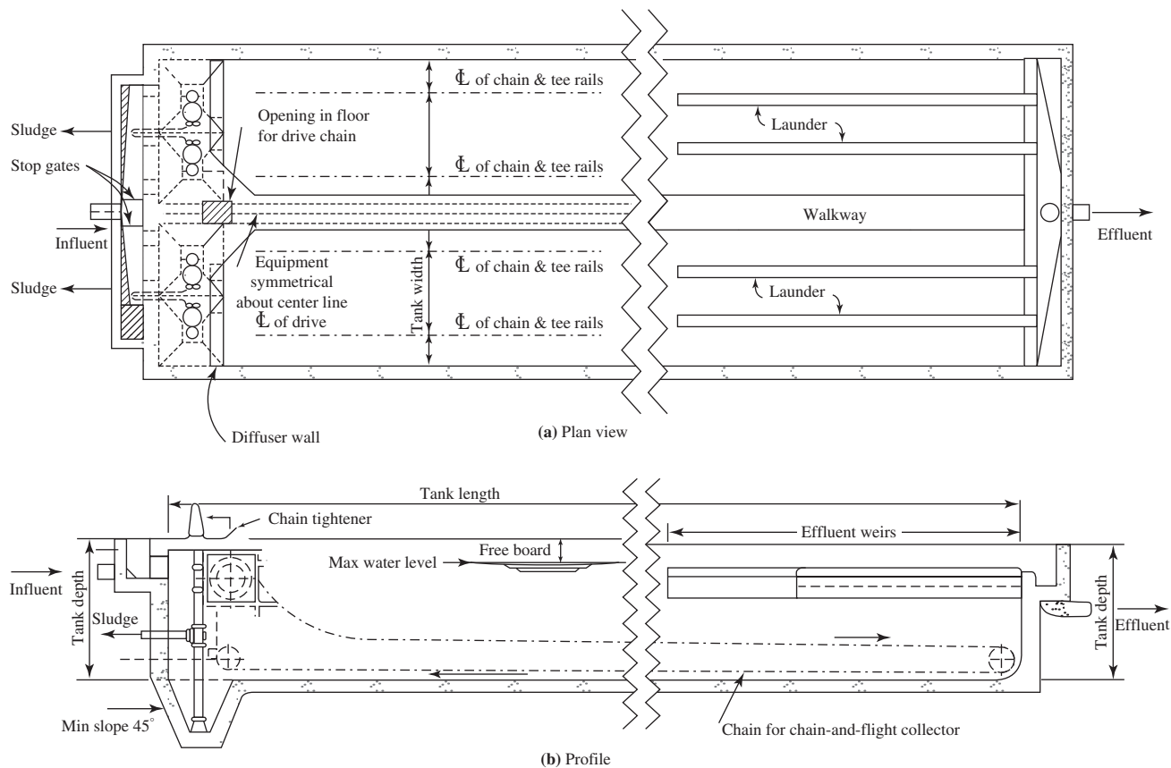
FIGURE 10-13 (a) Plan and (b) profile of horizontal-flow, rectangular sedimentation basin.
