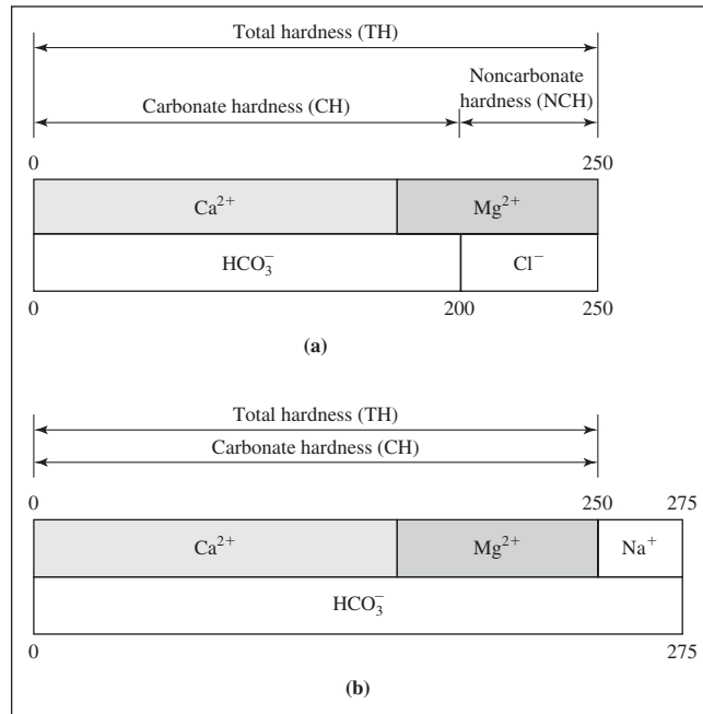
FIGURE 7-4 Relationships between total hardness, carbonate hardness, and noncarbonate hardness. (Source: Davis and Cornwell, 2008.)
