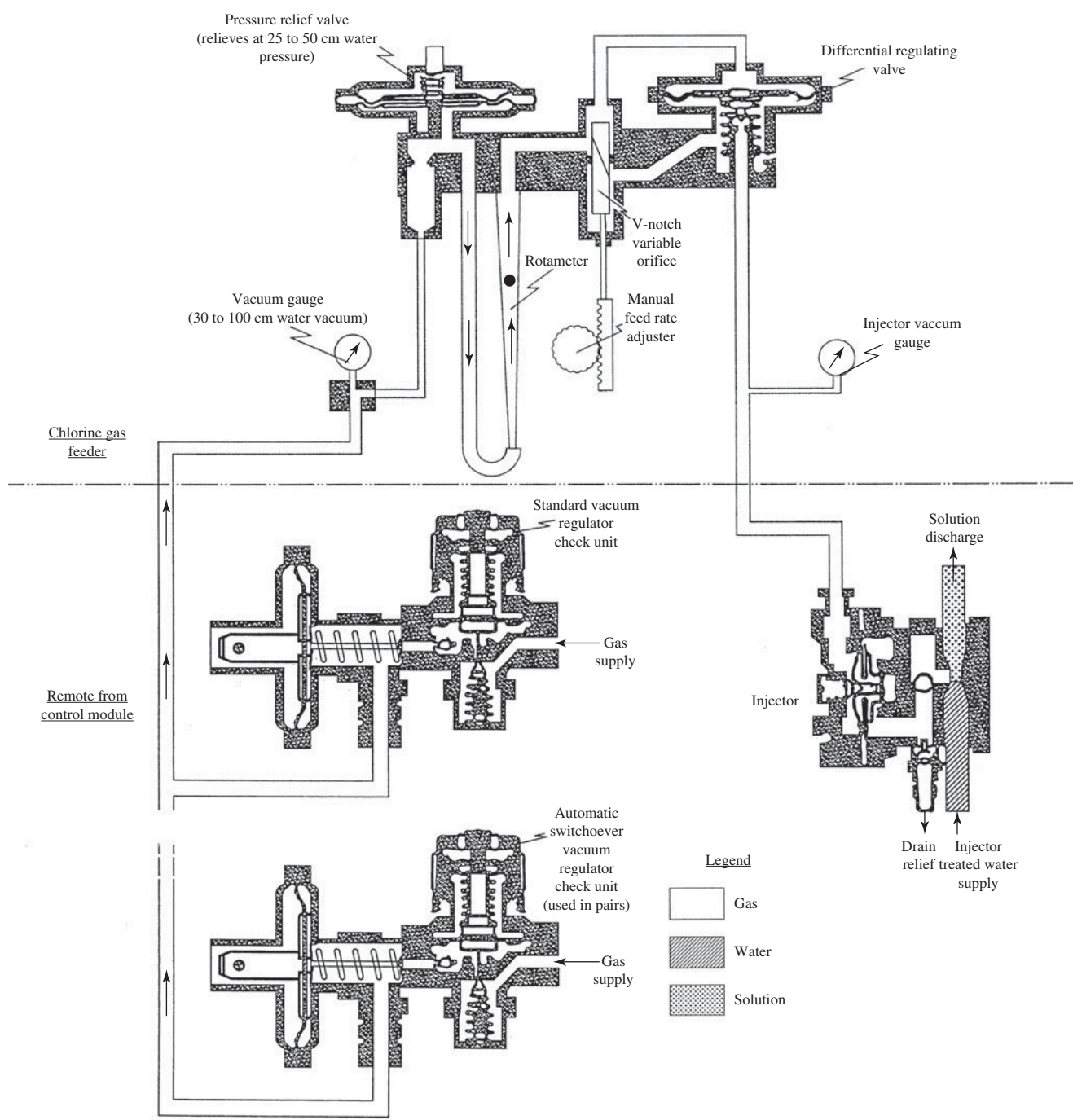
FIGURE 5-5 Flow diagram for conventional chlorinator.
