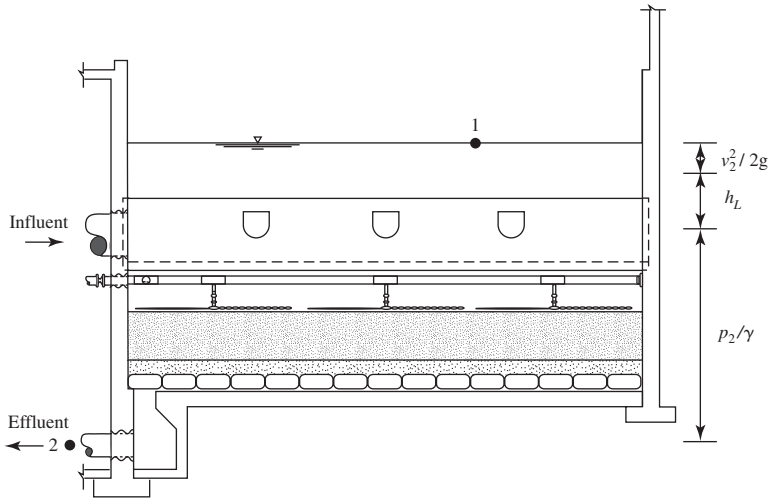
FIGURE 11-16 Schematic of granular filter during filtration. The Notation for Equation 11-22 is shown at right.
