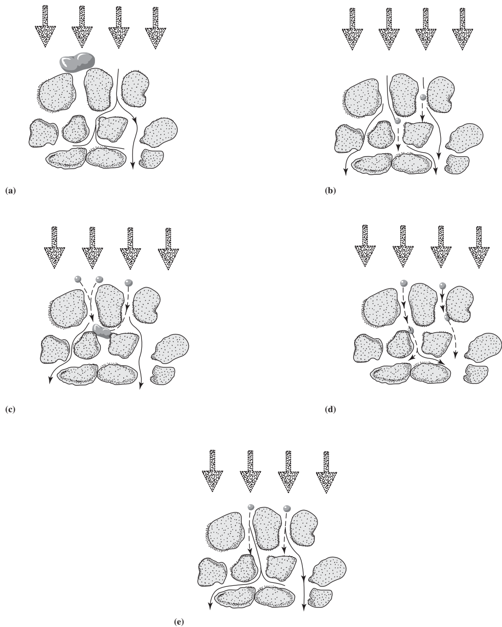
FIGURE 11-4 Mechanisms of granular filtration: (a) mechanical screening, (b) sedimentation, (c) flocculation, (d) interception, (e) impaction. Dashed line is particle trajectory. Solid line is water streamline (flow path).
