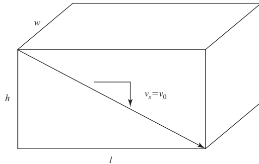
FIGURE 10-6 Dimensional definition of settling zone for Camp's derivation of overflow rate for a rectangular horizontal-flow sedimentation tank.
