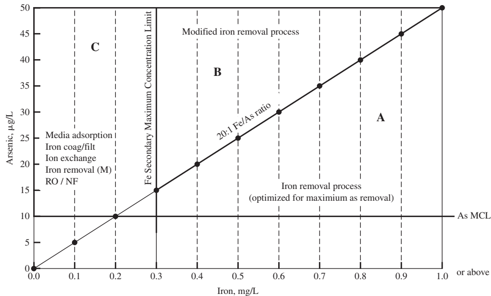
FIGURE 14-2 Arsenic treatment process selection guide. (Source: Cook, 2005.)
