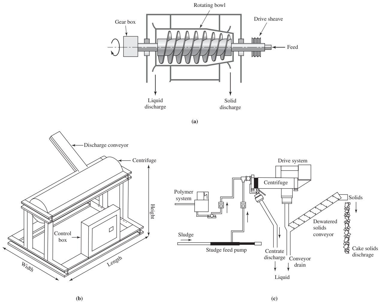
FIGURE 15-8 Solid bowl centrifuge. (a) Schematic, (b) isometric, (c) process layout. (Schematic Courtesy Bird Machine Company.)
