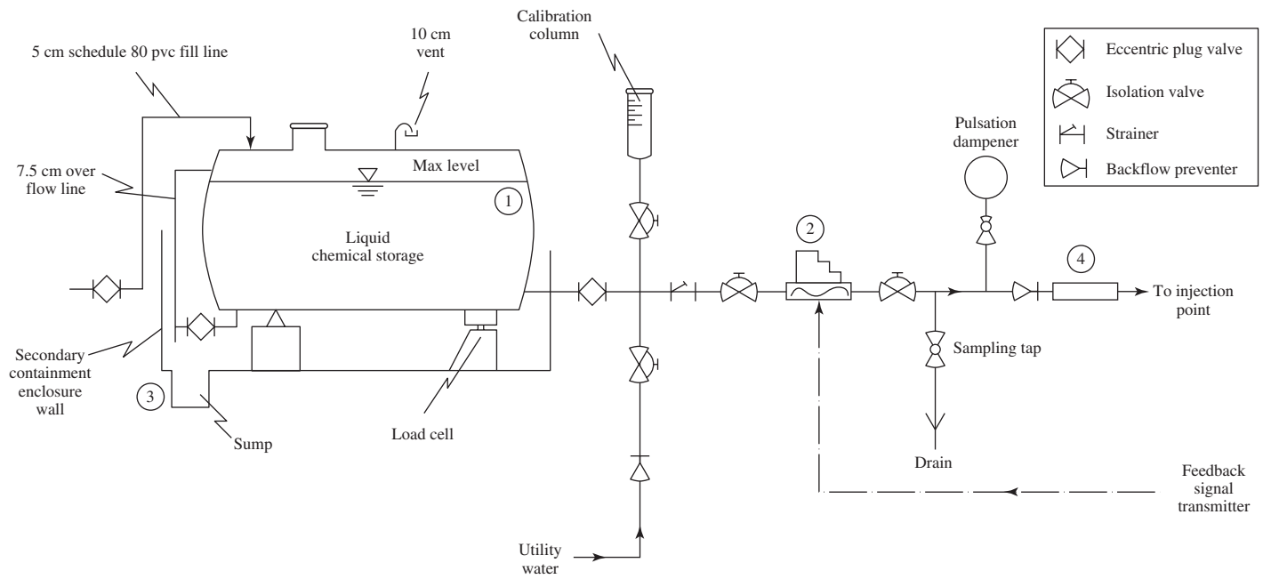
FIGURE 5-4 Liquid chemical feed system.
