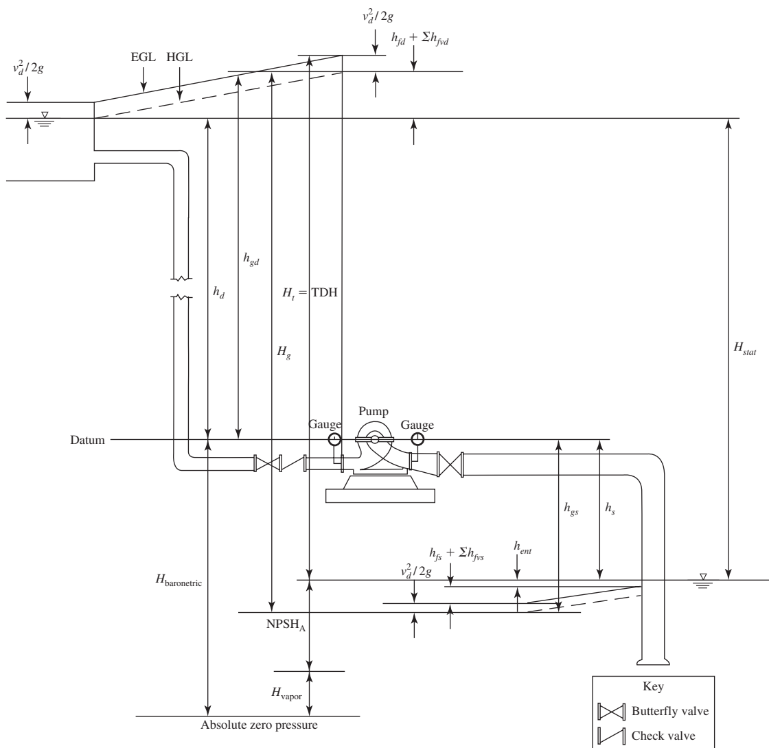
FIGURE 3-14 Terminology for a pump with a negative suction head.
