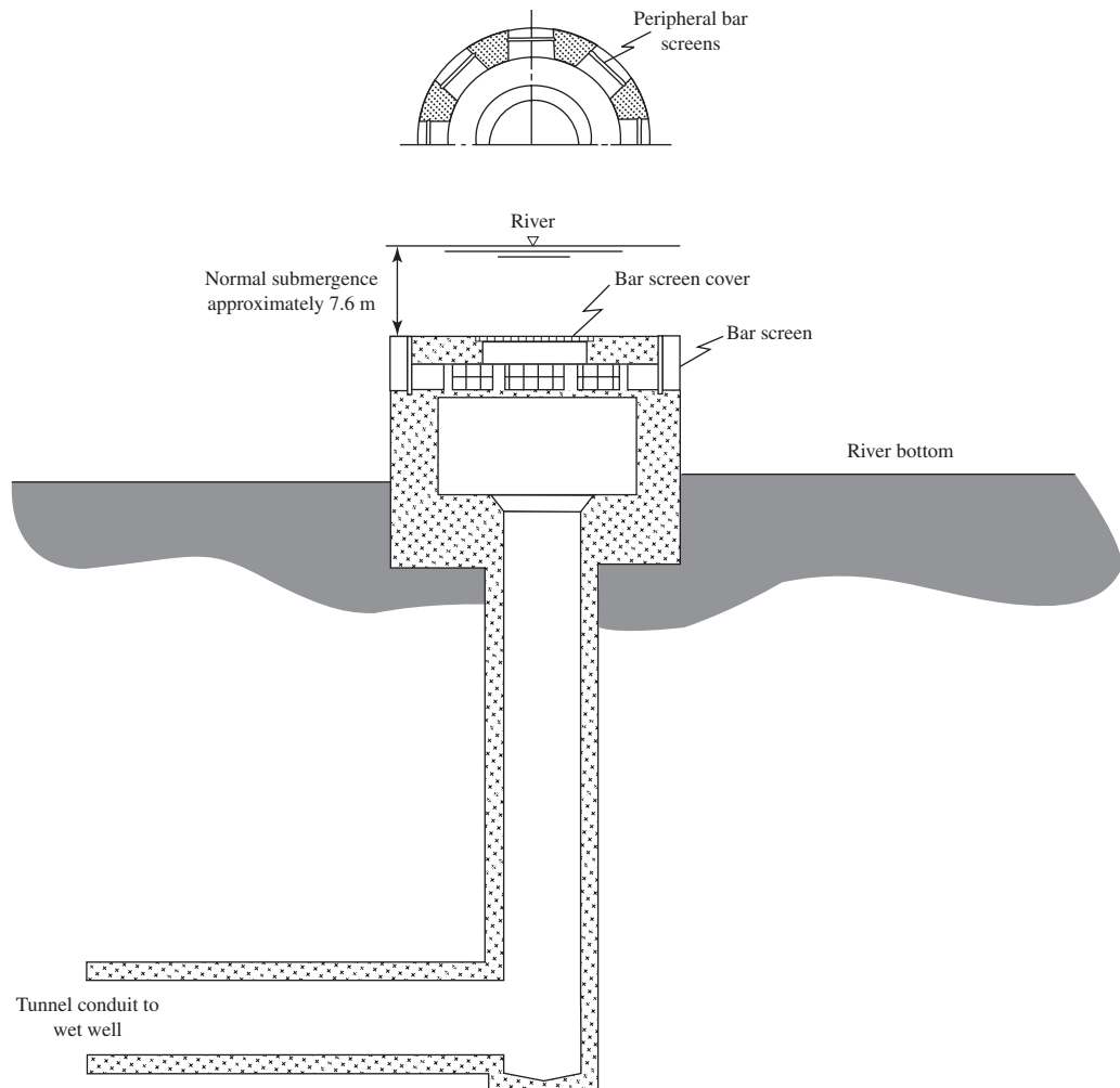
FIGURE 3-7 River intake.
