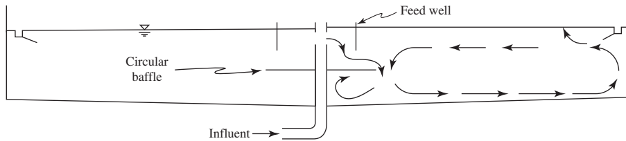
FIGURE 21-11 Circular baffle at inlet to reduce cascade effect.
