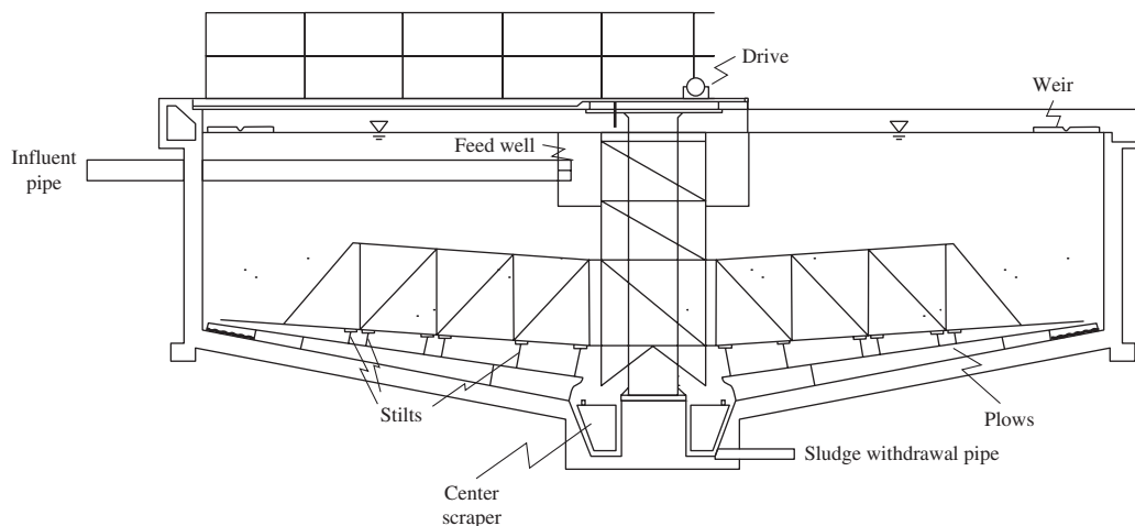
FIGURE 15-2 Continuous-flow gravity thickener.
