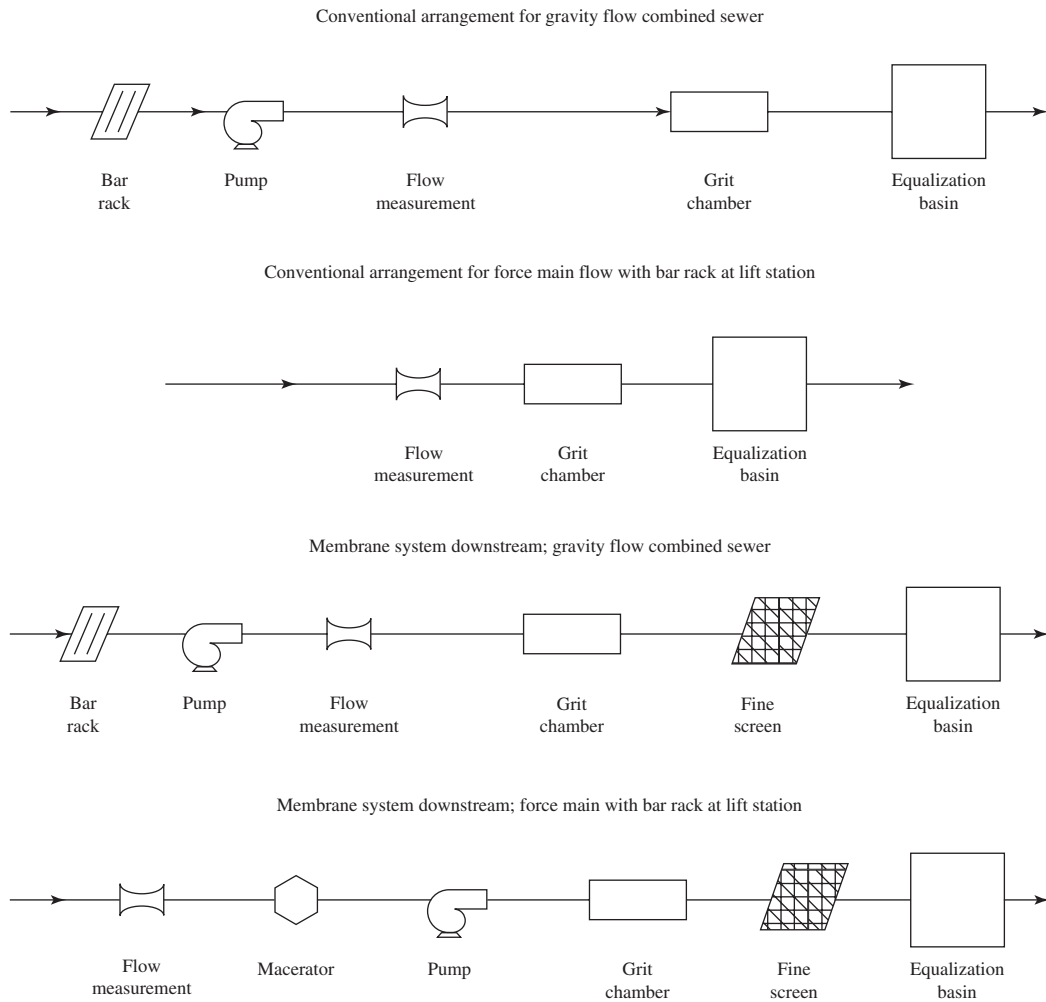
FIGURE 20-19 Examples of some alternative arrangements of preliminary treatment processes.
