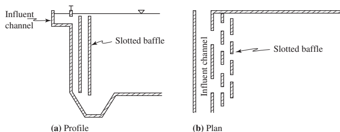
FIGURE 21-15 Slotted baffles in a rectangular primary tank.
