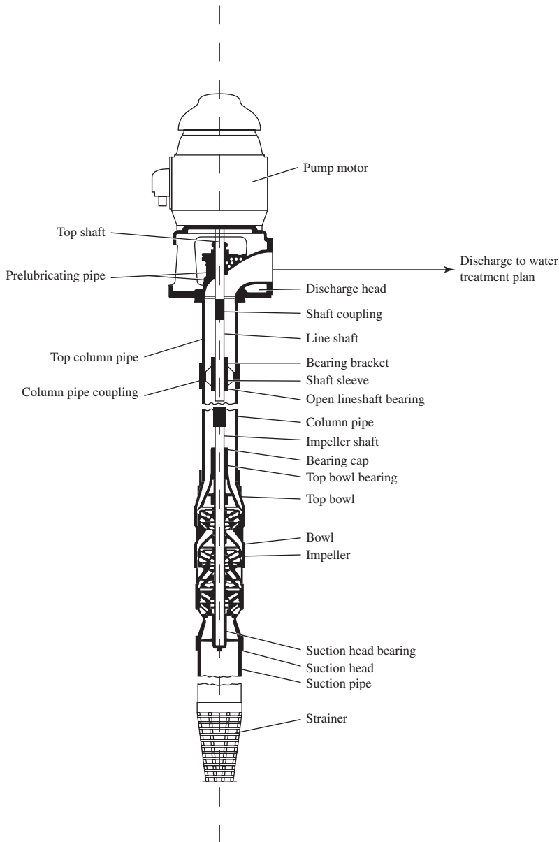
FIGURE 3-11 Section of vertical turbine pump with closed impellers and open-line shafting (water lubrication).
