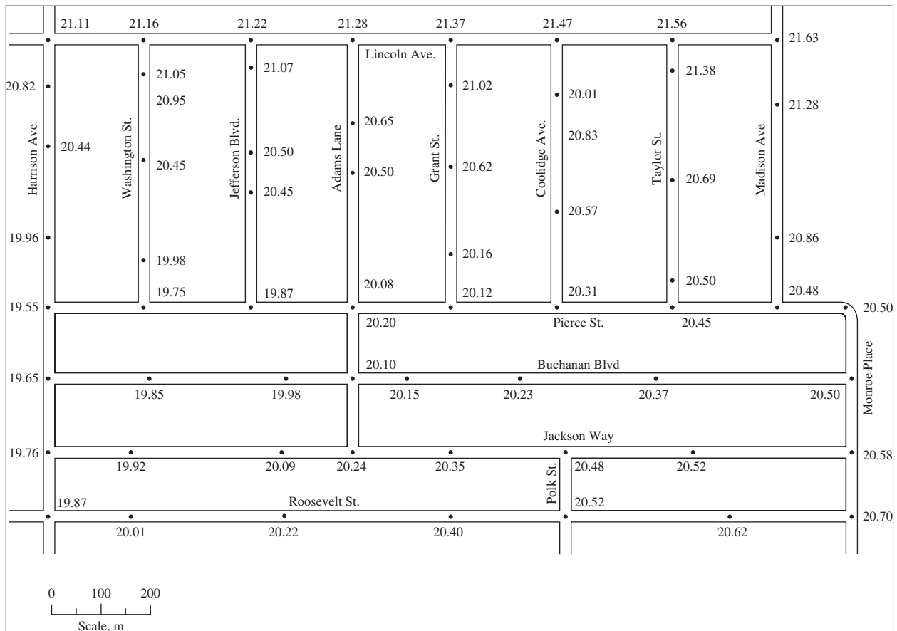
FIGURE P-19-14 Map for Problem 19-14. Surface elevations are in meters at points noted by dots. Intermediate manholes between street intersections are not shown. These must be added. Interpolate between elevations shown for additional elevations. (Source: Metcalf & Eddy, 1981.)
