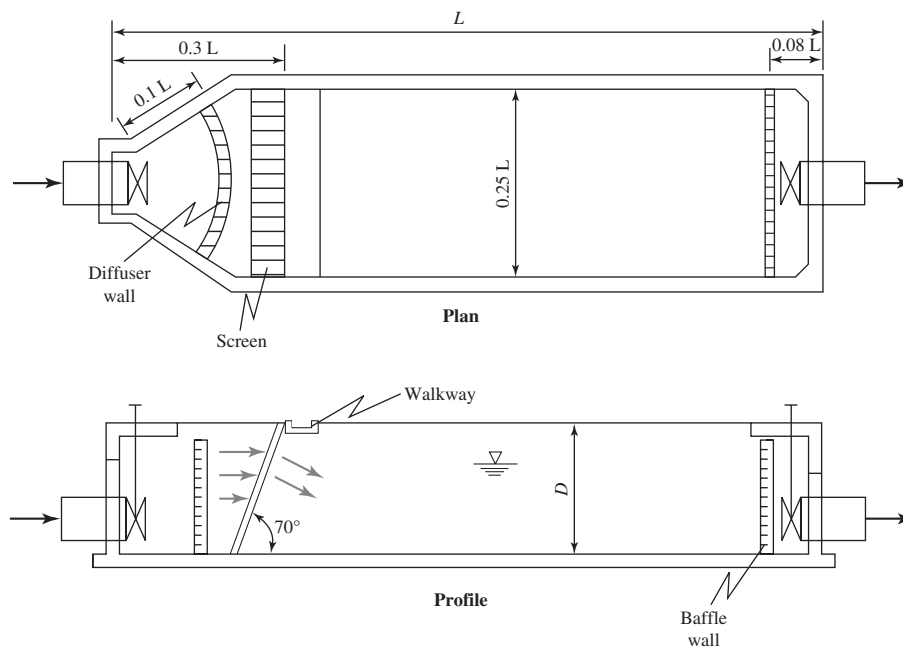
FIGURE 3-19 Grit chamber.
