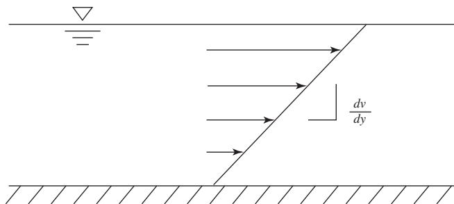
FIGURE 6-12 Velocity gradient.
