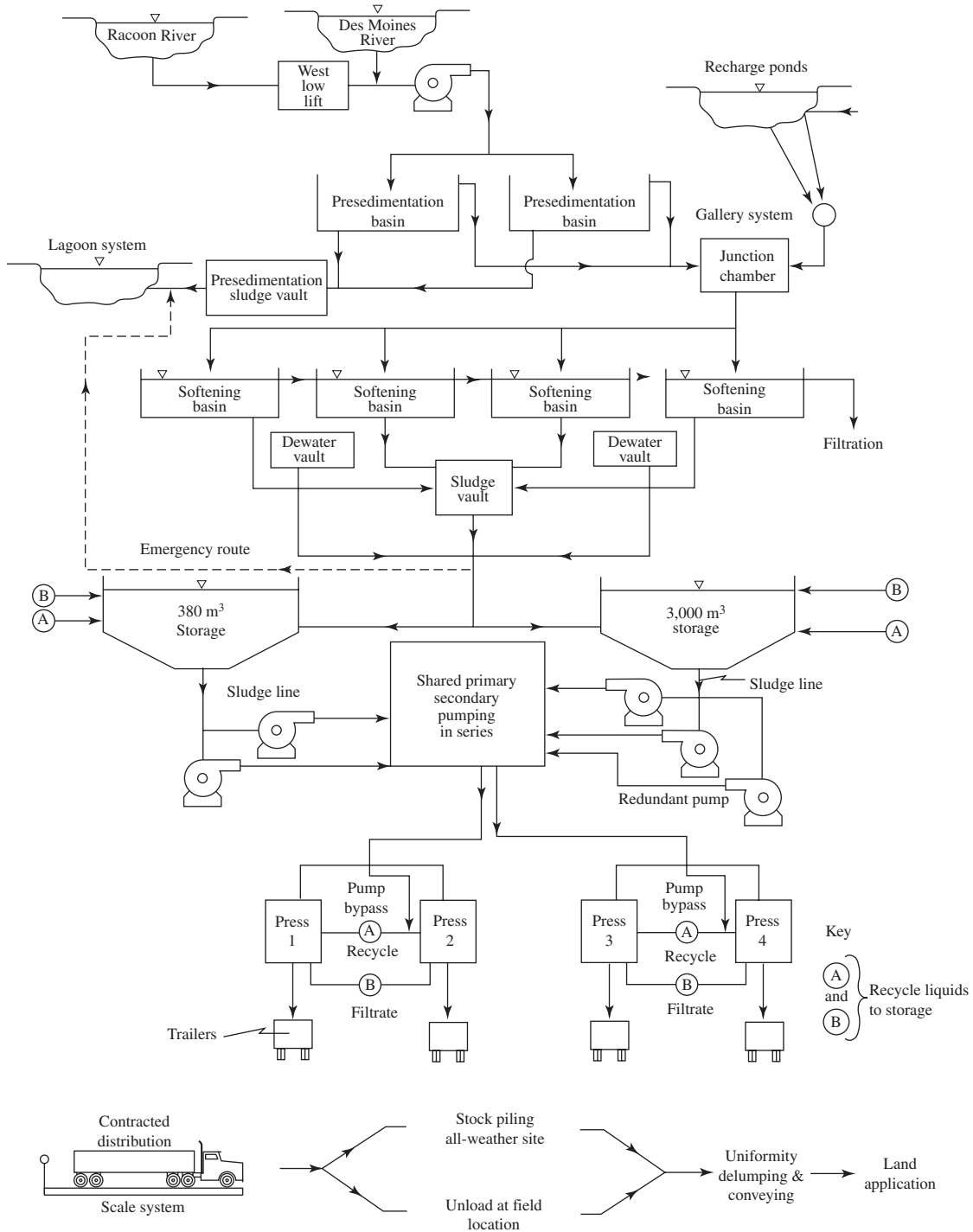
FIGURE P-16-13 Des Moines WTP residuals handling. Supernatant from storage is recycled to head end of plant.
