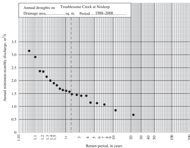
FIGURE 2-4 Annual droughts on Troublesome Creek at Nosleep.
