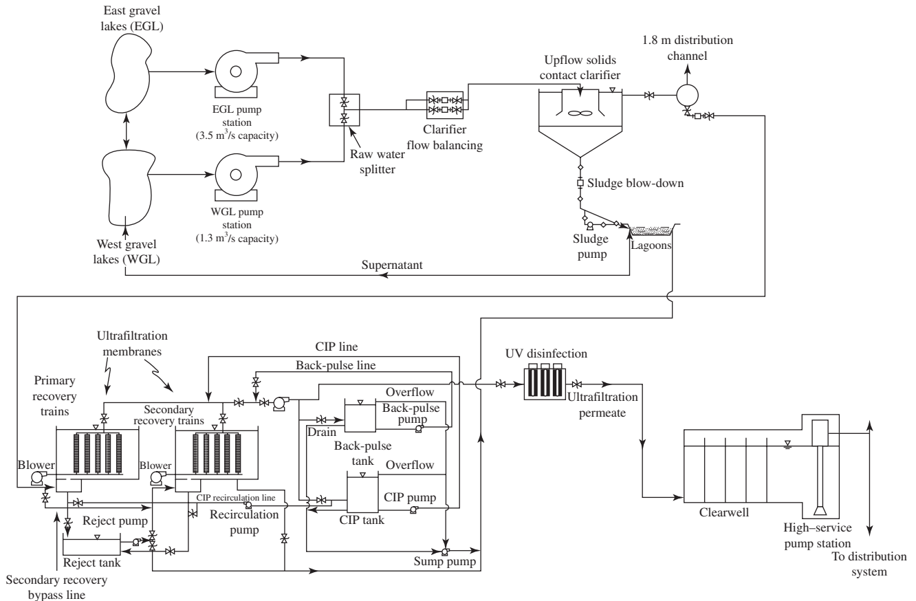
FIGURE P-16-11 Thornton's WTP.
