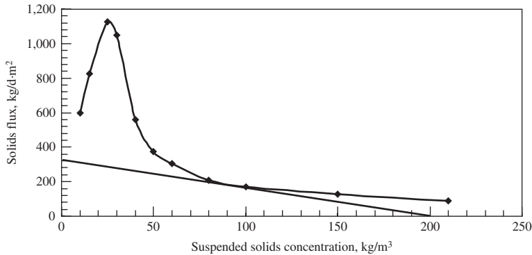
FIGURE 15-5 Batch flux curve.
