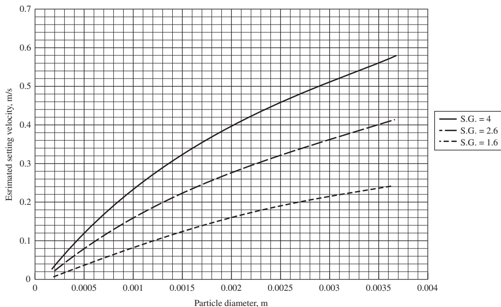
FIGURE 11-7 Particle settling velocity estimation chart. S. G. = specific gravity.
