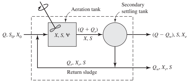
FIGURE 23-9 Completely mixed biological reactor with solids recycle. (Source: Davis and Cornwell, 2008.)
