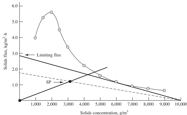
FIGURE 25-5 Gravity flux curve for Example 25-1.
