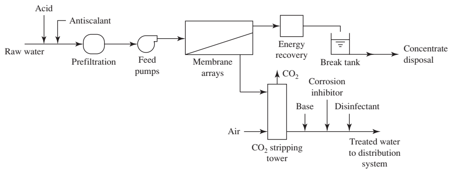
FIGURE 9-8 Schematic of typical reverse osmosis facility.
