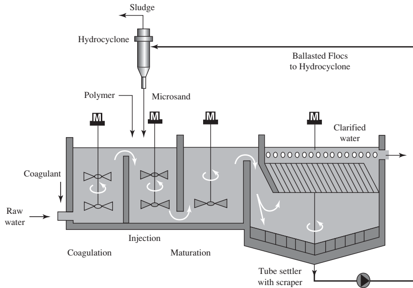
FIGURE 10-16 ACTIVFLO ballasted sedimentation process for water treatment. (Courtesy of Kruger Inc.)
