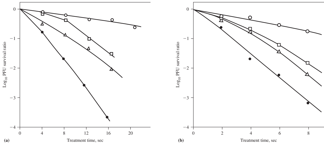
FIGURE 13-4 Inactivation of single poliovirus particles by HOCl (a) at 10°C, pH 6.0: (○) 1.5 μM, (□) 11 μM, (△) 20 μM, and (●) 41 μM; (b) at 20°C, pH 6.0: (○) 2.2 μM, (□) 11 μM, (△) 22 μM, and (●) 35 μM. (Source: Floyd, et al., 1979.)
