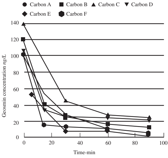
FIGURE 14-10 Kinetic test results for adsorption of MIB for various PACs. (Source: Huang et al., 1996).
