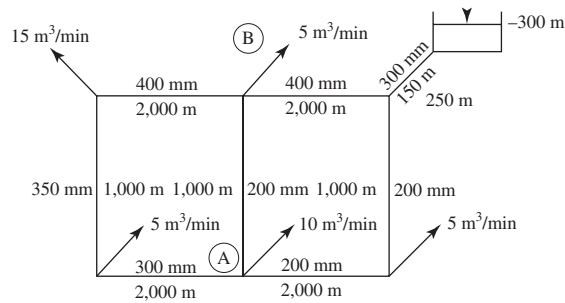
FIGURE P-17-26 Distribution network analysis with elevated storage. Adapted from Steel and McGhee, 1979.
