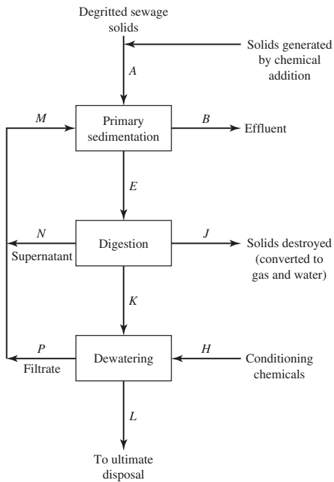
FIGURE 27-3 Primary WWTP flowsheet. (Source: U.S. EPA, 1979.)
