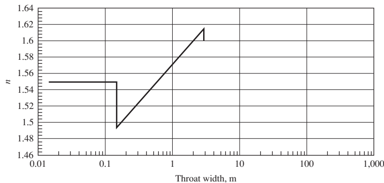
FIGURE 20-3A Parshall flume coefficient n .
