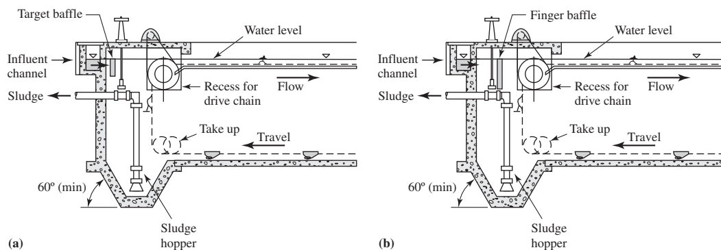
FIGURE 21-14 Examples of (a) target and (b) finger baffles.
