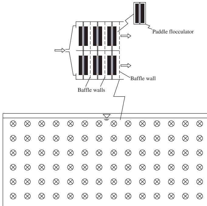
FIGURE 6-19 Baffle wall arrangement for three compartment flocculator. Note that there are two parallel treatment trains and that each baffle wall will have a different orifice arrangement.
