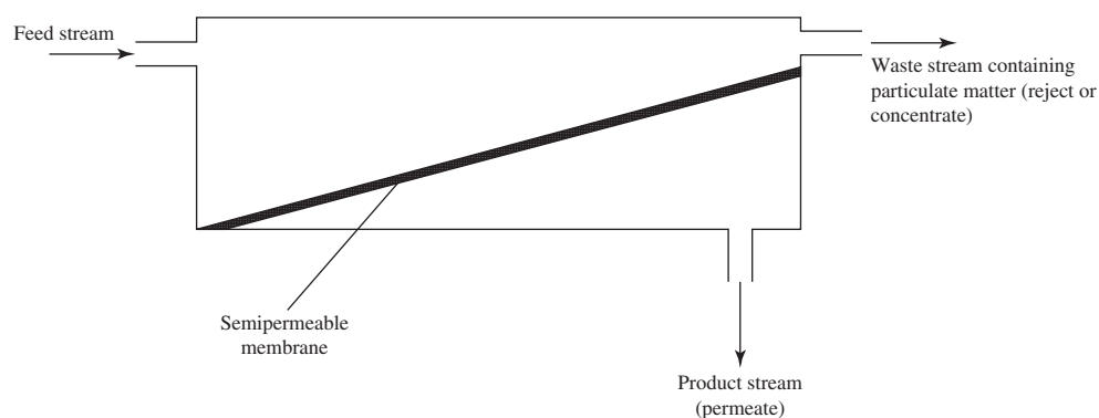
FIGURE 12-1 Schematic of separation process through semipermeable membrane.
