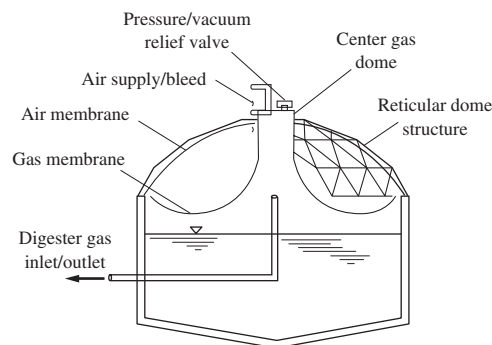
FIGURE 27-18 Anaerobic digester with membrane gas cover. (Source: Metcalf & Eddy, 2003.)
