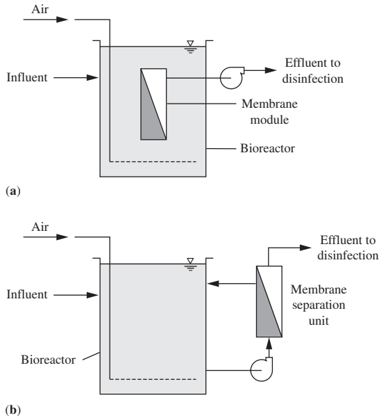
FIGURE 23-6 Schematic diagram of membrane bioreactors: (a) immersed membrane, (b) external membrane. (Source: Metcalf & Eddy, 2003.)
