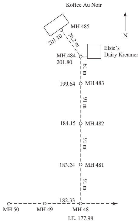
FIGURE 19-12 Plan view of sewer for Example 19-2. MH = manhole. Elevations on the left of the MH are surface elevations.
