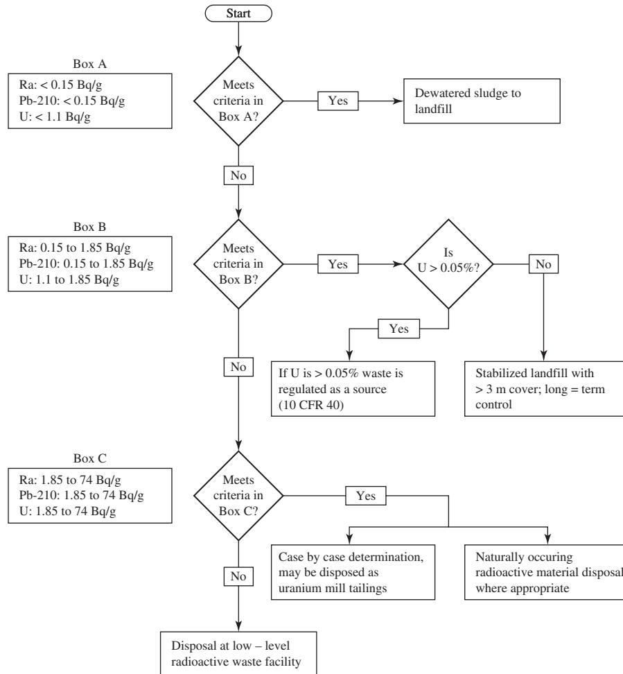
FIGURE 15-16 U.S. EPA suggested disposal alternatives for water treatment plant solid wastes containing natural radioactivity.
