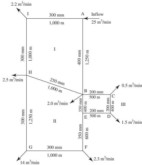
FIGURE P-17-25 Distribution network analysis with fire. Adapted from Steel and McGhee, 1979.
