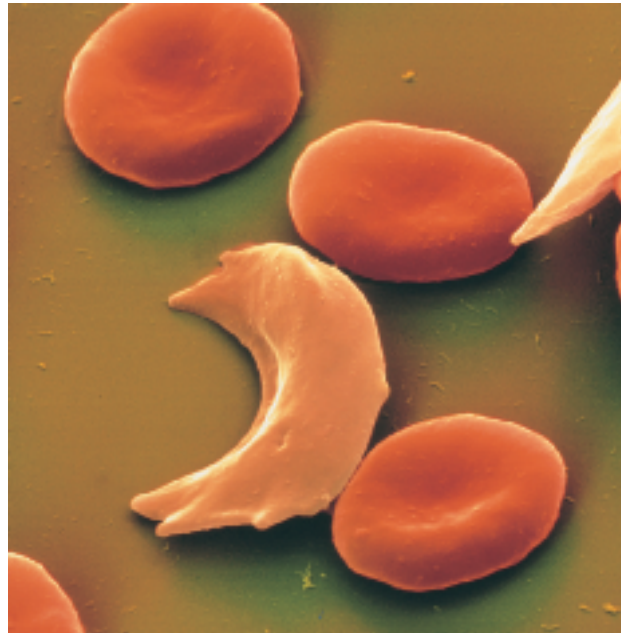
Figure 6-10 An electron micrograph of a sickle-shaped red blood cell. Other, more rounded cells appear almost normal. [Meckes/Ottawa/Photo Researchers.]
