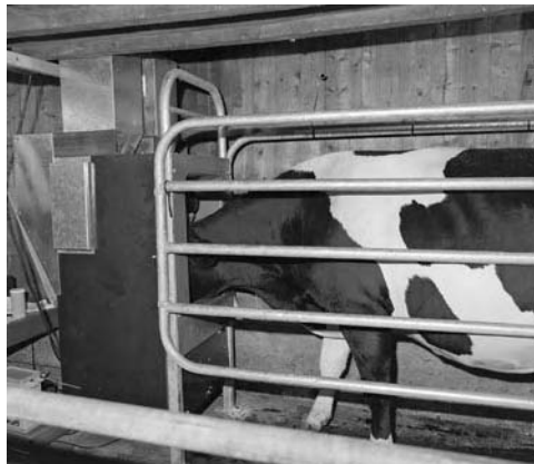
Fig. 25.2. A transponder-controlled feeding stall was modified to allow individual cow breath samples to be taken before feed was dispensed to the cow. Photo: Silsoe Research Institute.
