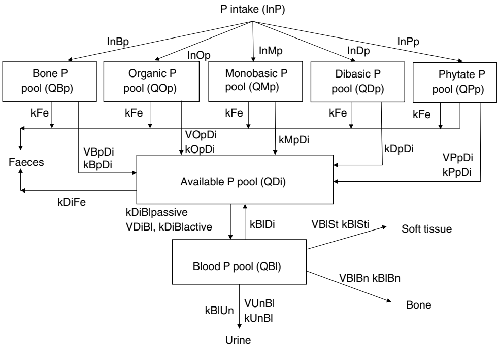
Fig. 18.1. Diagram of dynamic model of P utilization in salmonid fish. Boxes indicate pools and arrows indicate fluxes.
