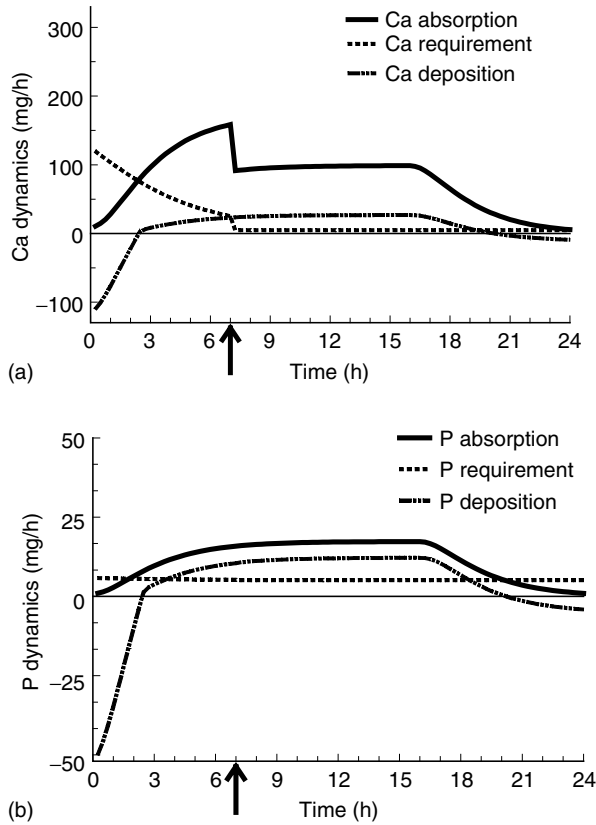
Fig. 19.5. Simulated diurnal dynamics of (a) calcium (Ca) and (b) phosphorus (P) in a layer at oviposition 7 h after light is switched on. The arrow denotes time of oviposition. Ca absorption is absorption from the duodenum, Ca requirement is requirement for maintenance and egg production (shell, yolk and white), and Ca deposition is bone synthesis (positive values) or bone mobilization (negative values).
