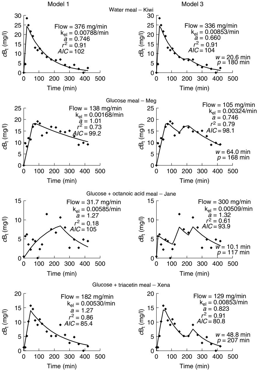
Fig. 8.5. Fits of models 1 and 3 (solid lines), assuming continuous and intermittent zero-order gastric emptying, respectively, to four selected plasma acetaminophen appearance curves ( \blacklozenge ).
