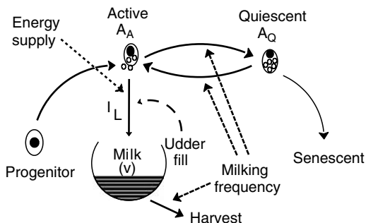
Fig. 34.2. Representation of the lactation submodel. Solid lines represent fluxes between pools and dashed lines represent influences of milking frequency (MF), energy availability and udder fill on these fluxes.
