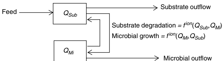
Fig. 26.1. Comparison of static and dynamic representations of substrate degradation and microbial growth (arrows indicate flows, boxes indicate state variables in a dynamic system).
