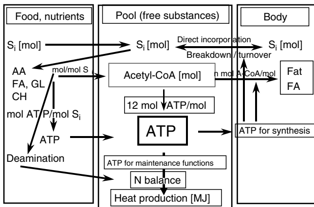
Fig. 31.4. Model of intermediary metabolism according to the adenosine triphosphate (ATP) concept. S = substrate, AA = amino acids, FA = fatty acids, GL = glycerine, CH = carbohydrates.
