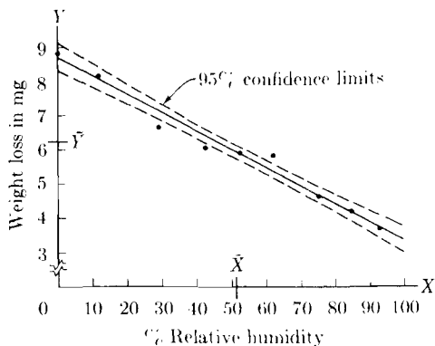
FIGURE 11.11 95% confidence limits to regression estimates for data of Figure 11.6.
