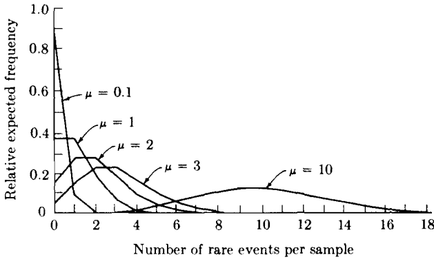
FIGURE 4.3 Frequency polygons of the Poisson distribution for various values of the mean.
