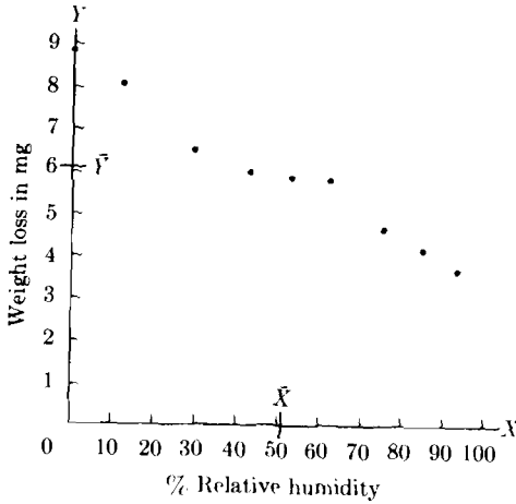
FIGURE 11.3 Weight loss (in mg) of nine batches of 25 Tribolium beetles after six days of starvation at nine different relative humidities. Data from Table 11.1, after Nelson (1964).
