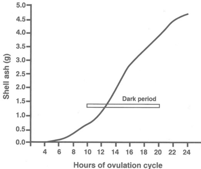
Fig. 5.6 Shell mineral deposition over a 24h ovulation cycle.
