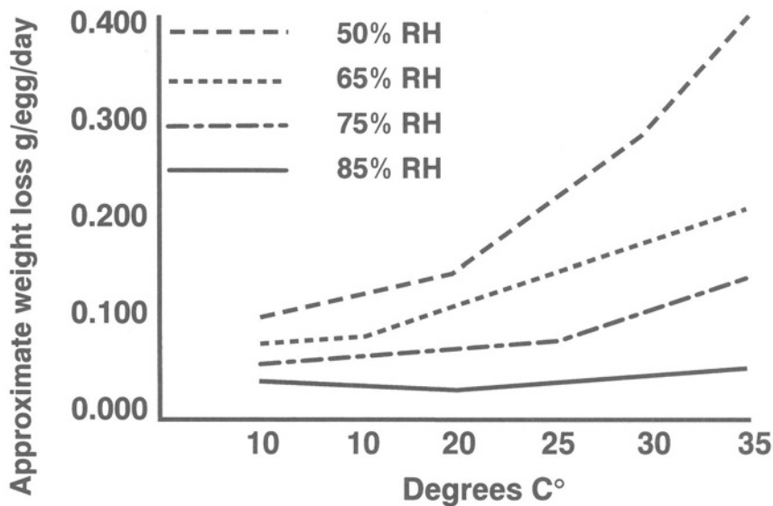
Fig. 8.20 Effects of temperature and humidity on egg weight loss.
