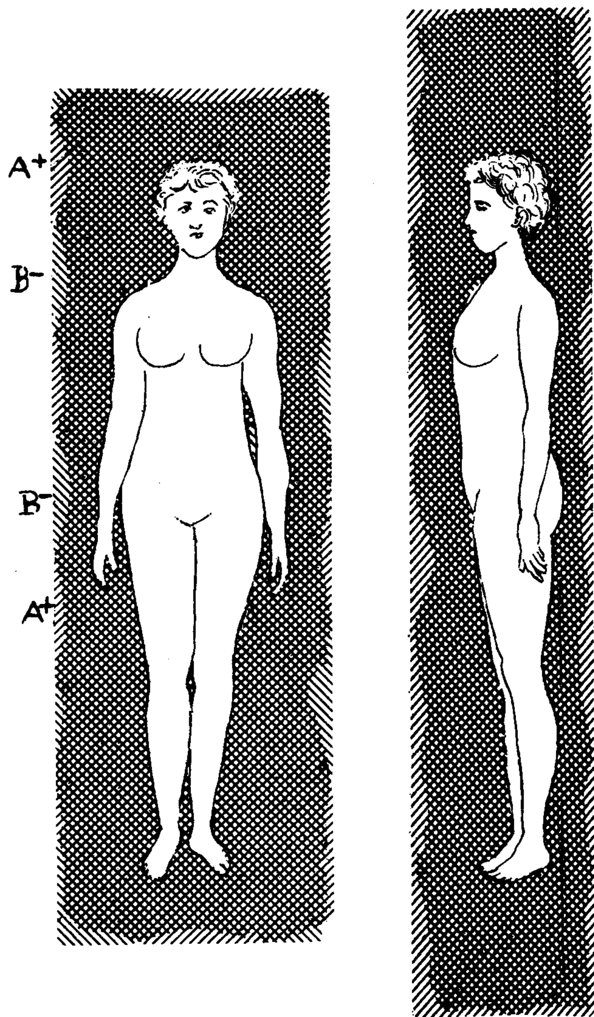
The Lines Of Force And People
