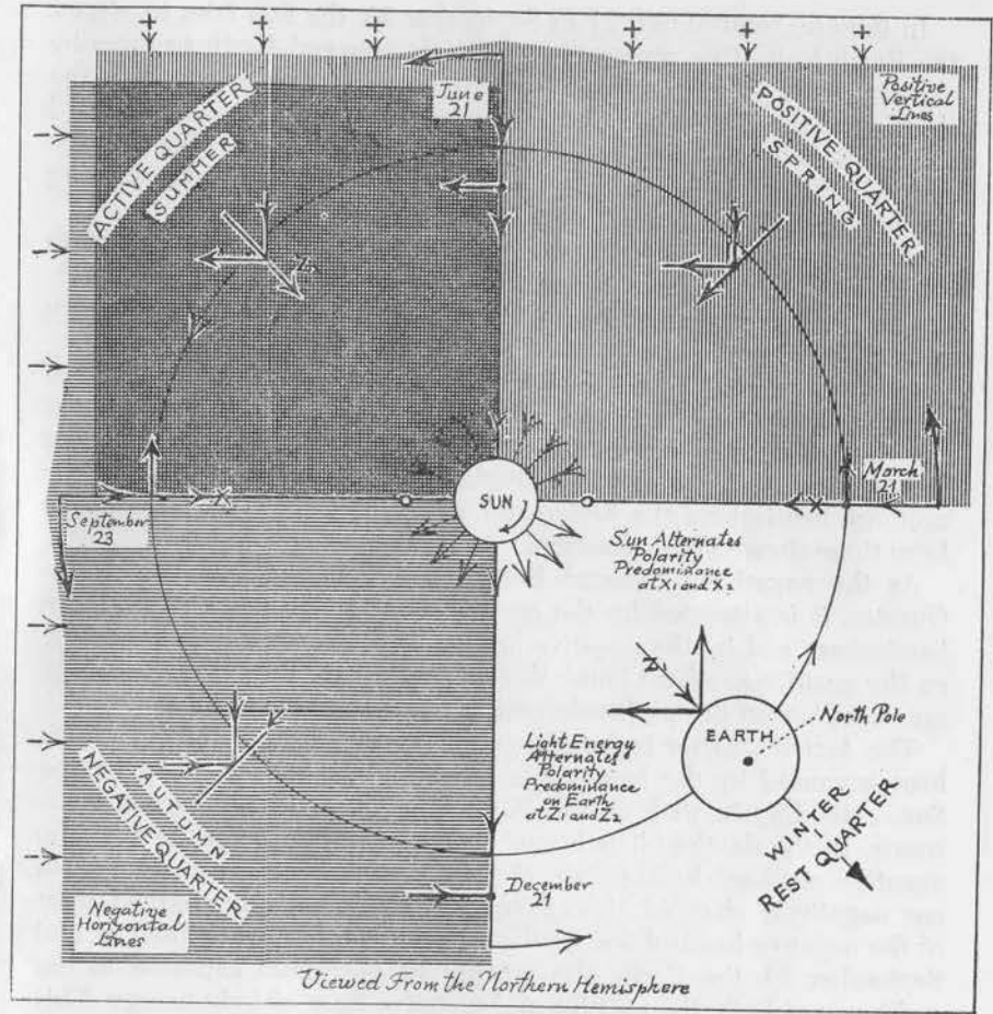
Orbit Principle Of The Earth
