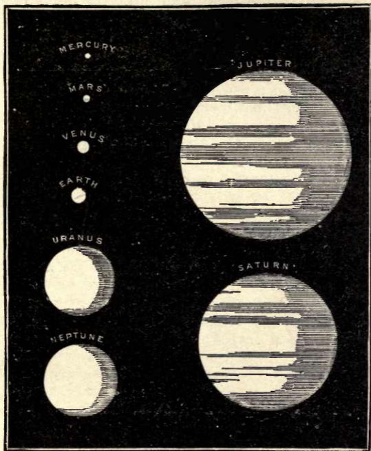
FIG. 3.—Comparative Sizes of the Major Planets.
