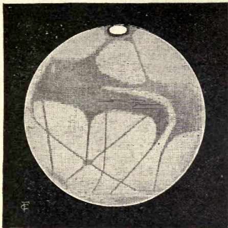
FIG. 13.—Mars, August 27, 1892 (Guiot).
