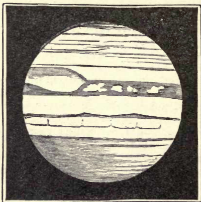
FIG. 14.—Jupiter, November 27, 1857 (Dawes).
