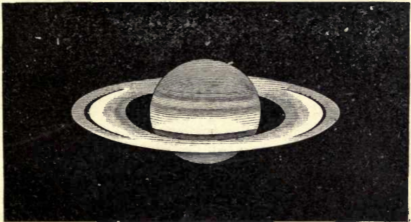
FIG. 15.—Saturn, Jan. 26, 1889 (Antoniadi).
