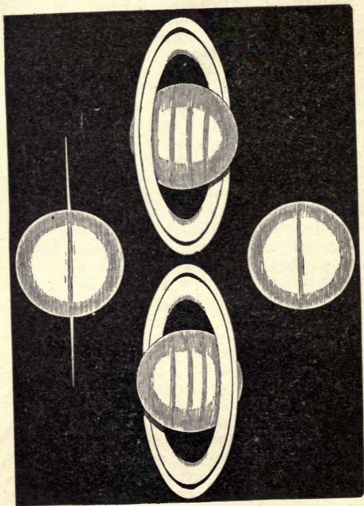
FIG. 16.—General view of the Phases of Saturn's Rings.
