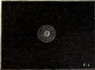
FIG. 22.—Holmes's Comet, Nov. 9, 1892 (Denning).
