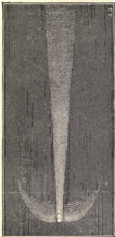
FIG. 25.—Sawerthal's Comet, June 4, 1888 (Charlois).
