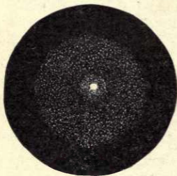
FIG. 19.—Telescope Comet with a nucleus.
