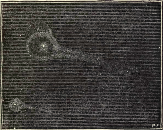
FIG. 26.—Biela's Comet, February 19, 1846.
