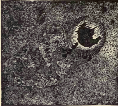
FIG. 5.—Ordinary Sun-spot, June 22, 1885.
