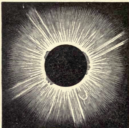
FIG. 8.—The Sun totally eclipsed, July 18, 1860 (Feilitzsch).
