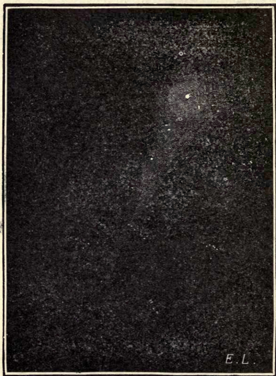
FIG. 21.—Quenisset's Comet, July 9, 1893 (Quenisset).
