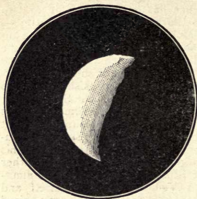
FIG. 9.—Venus, Dec. 23, 1885.
