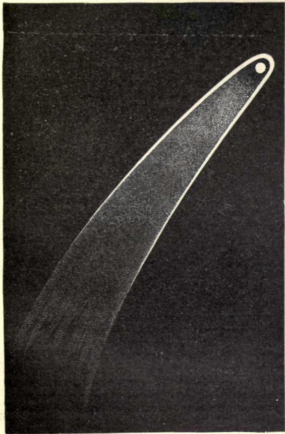
FIG. 27.—The Great Comet of 1811.
