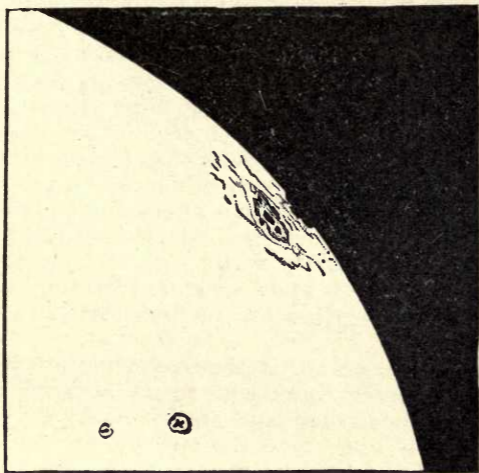
FIG. 7.—Sun-spot seen as a Notch.
