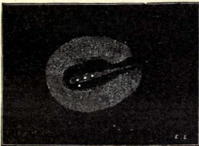
FIG. 23.—Holmes's Comet, Nov. 16, 1892 (Denning).
