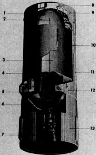
SATURN IB
